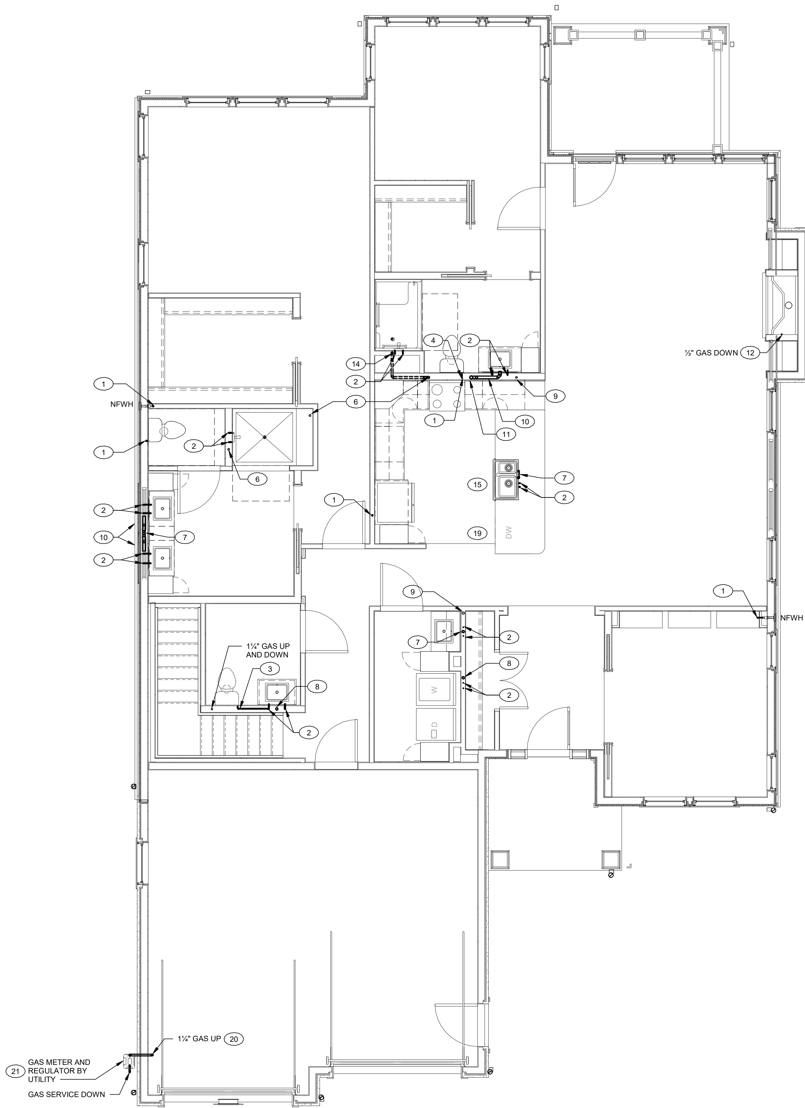
1 UNIT N - SIWANOY II - FLOOR PLAN - PLUMBING 1/4" = 1'-0"
