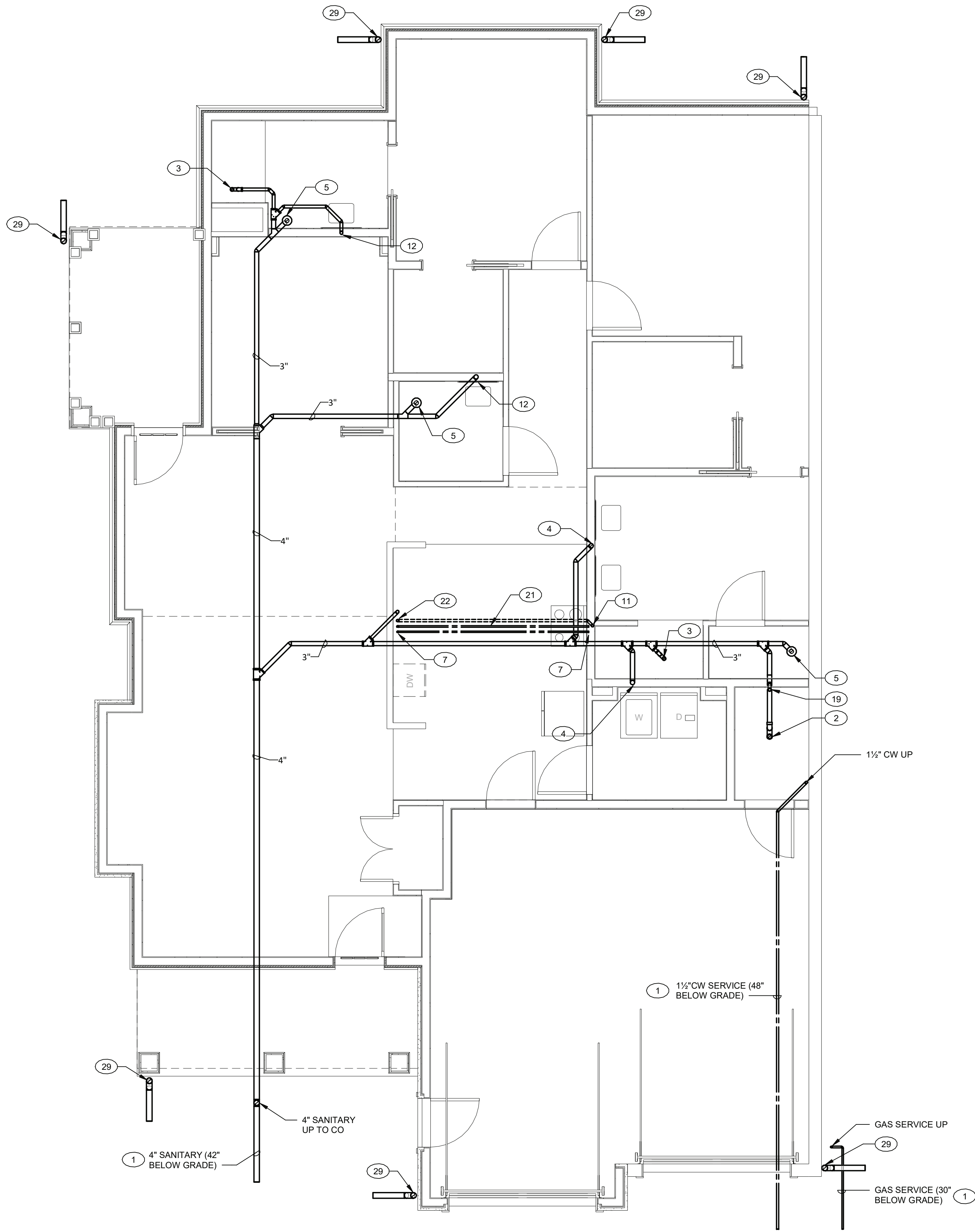
2 UNIT M - SHENOROCK I - BELOW FLOOR PLAN - PLUMBING 1/4" = 1'-0"
