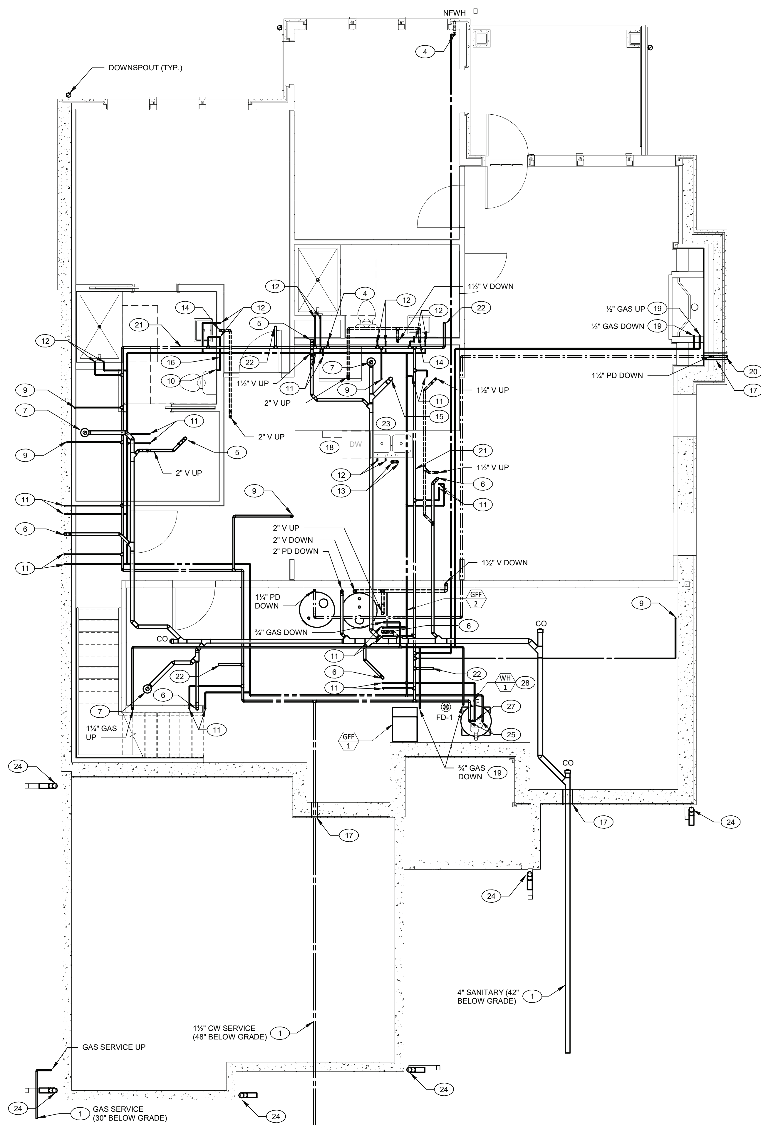
2 UNIT N - SIWANOY II - ABOVE BASEMENT FLOOR PLAN - PLUMBING 1/4" = 1'-0"
