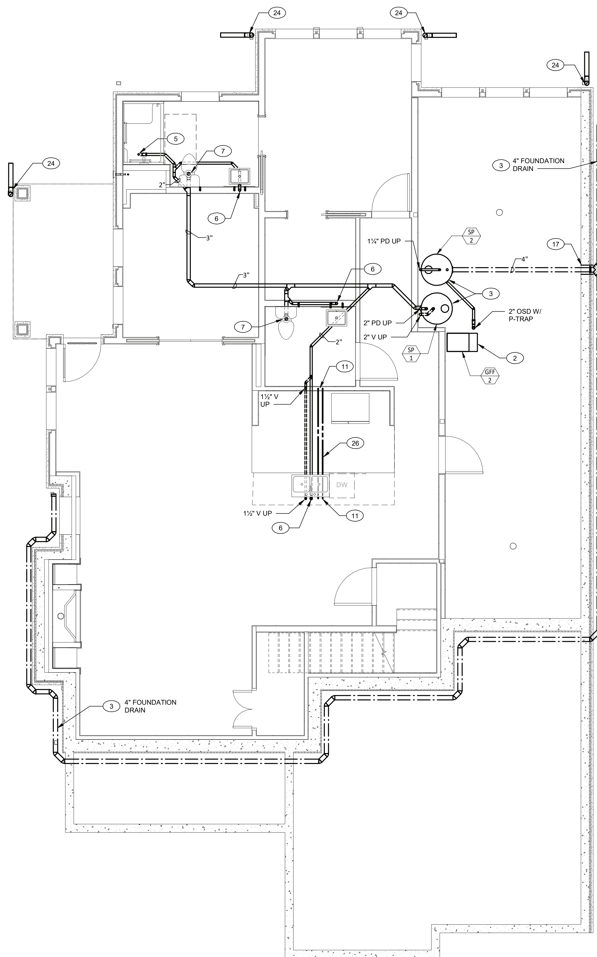
1 UNIT M - SHENOROCK II - BELOW BASEMENT FLOOR PLAN - PLUMBING 1/4" = 1'-0"
