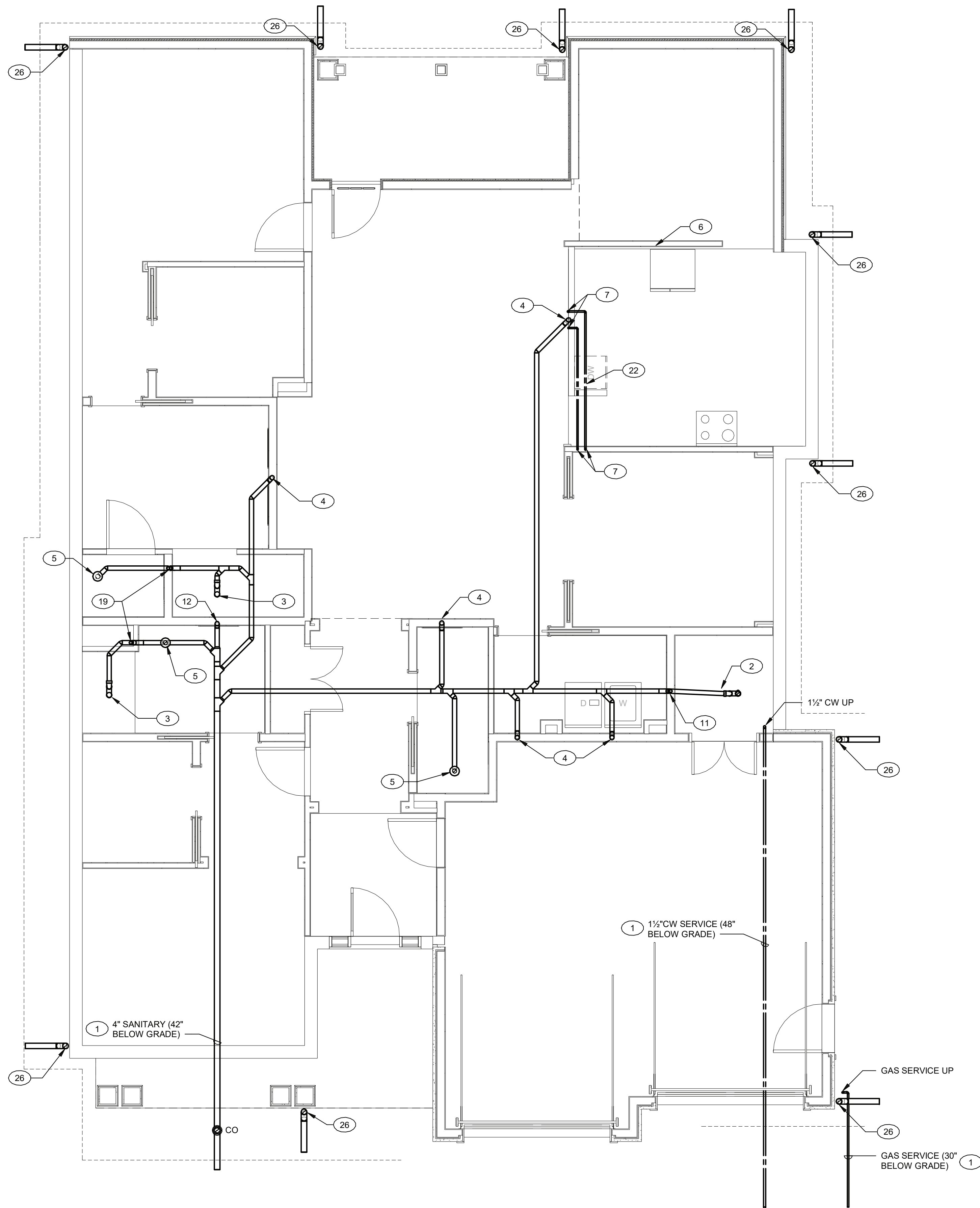
2 UNIT O - STRATHGLASS I - BELOW FLOOR PLAN - PLUMBING 1/4" = 1'-0"
