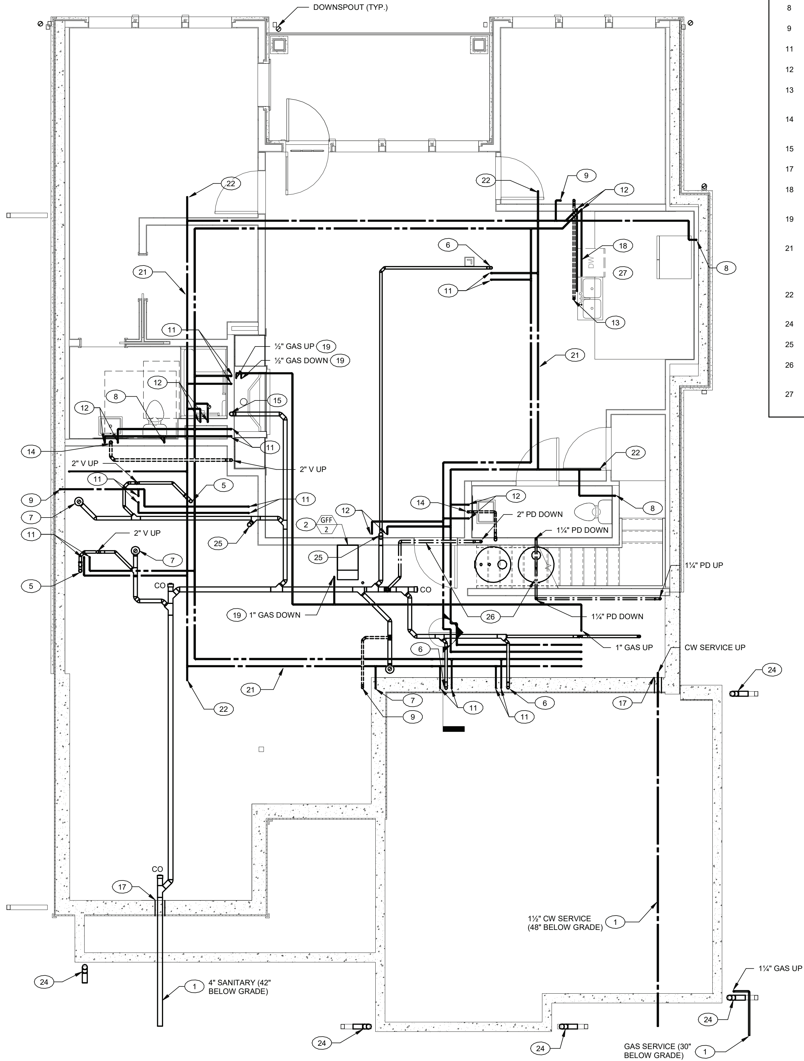
2 UNIT O - STRATHGLASS II - ABOVE BASEMENT FLOOR PLAN - PLUMBING 1/4" = 1'-0"
