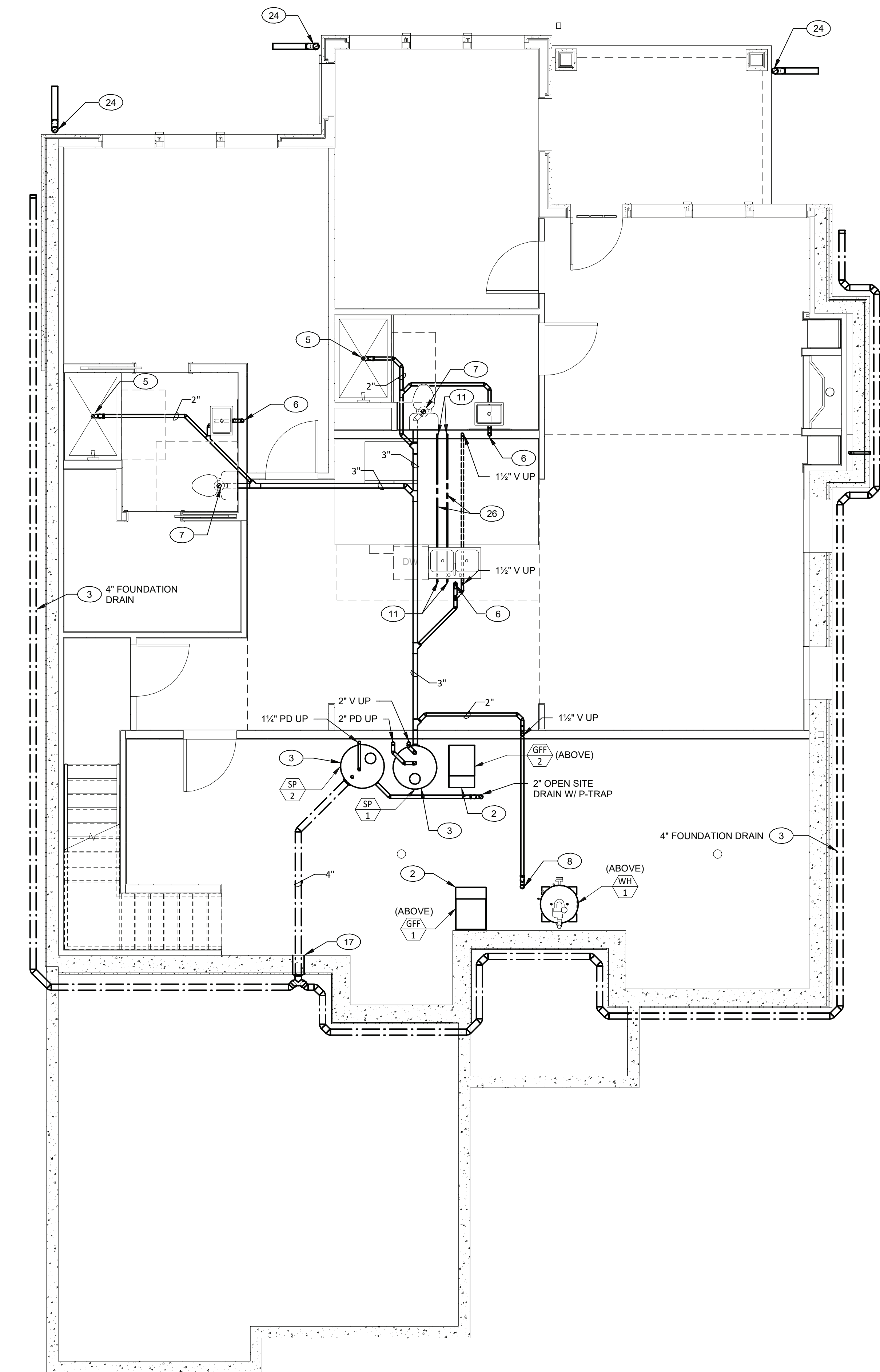
1 UNIT N - SIWANOY II - BELOW BASEMENT FLOOR PLAN - PLUMBING 1/4" = 1'-0"
