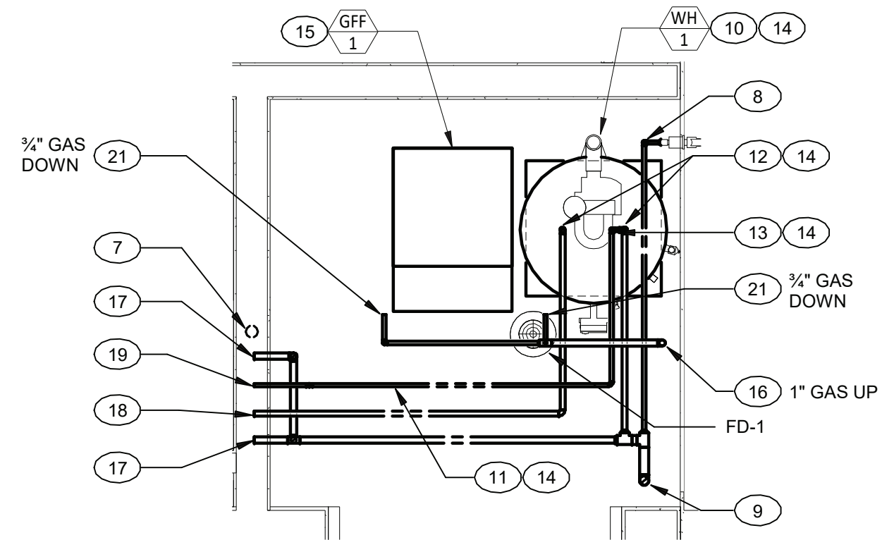
2 UNIT O - STRATHGLASS I - MECHANICAL ROOM PART PLAN 1/2" = 1'-0"
