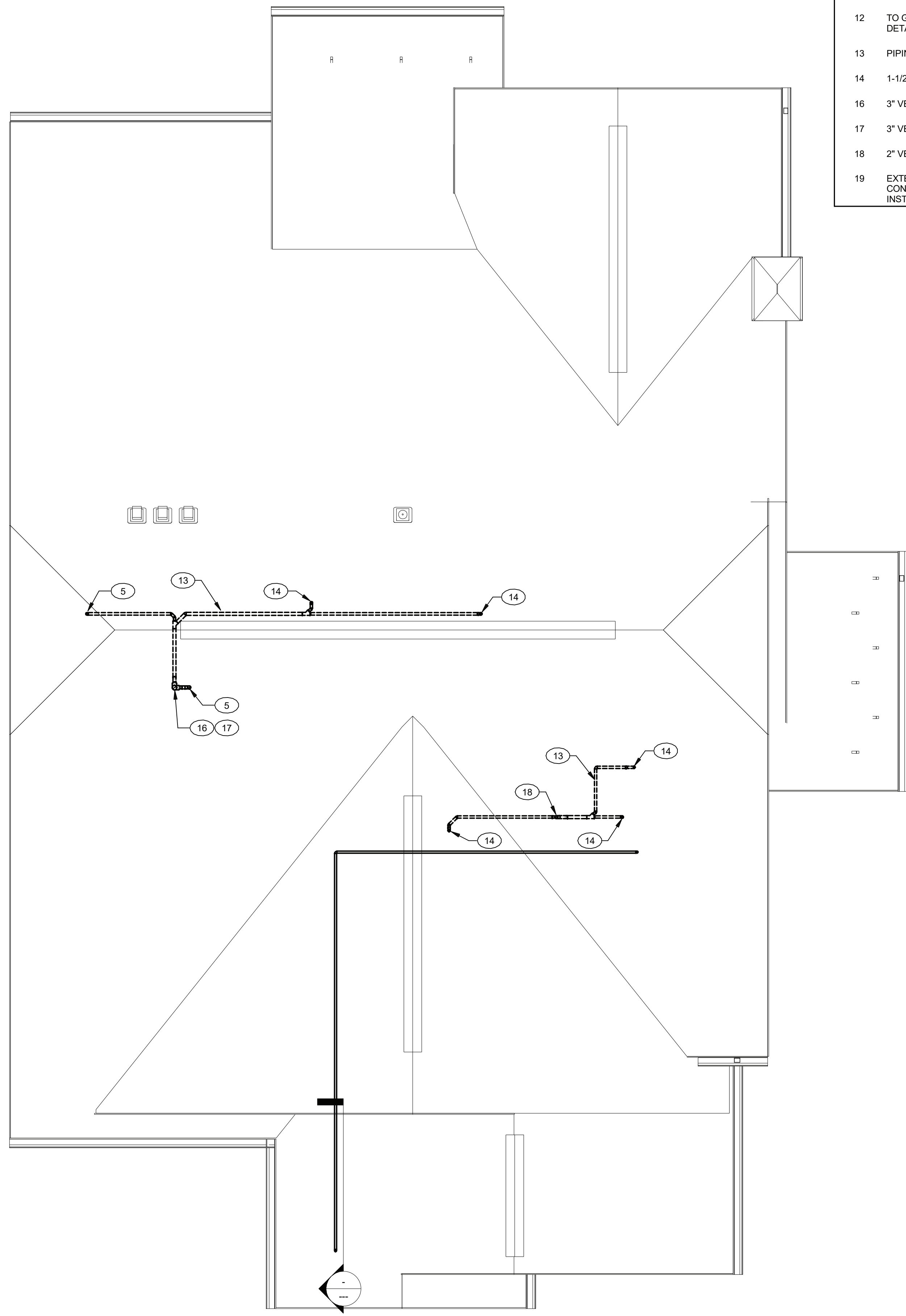
2 UNIT L - MAMARONECK II - ATTIC/ROOF PLAN - PLUMBING 1/4" = 1'-0"
