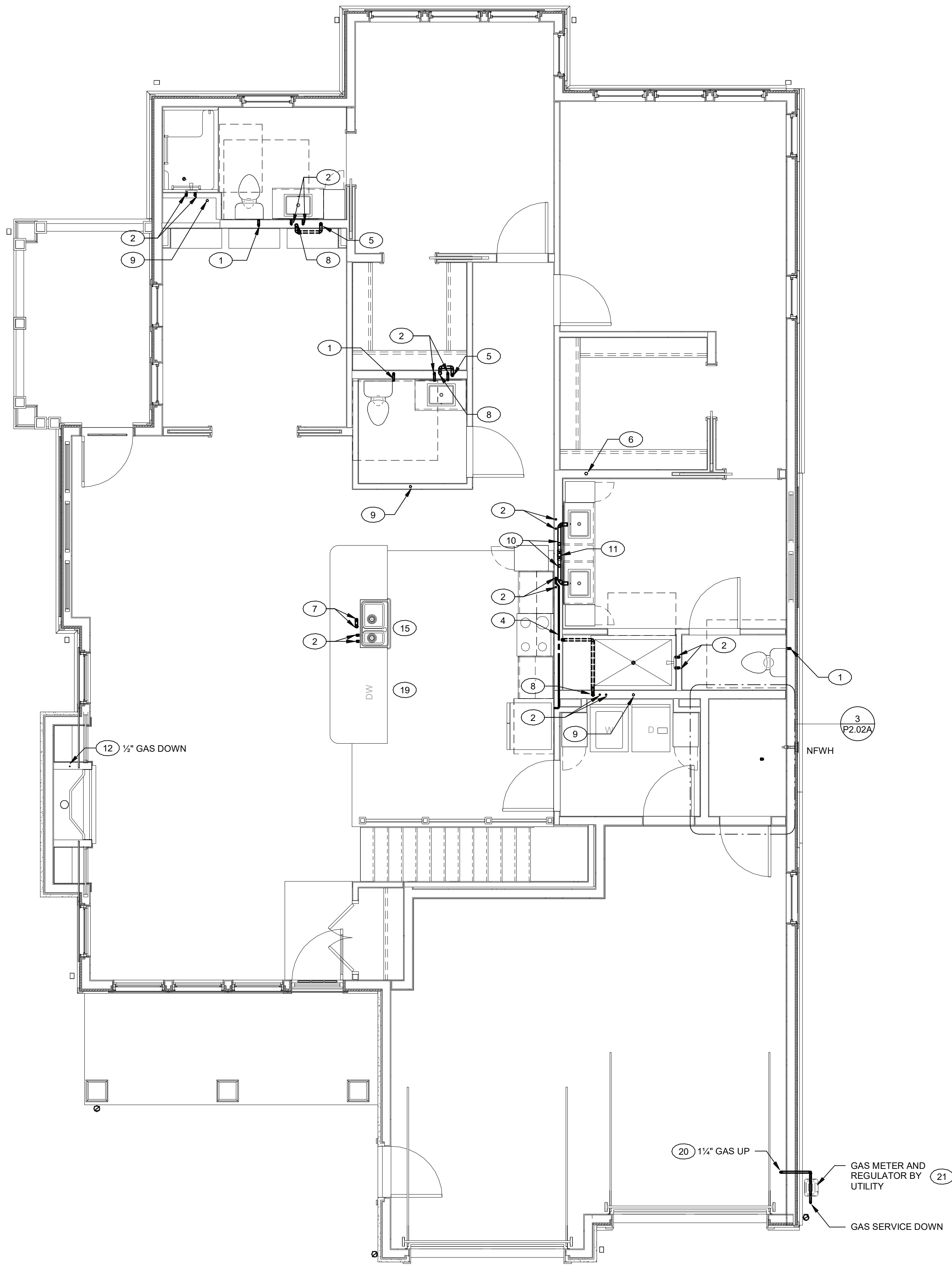
1 UNIT M - SHENOROCK II - FLOOR PLAN - PLUMBING 1/4" = 1'-0"
