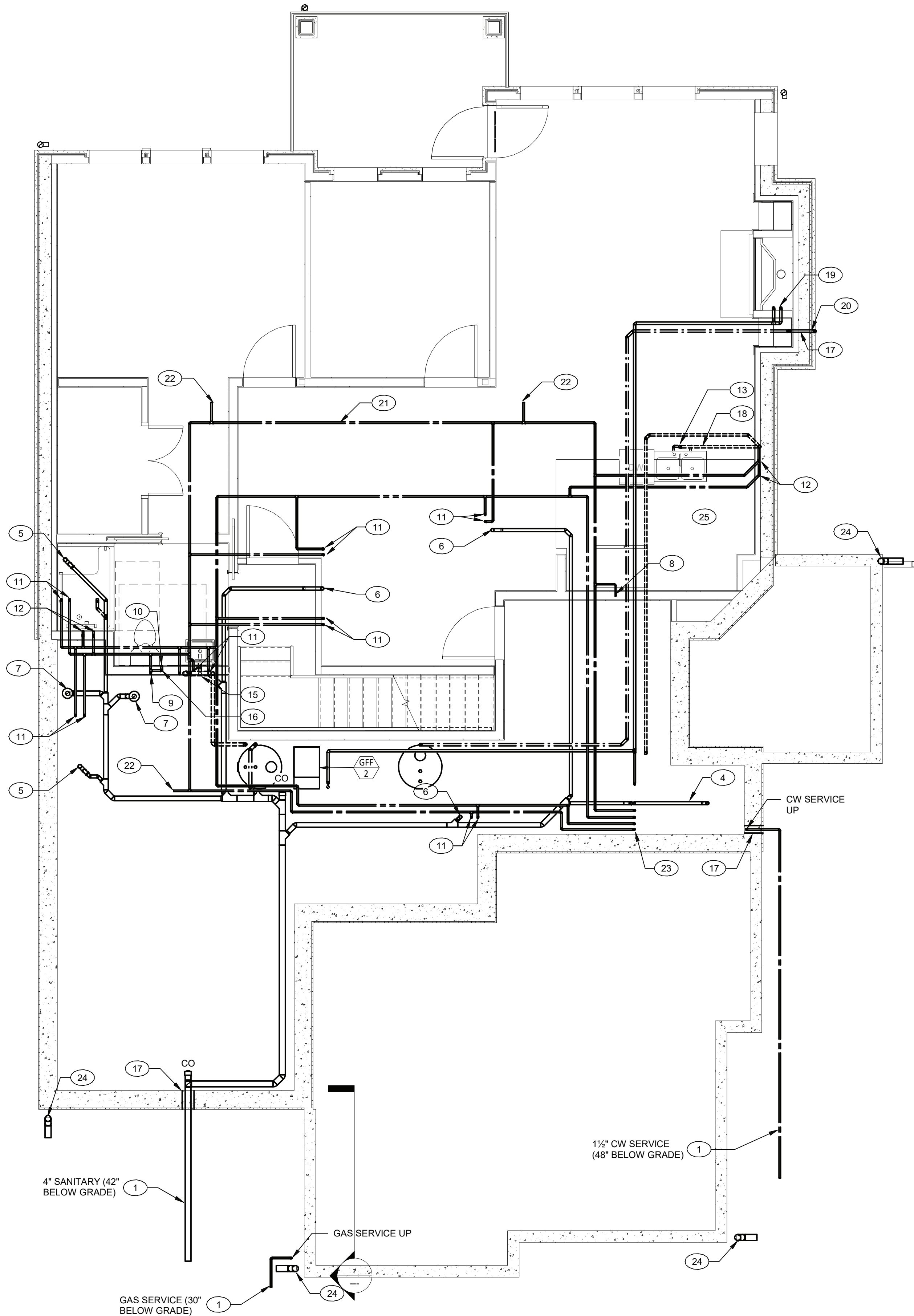
2 UNIT L - MAMARONECK II - ABOVE BASEMENT FLOOR PLAN - PLUMBING 1/4" = 1'-0"
