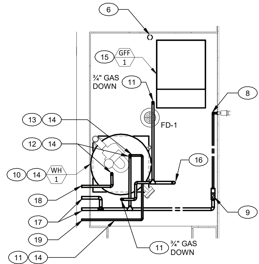
2 UNIT M - SHENOROCK I - MECHANICAL ROOM PART PLAN 1/2" = 1'-0"
