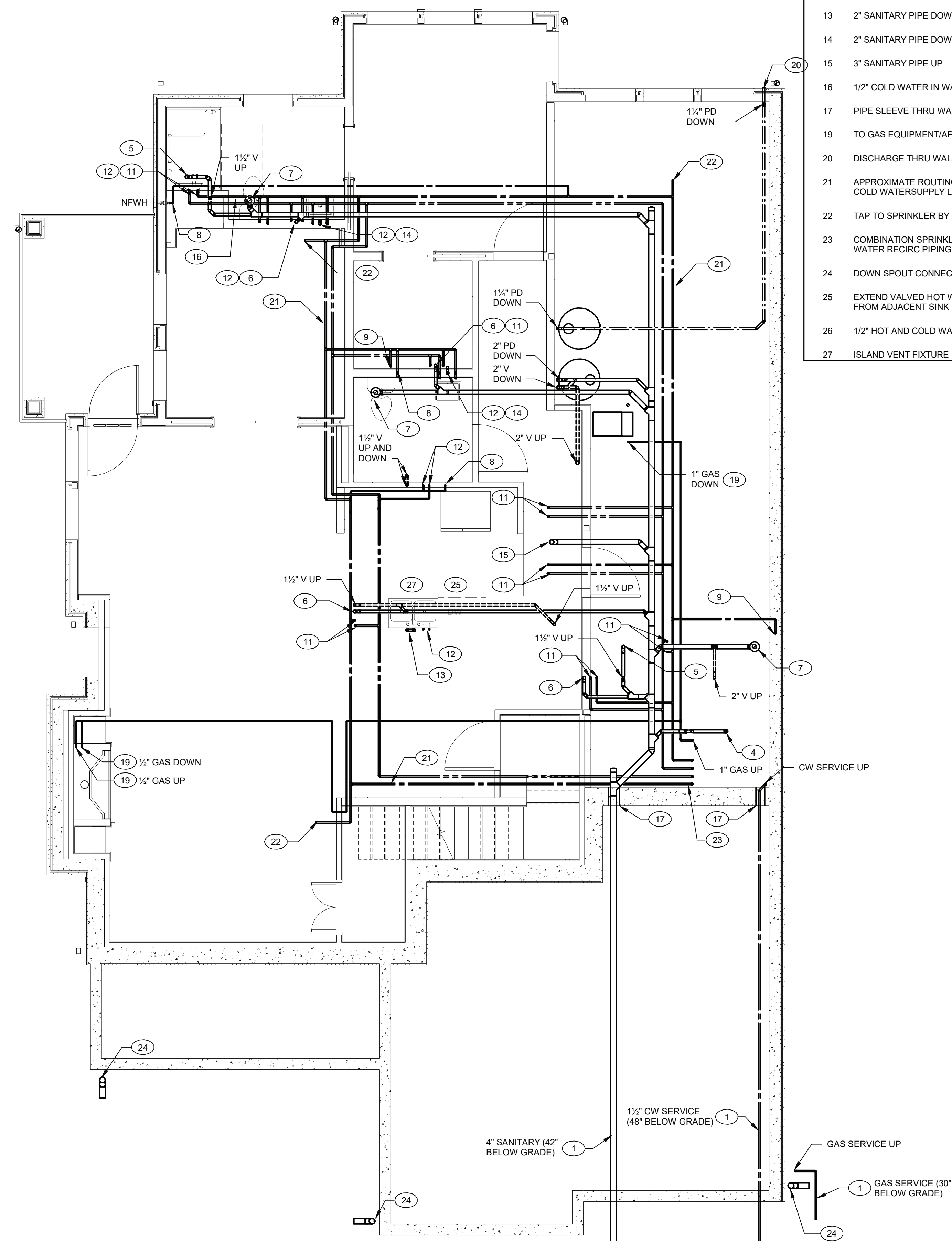
2 UNIT M - SHENOROCK II - ABOVE BASEMENT FLOOR PLAN - PLUMBING 1/4" = 1'-0"
