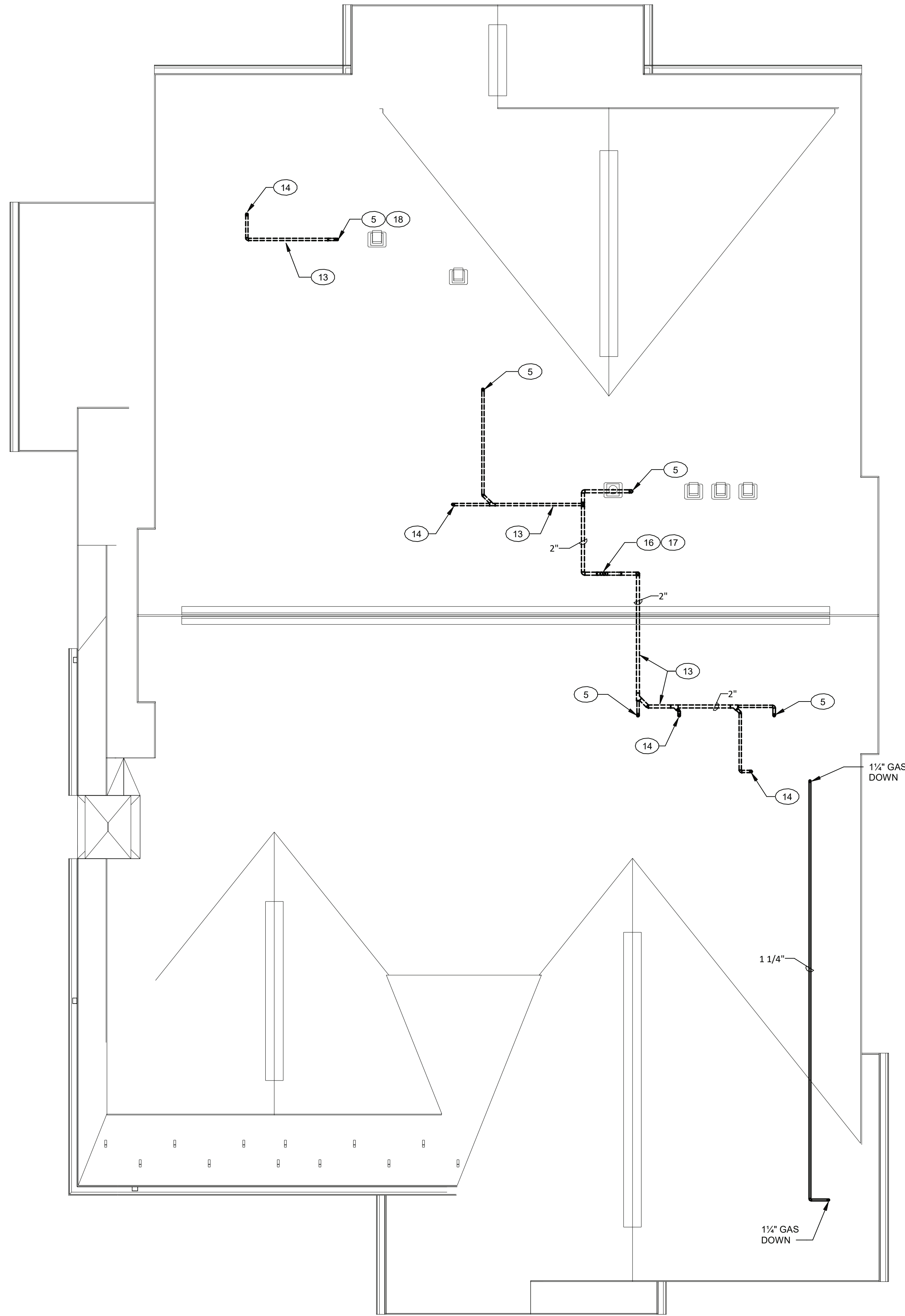
2 UNIT M - SHENOROCK II - ATTIC/ROOF PLAN - PLUMBING 1/4" = 1'-0"
