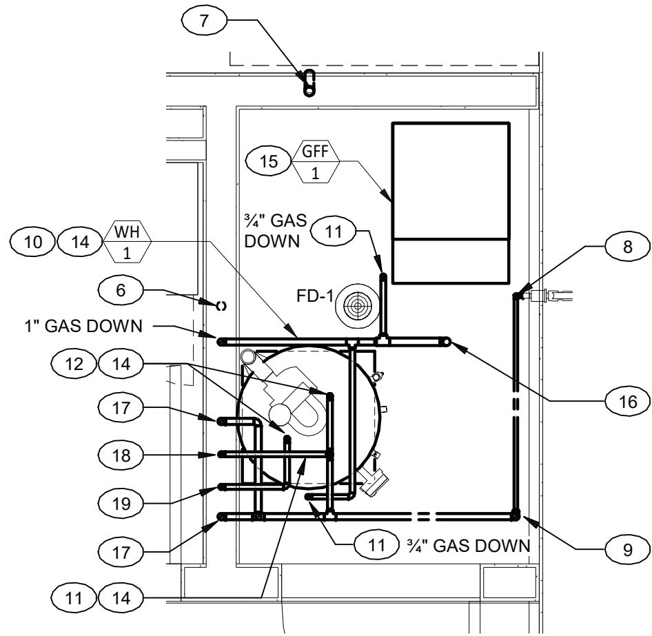
3 UNIT M - SHENOROCK II - MECHANICAL ROOM PART PLAN 1/2" = 1'-0"
