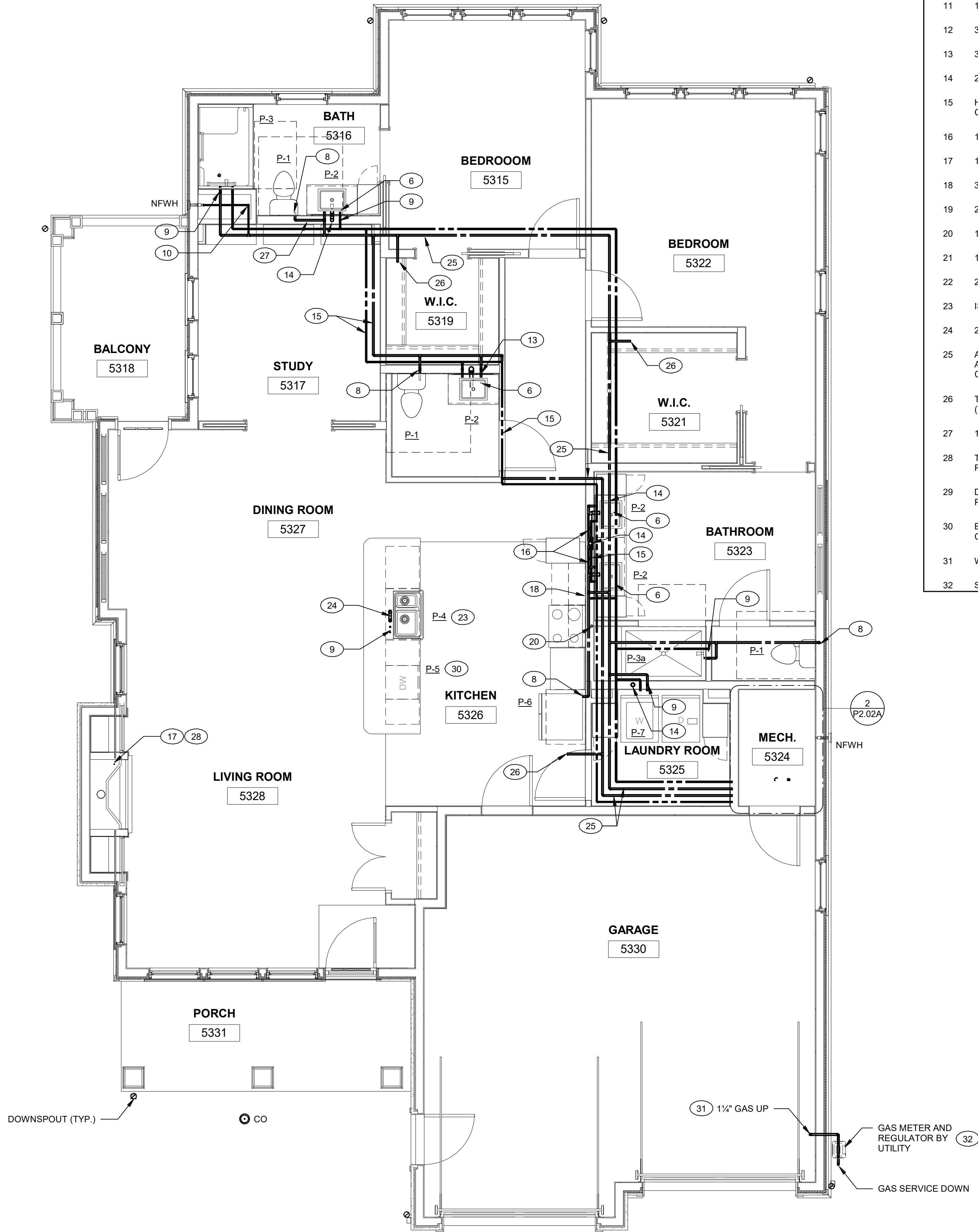
1 UNIT M - SHENOROCK I - FLOOR PLAN - PLUMBING 1/4" = 1'-0"
