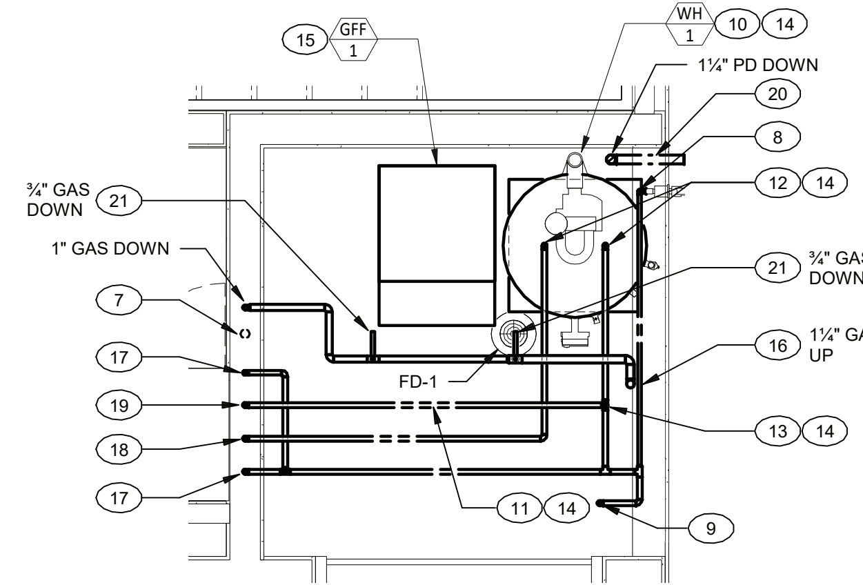
3 UNIT O - STRATHGLASS II - MECHANICAL ROOM PART PLAN 1/2" = 1'-0"
