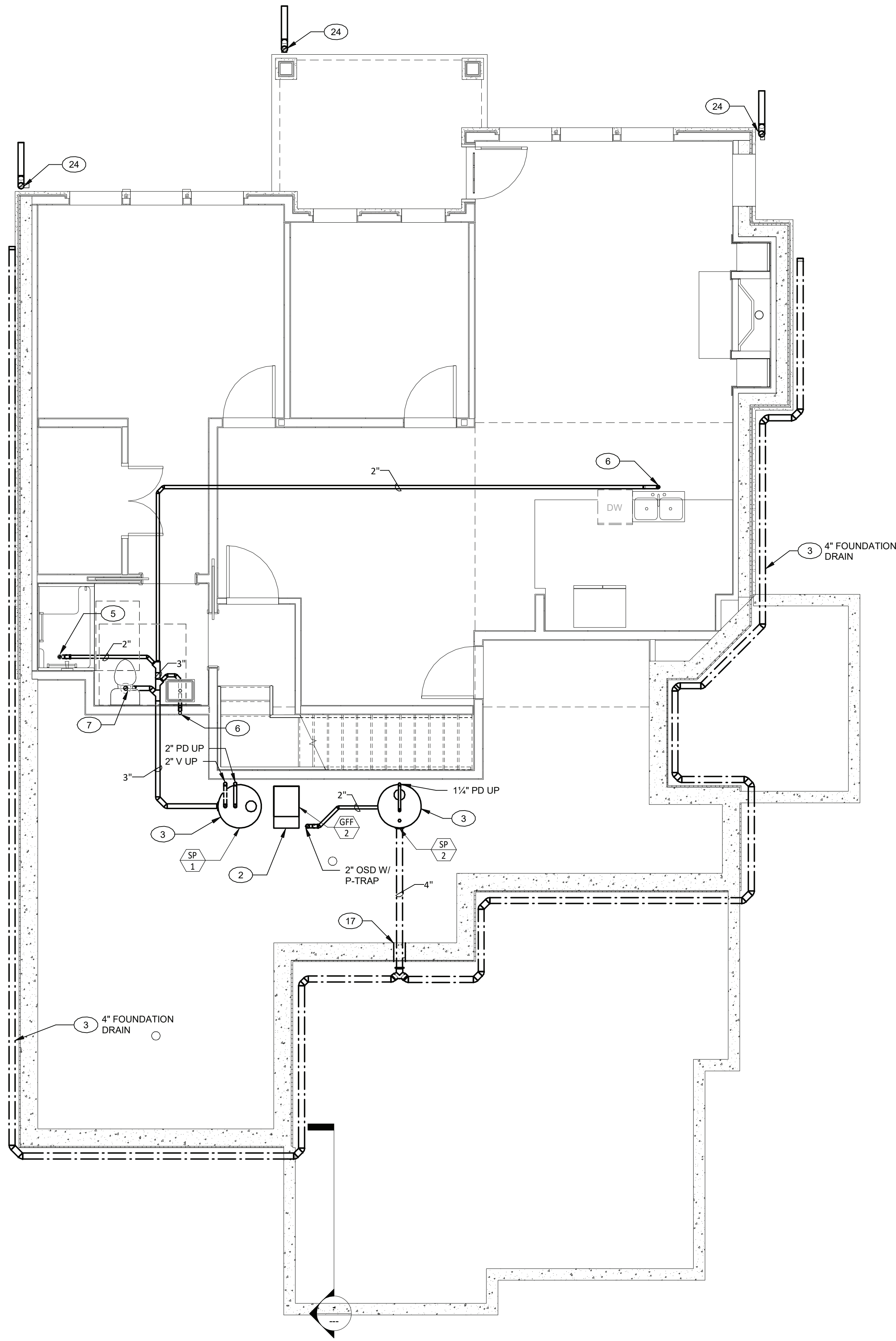
1 UNIT L - MAMARONECK II - BELOW BASEMENT FLOOR PLAN - PLUMBING 1/4" = 1'-0"
