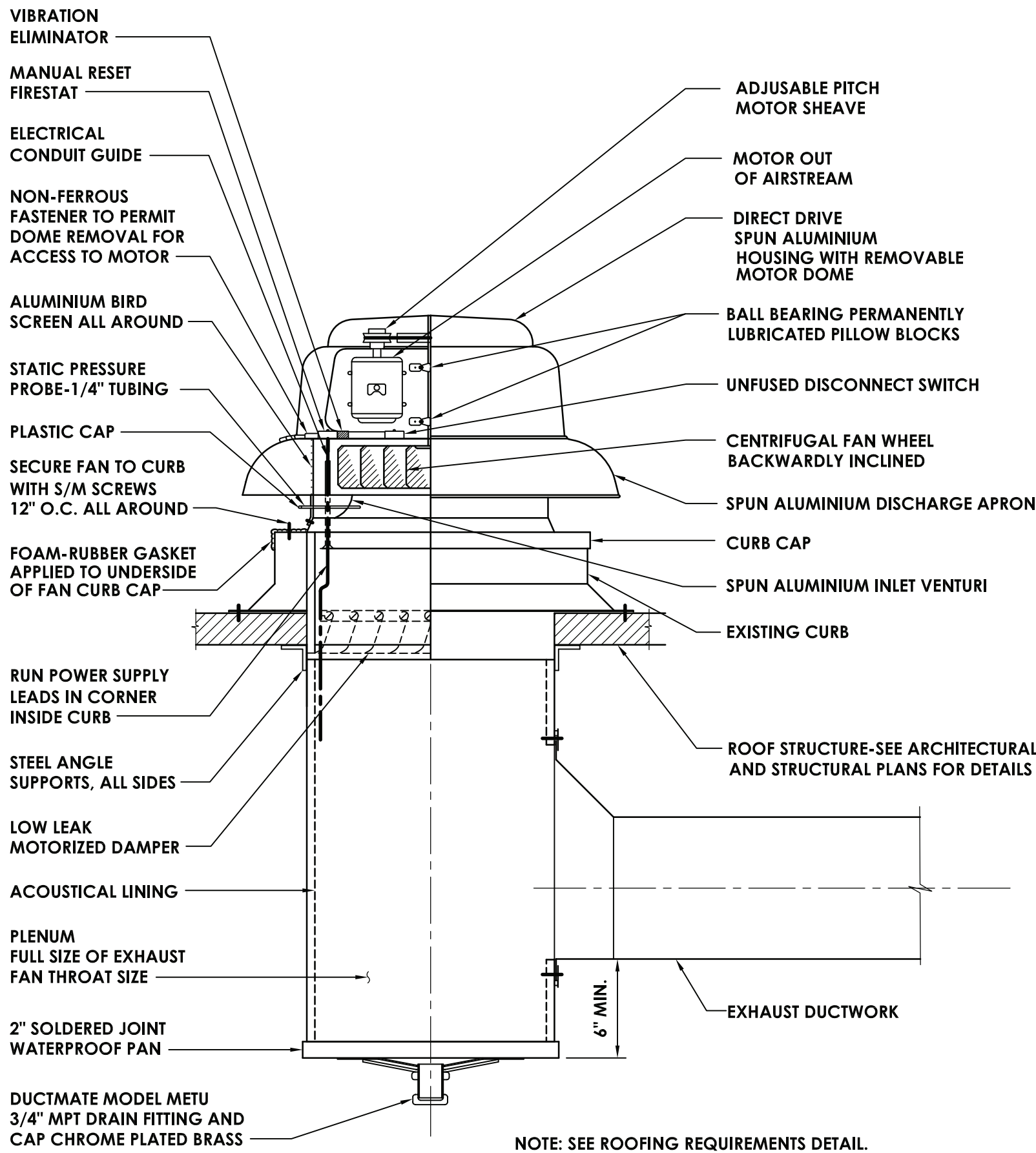
6 EXHAUST FAN DETAIL H201 NOT TO SCALE
