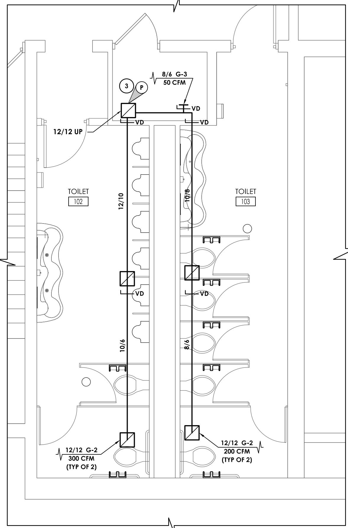
2 TOILET ROOMS #102 & #103 NEW WORK PLAN H201 SCALE: 1/4" = 1'-0"
