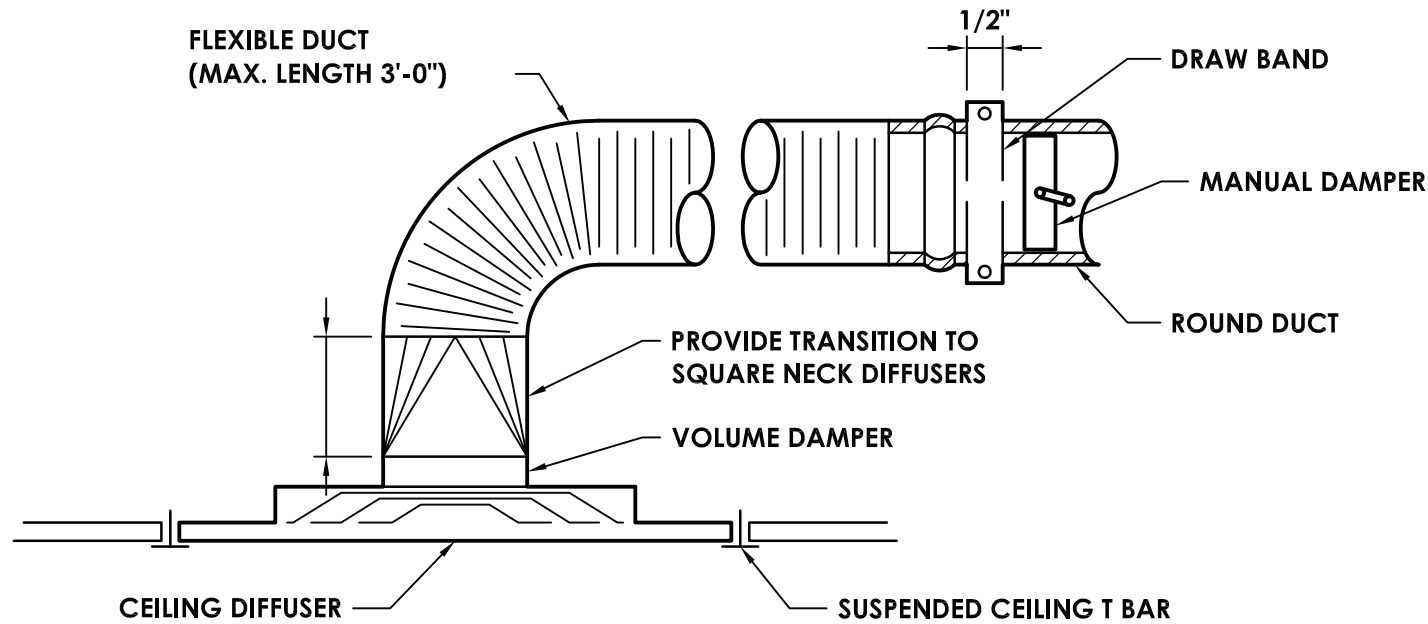
7 DIFFUSER DETAIL H201 NOT TO SCALE
