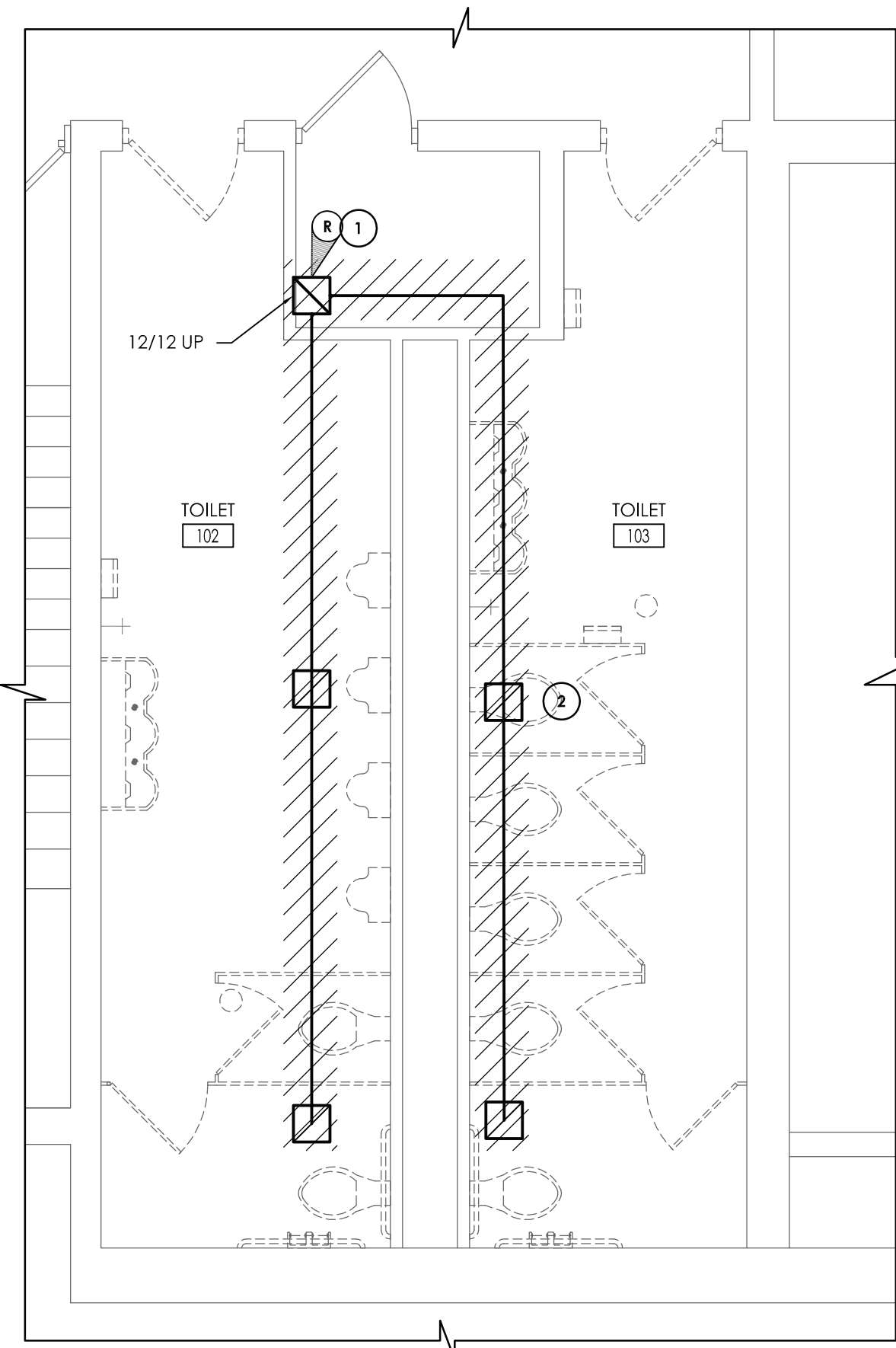
1 TOILET ROOMS #102 & #103 DEMOLITION PLAN H201 SCALE: 1/4" = 1'-0"
