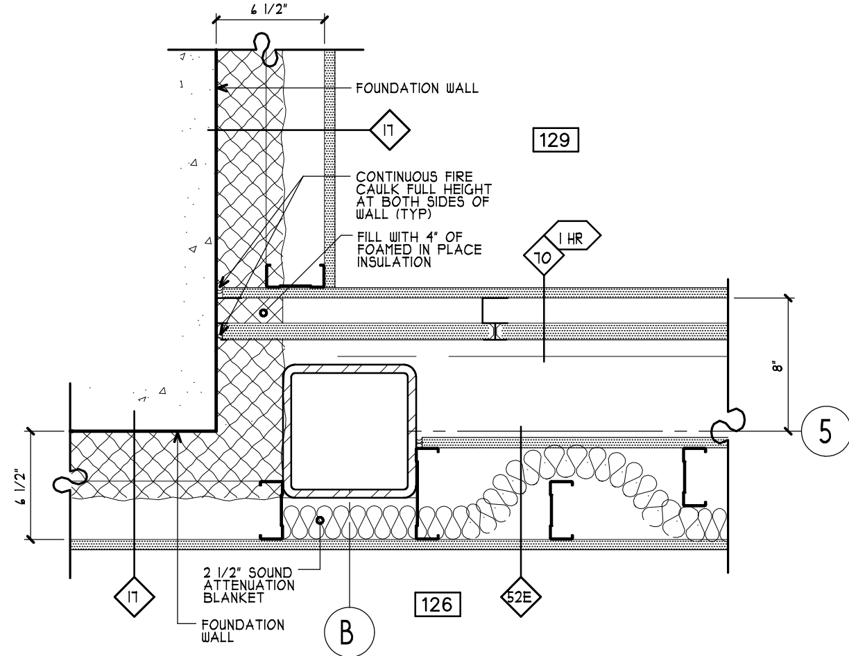
8 PLAN DETAIL (1 FLR) A405 SCALE: 1 1/2" = 1'-0" A100
