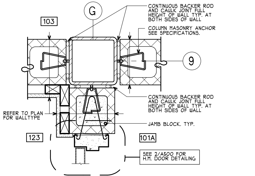
6 PLAN DETAIL (1 FLR) A405 SCALE: 1 1/2" = 1'-0" A100
