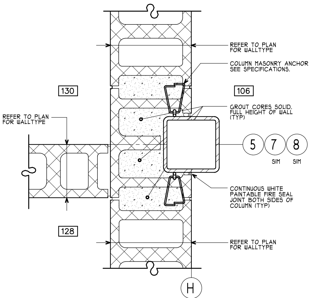
4 PLAN DETAIL (1 FLR) A405 SCALE: 1 1/2" = 1'-0" A100
