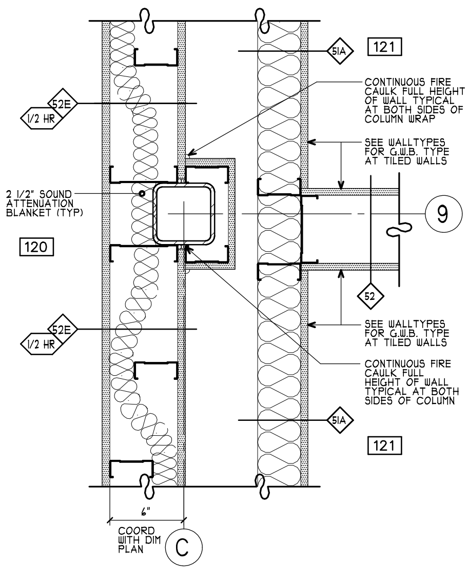
11 PLAN DETAIL (1 FLR) A405 SCALE: 1 1/2" = 1'-0" A100
