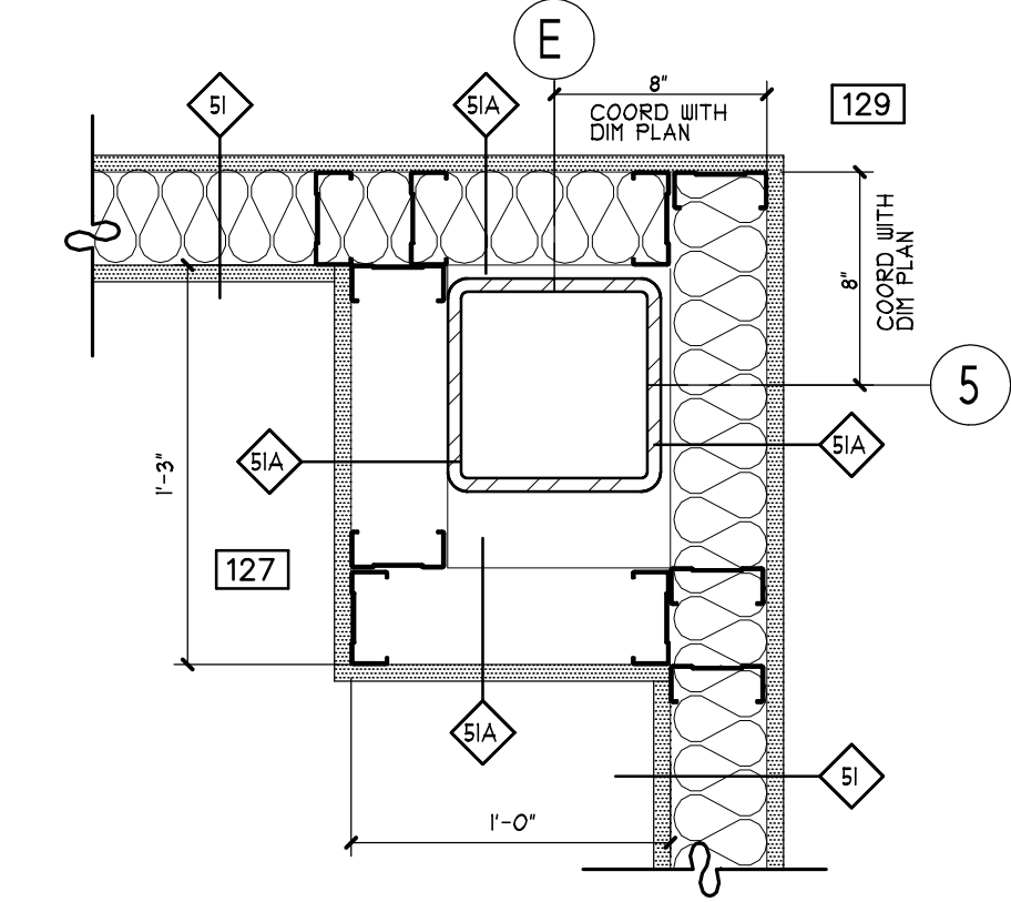
12 PLAN DETAIL (1 FLR) A405 SCALE: 1 1/2" = 1'-0" A100
