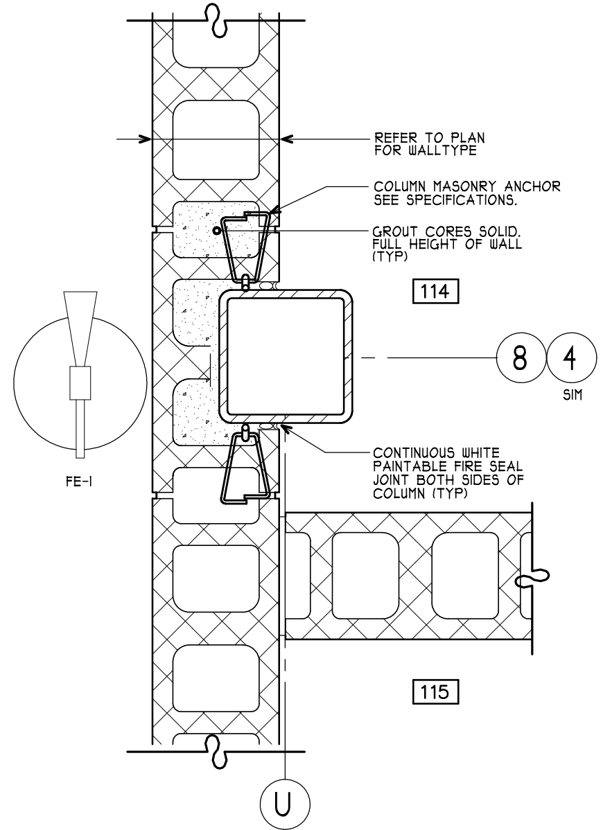
2 PLAN DETAIL (1 FLR) A405 SCALE: 1 1/2" = 1'-0" A100
