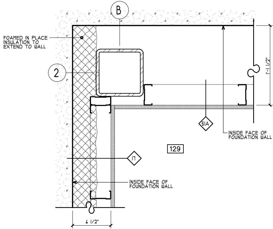
7 PLAN DETAIL (1 FLR) A405 SCALE: 1 1/2" = 1'-0" A100
