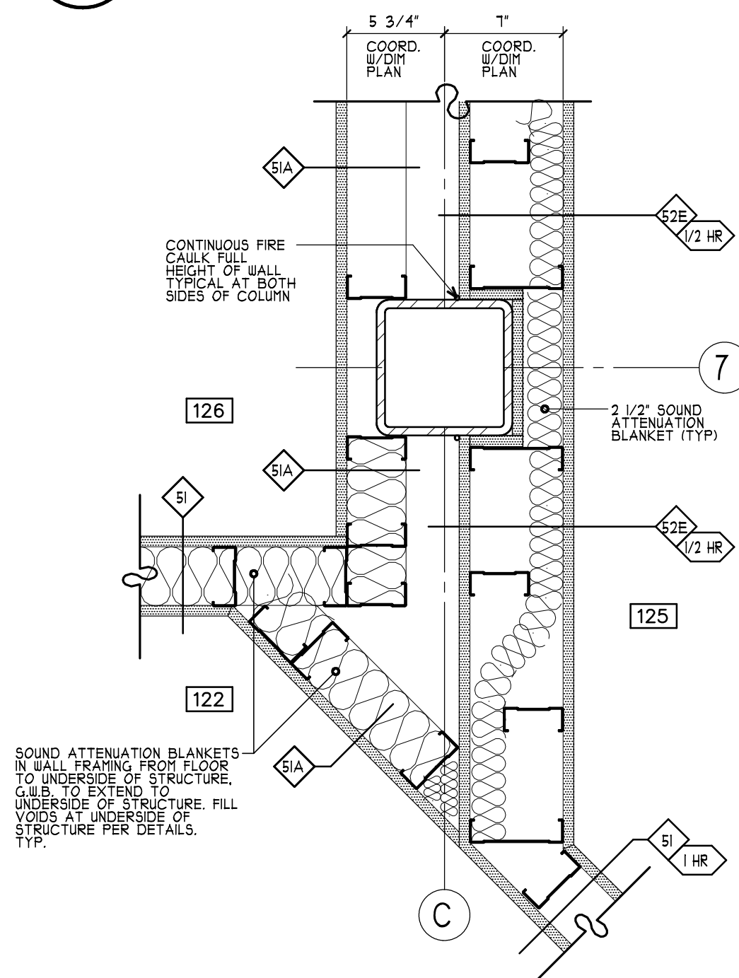
10 PLAN DETAIL (1 FLR) A405 SCALE: 1 1/2" = 1'-0" A100
