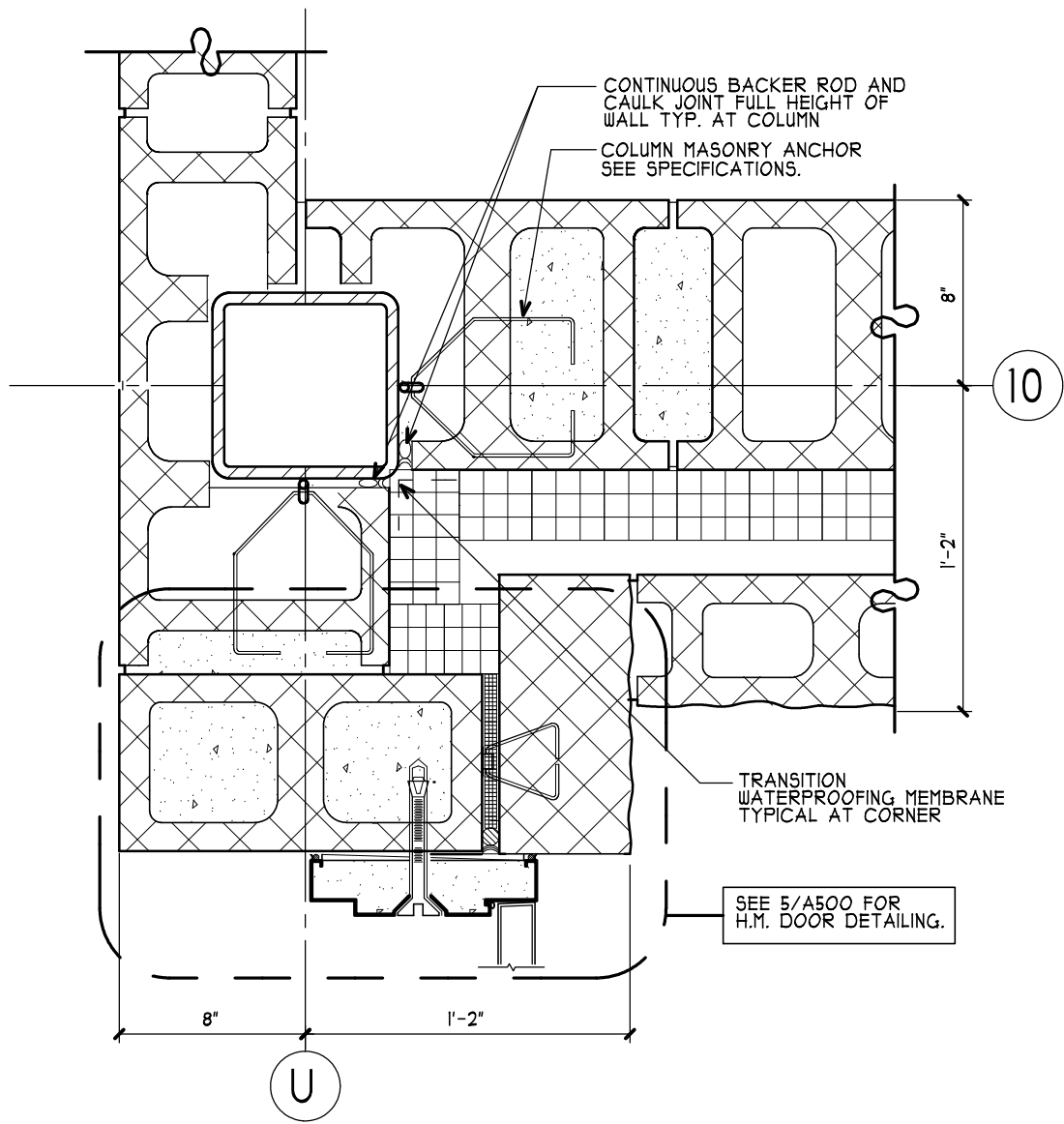
3 PLAN DETAIL (1 FLR) A405 SCALE: 1 1/2" = 1'-0" A100
