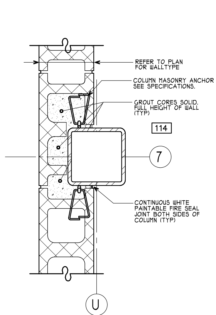
1 PLAN DETAIL (1 FLR) A405 SCALE: 1 1/2" = 1'-0" A100
