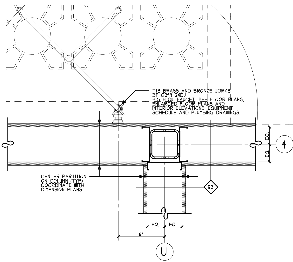
14 PLAN DETAIL (3 FLR) A405 SCALE: 1 1/2" = 1'-0" A102
