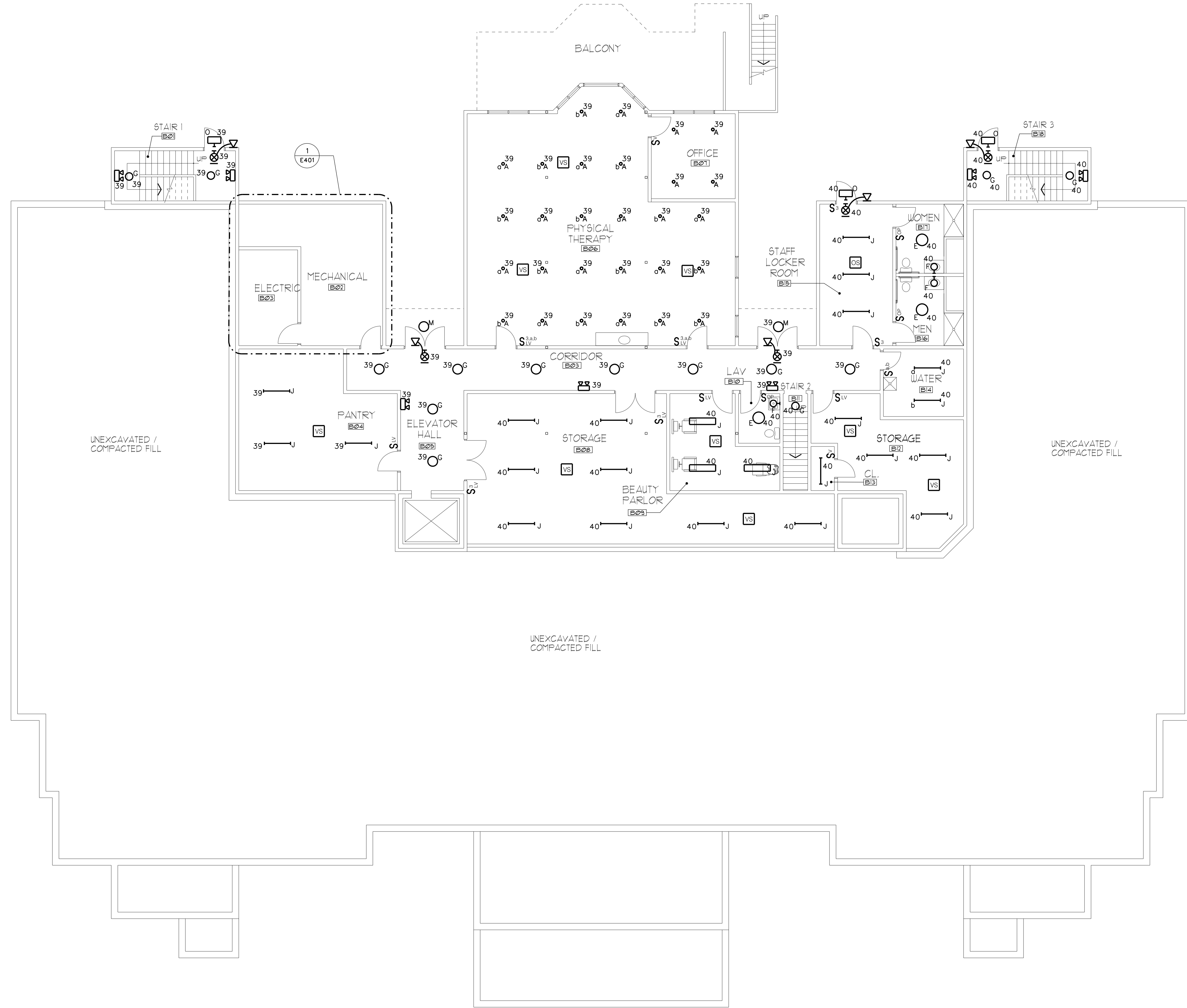
1 BASEMENT FLOOR PLAN SCALE: 1/8"=1'-0" NORTH 0 4' 8' 16'
