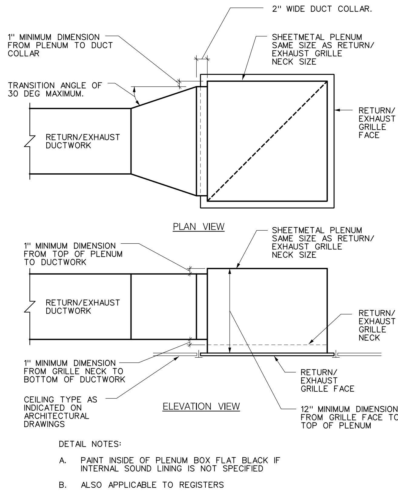
2 RETURN/ EXHAUST GRILLE PLENUM DETAIL SCALE: NONE DUCTED
