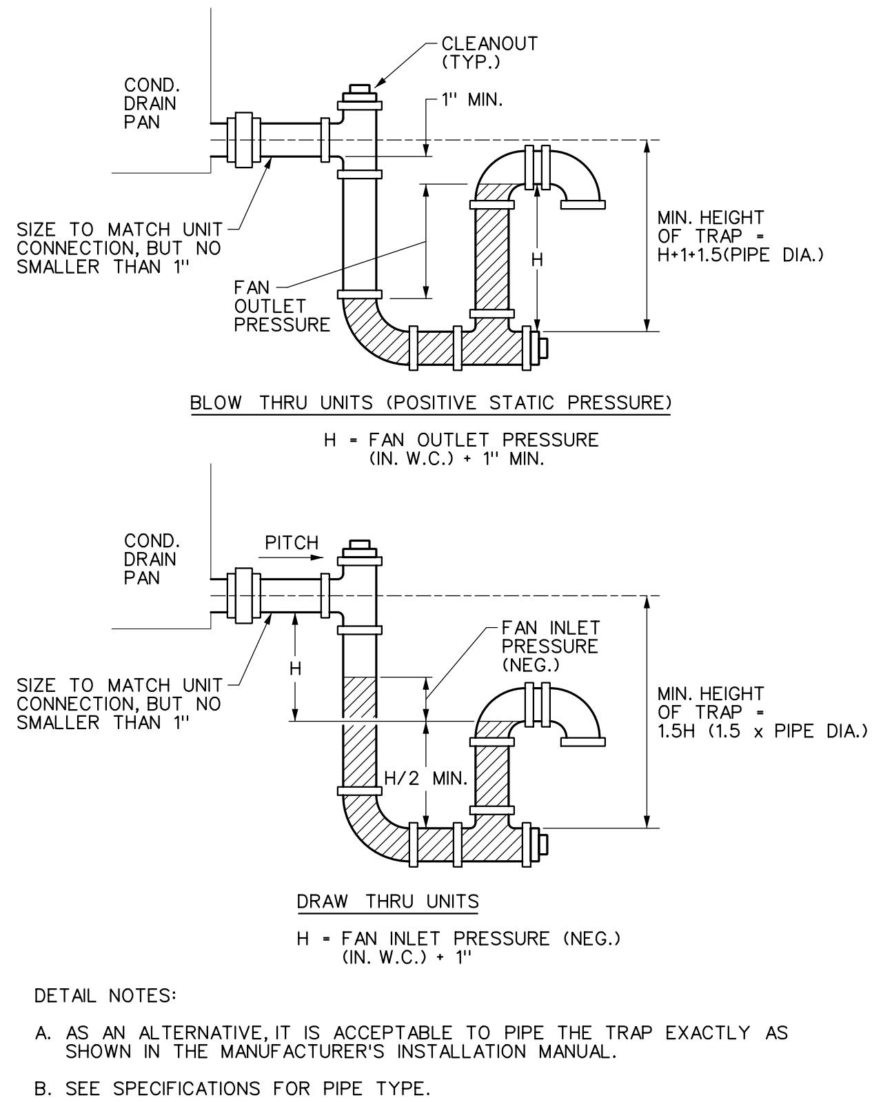
5 ROOFTOP UNIT CONDENSATE DRAIN TRAP DETAIL SCALE: NONE
