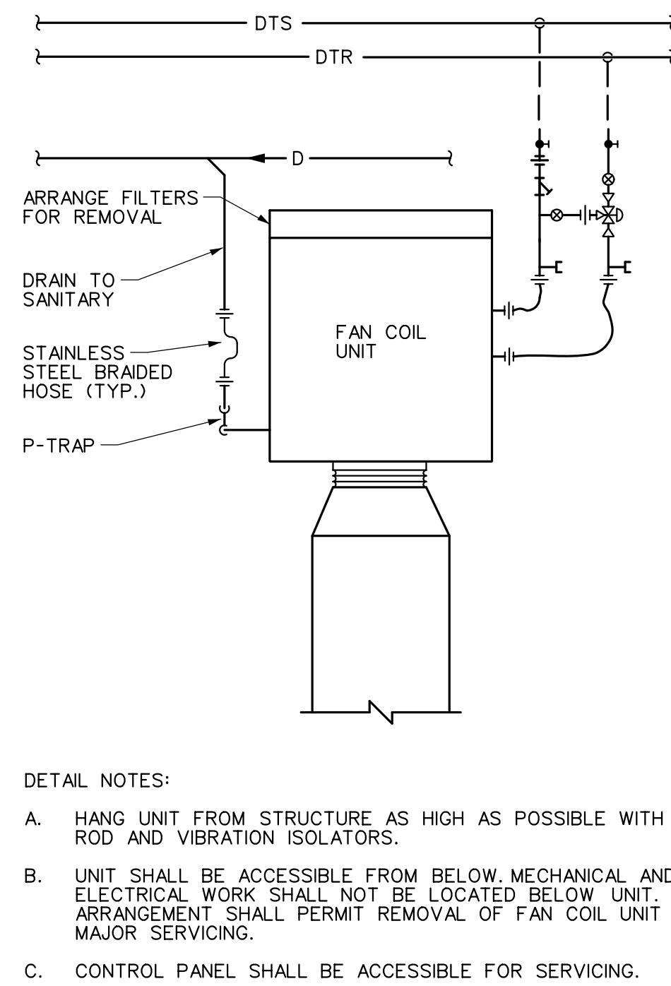
7 CEILING MOUNTED FAN COIL UNIT DETAIL SCALE: NONE DUAL TEMP
