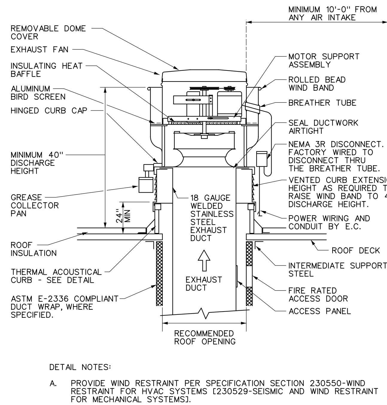
6 KITCHEN EXHAUST FAN DETAIL SCALE: NONE
