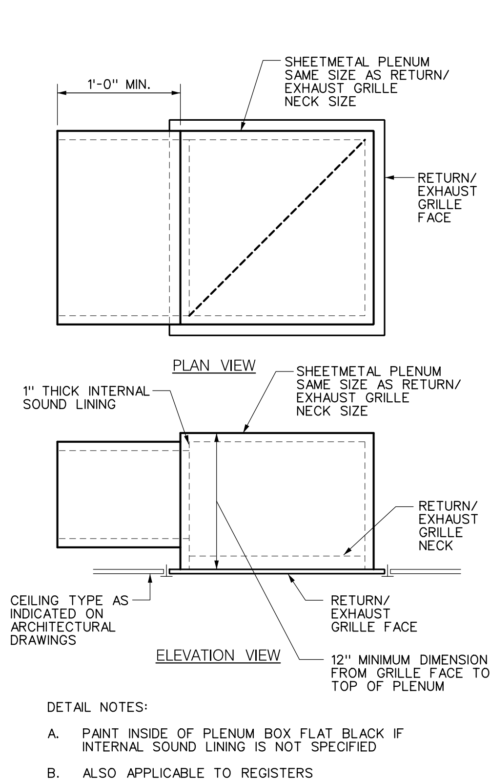
1 RETURN/ EXHAUST GRILLE PLENUM DETAIL SCALE: NONE NON-DUCTED
