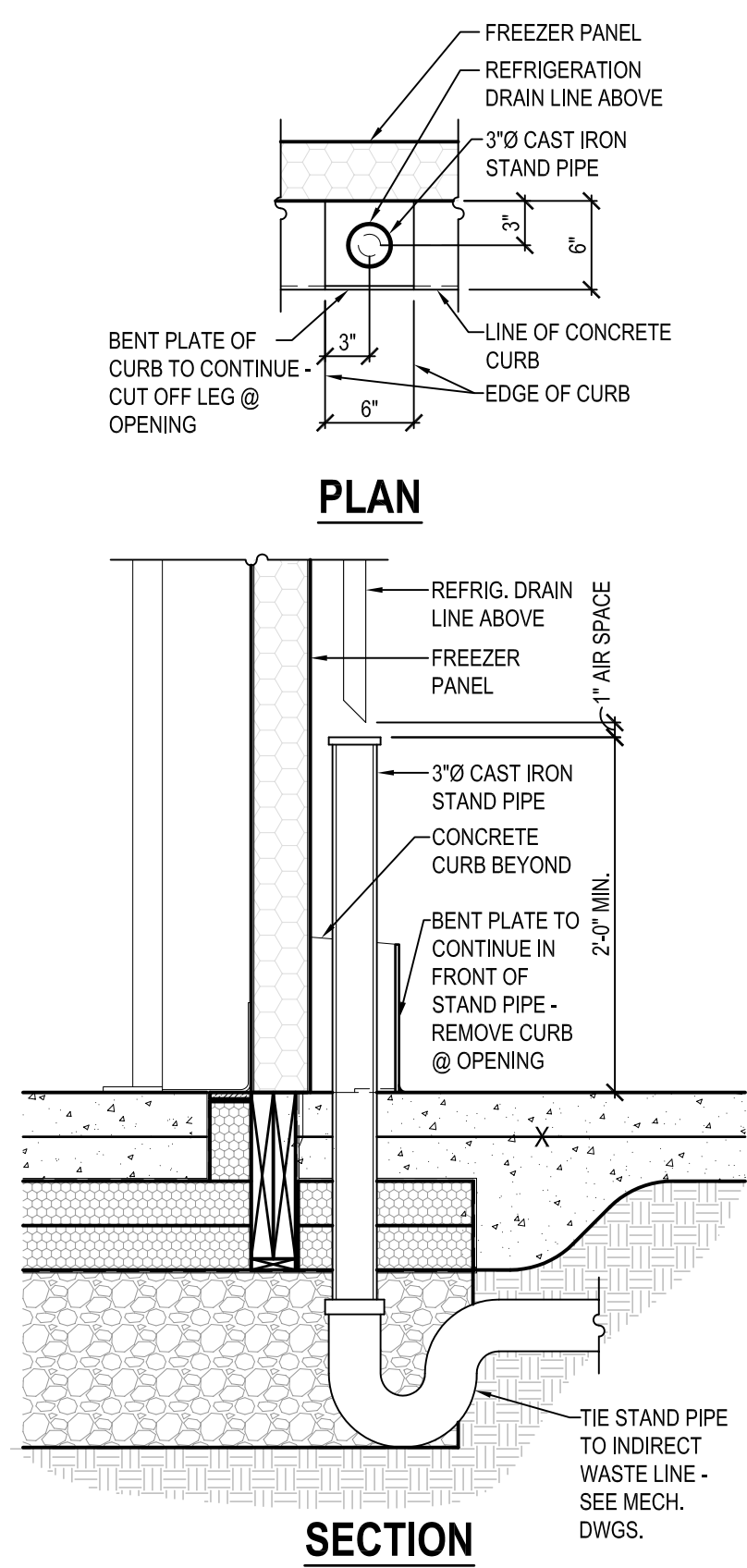
F STANDPIPE DETAILS SCALE: 1"=1'-0"
