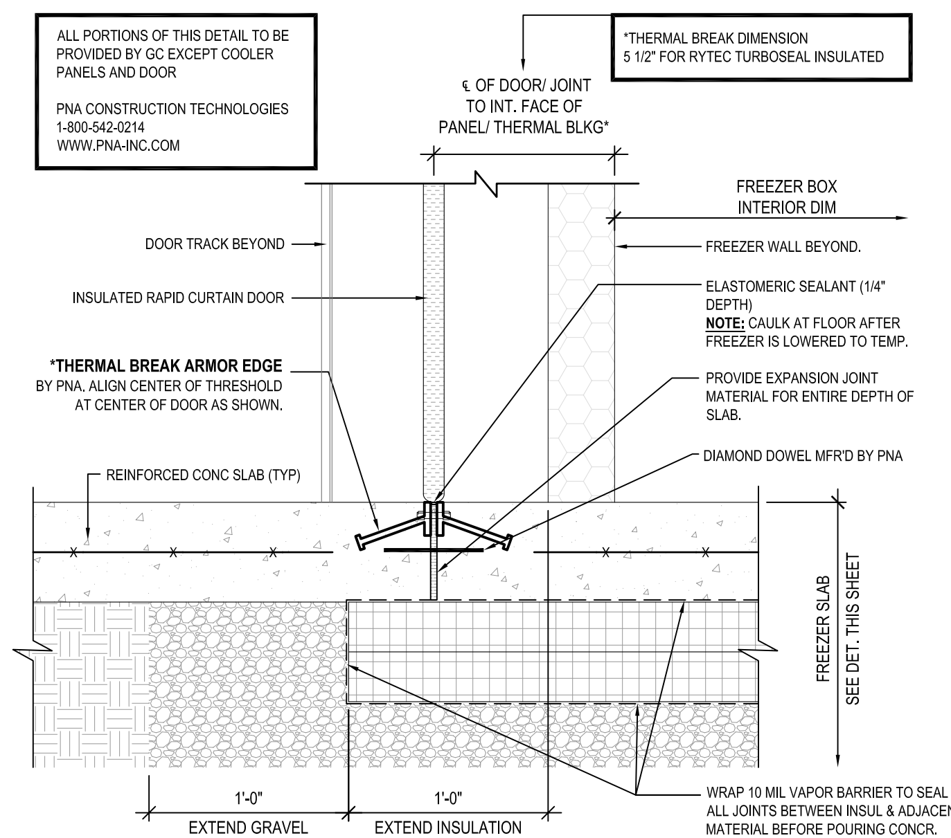
B1 FREEZER HIGH SPEED DOOR SILL PLATE SCALE: 1 1/2\"=1'-0"
