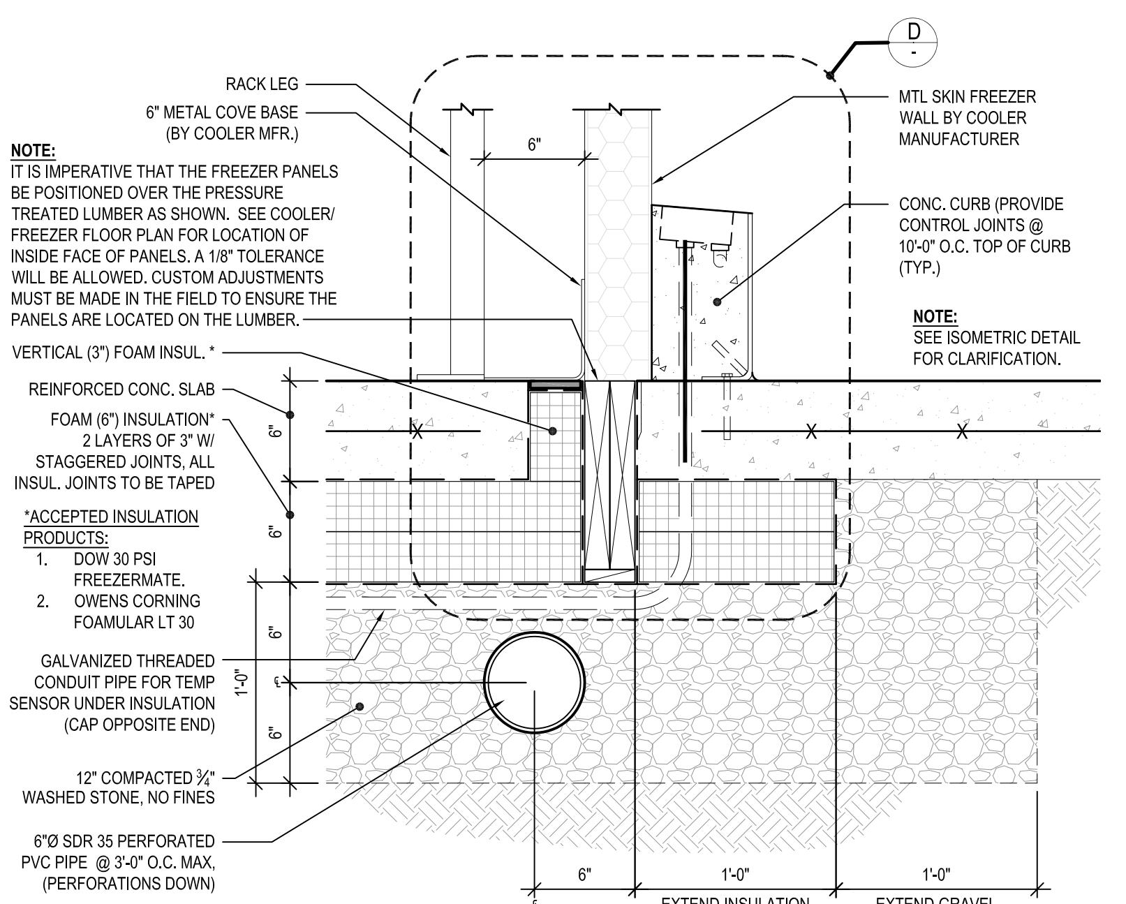
C FREEZER CURB & SLAB SCALE: 1 1/2\"=1'-0"
