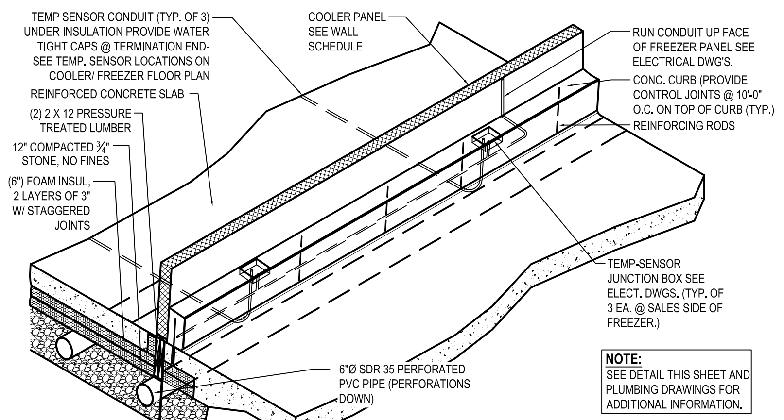
E PARTIAL ISOMETRIC FREEZER CURB & SLAB SCALE: 1/2\"=1'-0"
