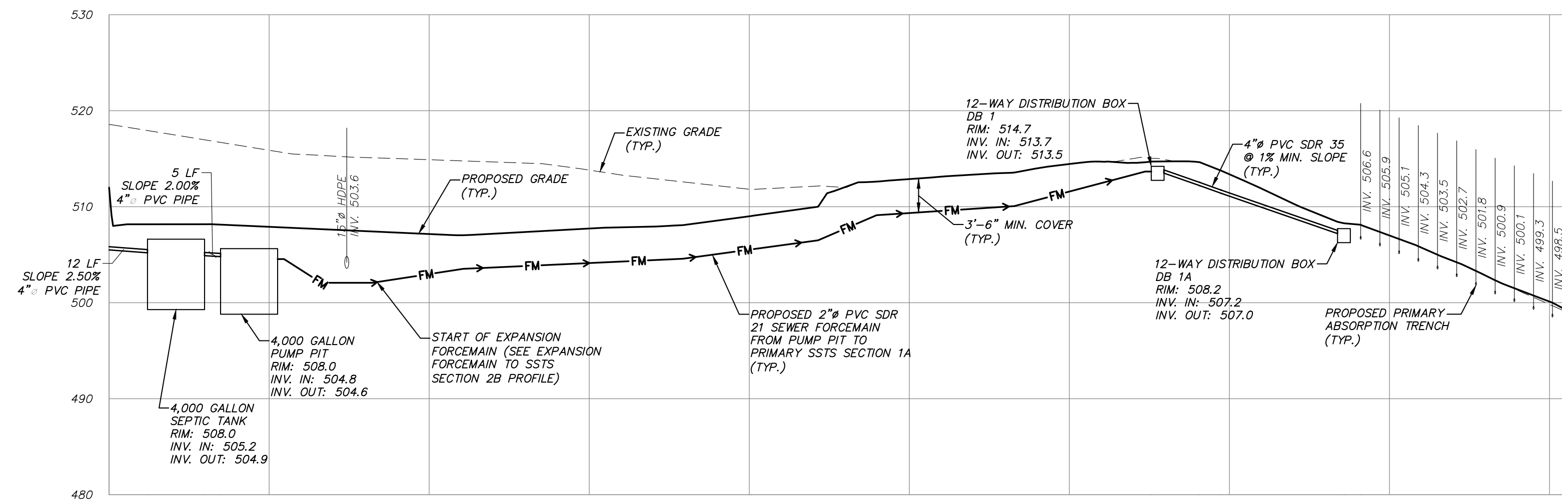
PROPOSED BUILDING TO PRIMARY SSTS SECTION 1A PROFILE
