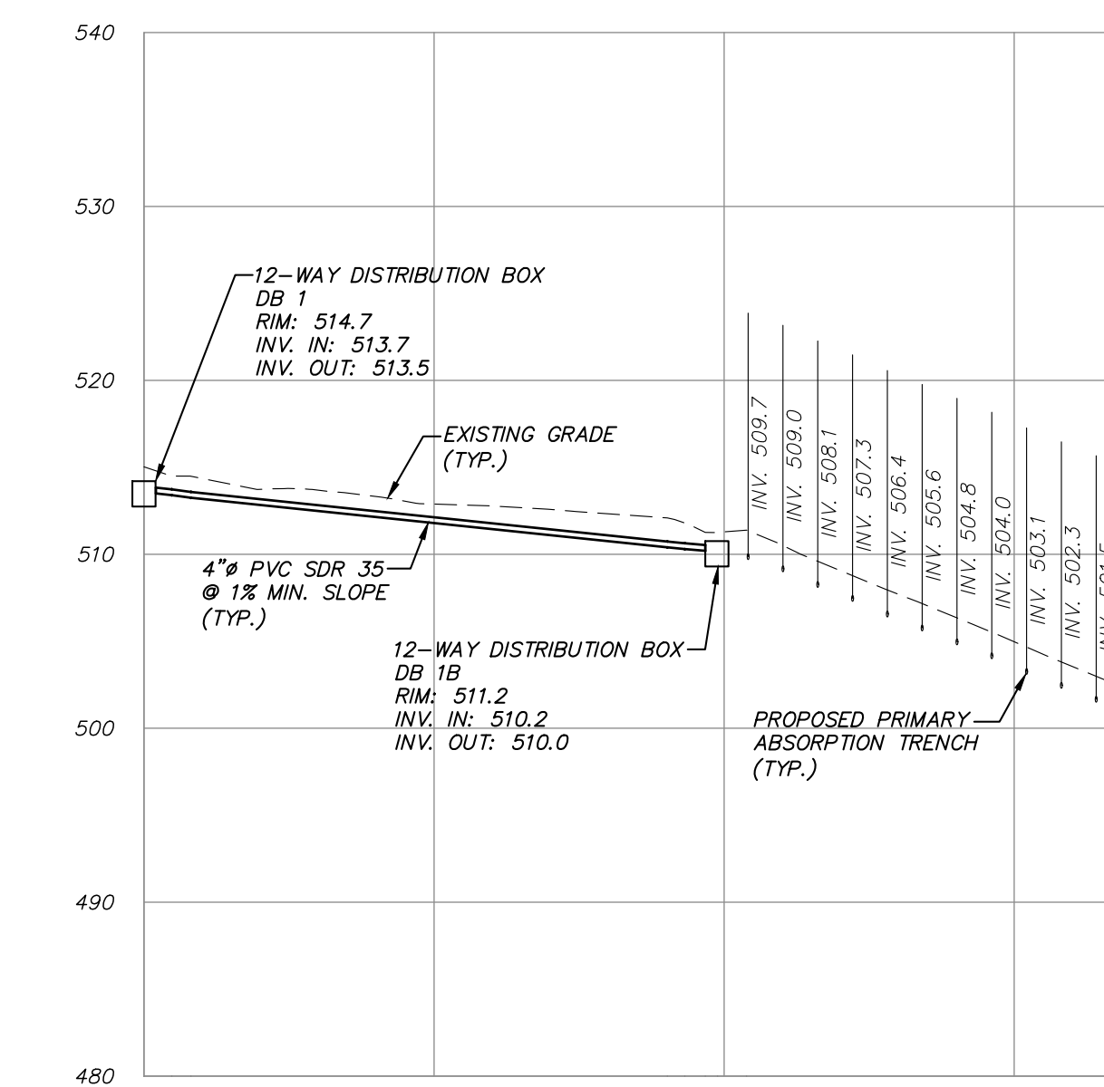
DISTRIBUTION BOX DB 1 TO PRIMARY SSTS SECTION 1B PROFILE
