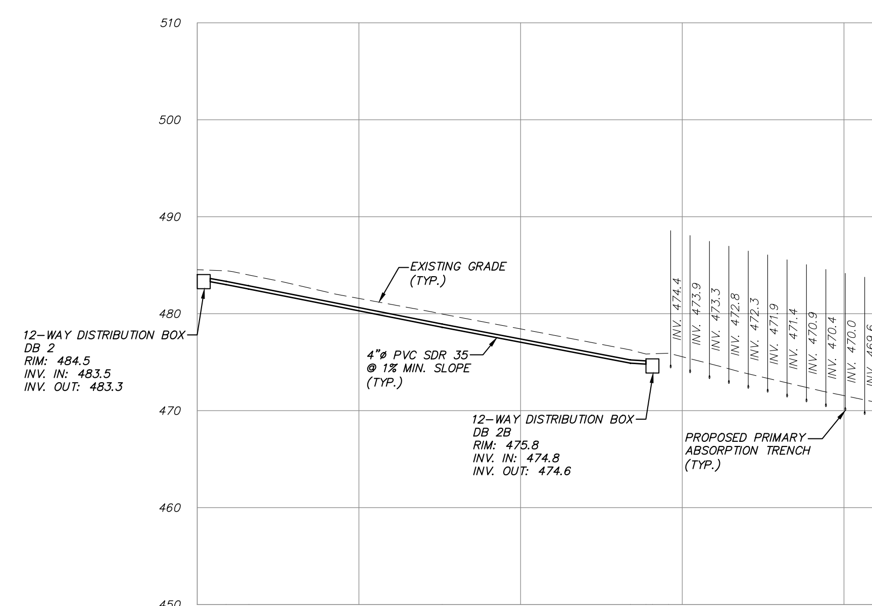
DISTRIBUTION BOX DB 2 TO EXPANSION SSTS SECTION 2B PROFILE
