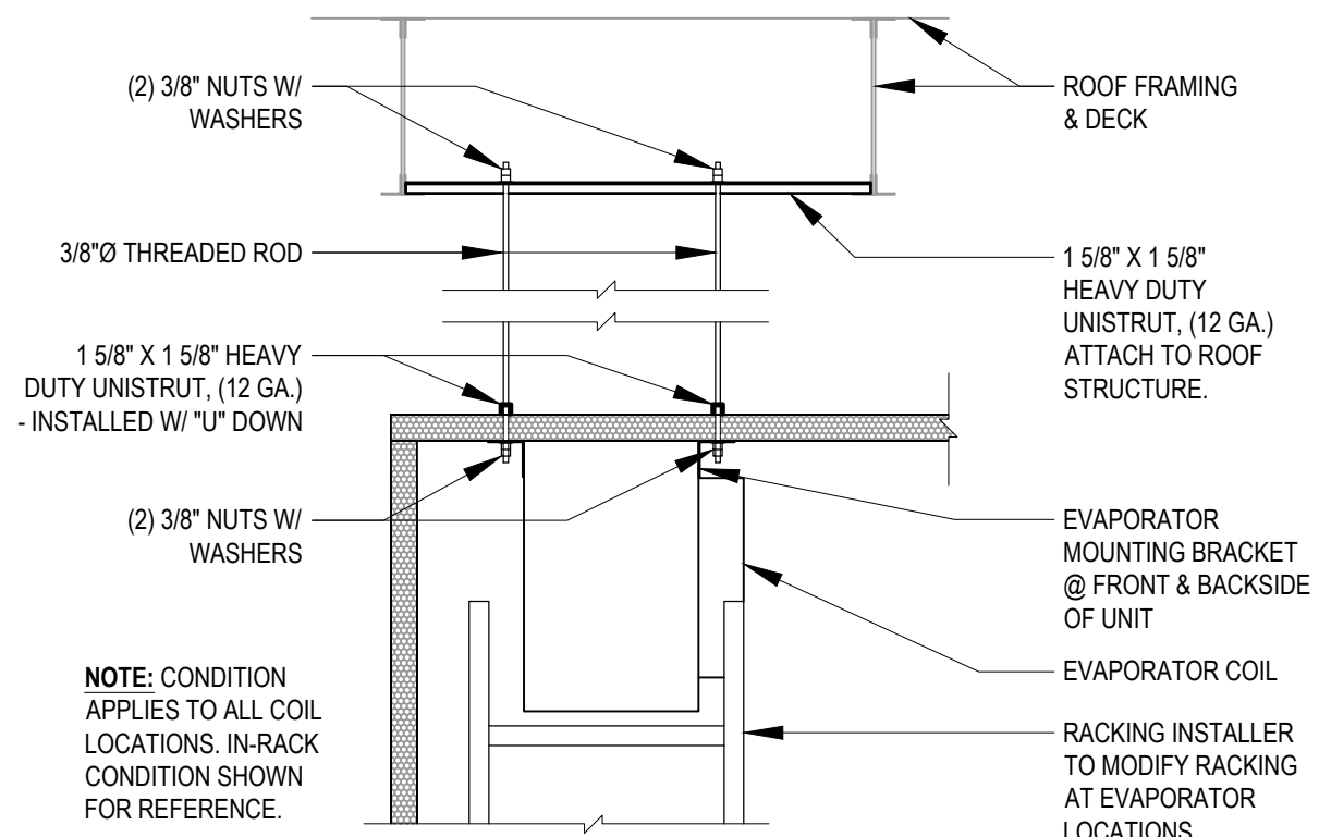
M ROOF SUPPORTED EVAPORATOR COIL CONNECTION DETAIL SCALE: N.T.S.
