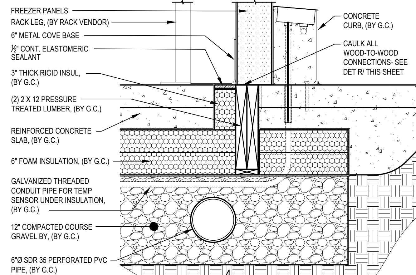
H FREEZER CURB DETAIL SCALE: 1-1/2" = 1'-0"
