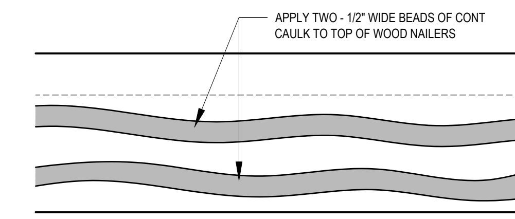
R FREEZER WOOD TO WOOD CONNECTION PLAN VIEW SCALE: N.T.S.
