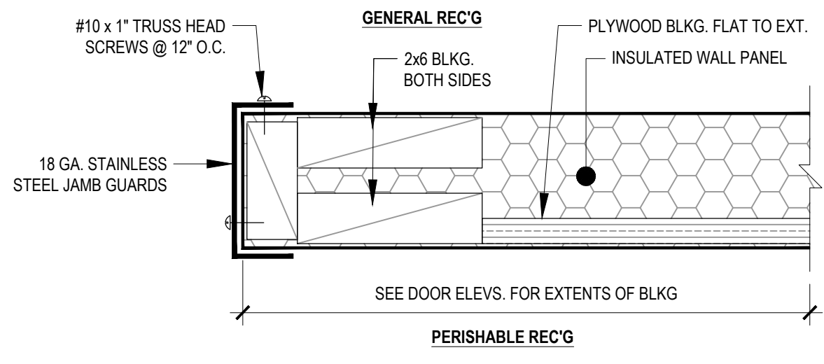
B1 PERISHABLE RECEIVING DOOR JAMB DETAIL SCALE: N.T.S.
