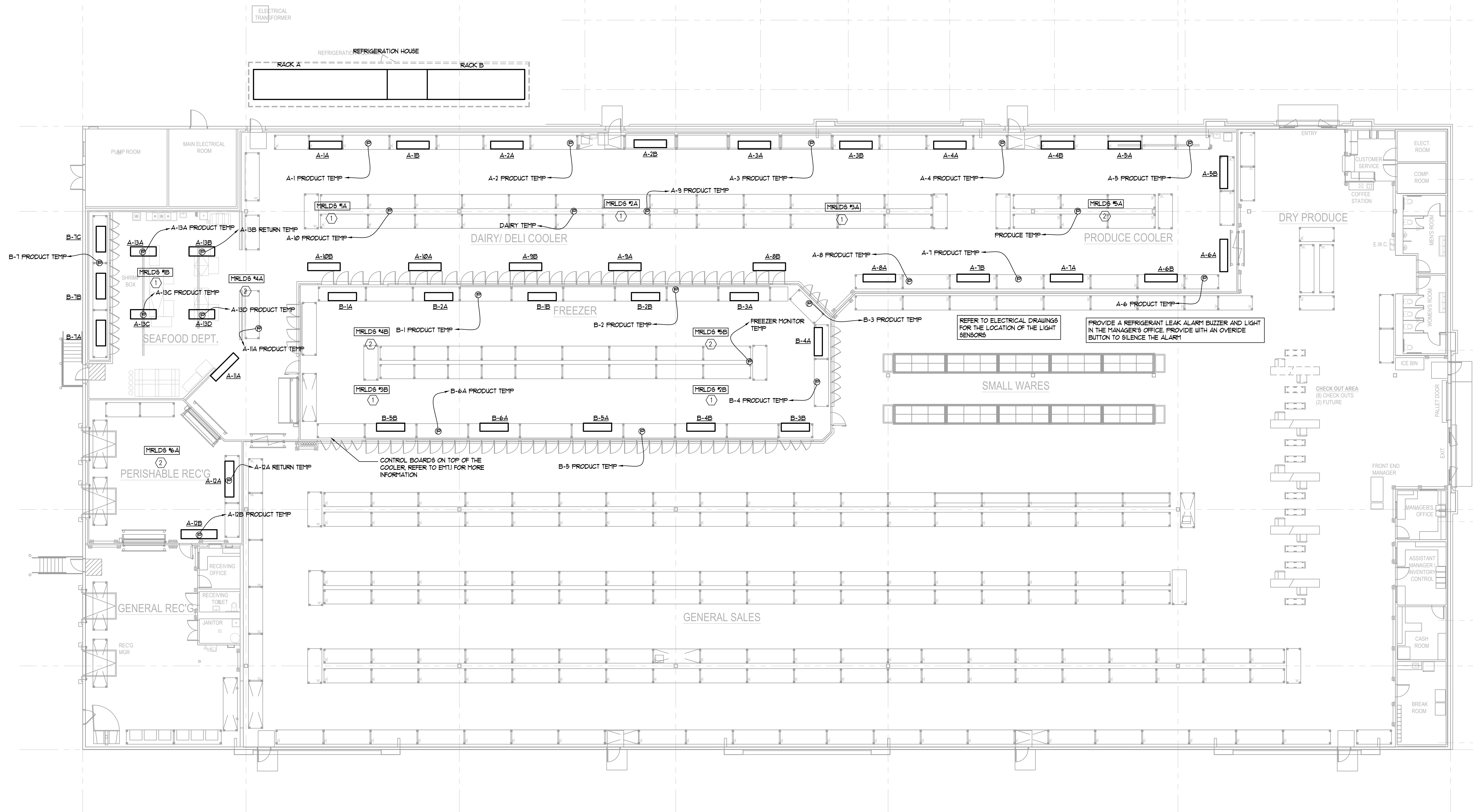
1 FLOOR PLAN – REFRIGERATION SENSOR LOCATIONS R1.2 3/32" = 1'-0"
