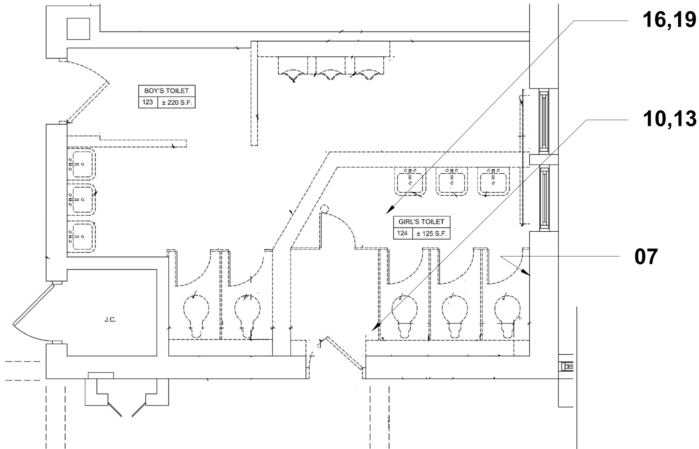
1 123 BOYS AND 124 GIRLS TOILET PLAN - FIRST FLOOR BSL001 SCALE: NOT TO SCALE
