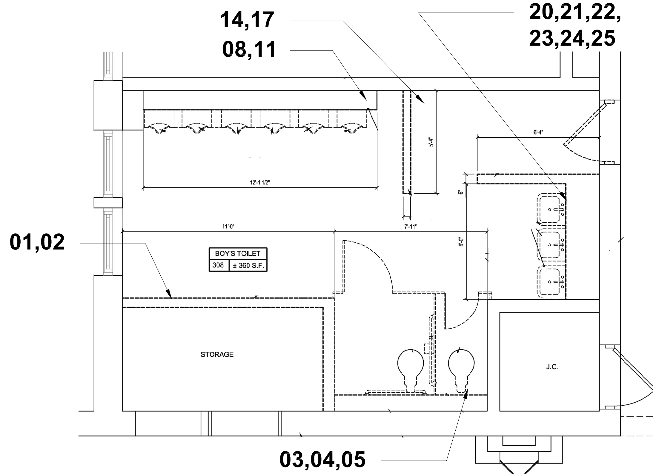
2 308 BOYS TOILET PLAN - THIRD FLOOR BSL001 SCALE: NOT TO SCALE
