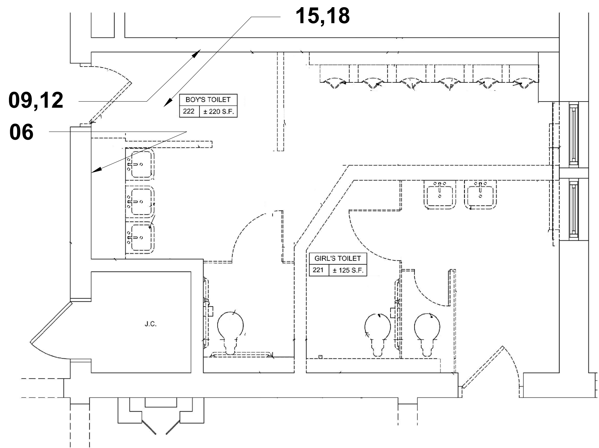
3 221 GIRLS AND 222 BOYS TOILET PLAN - SECOND FLOOR BSL001 SCALE: NOT TO SCALE
