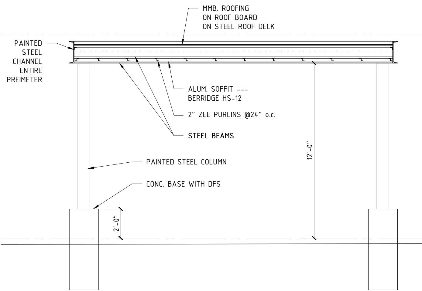
11 PORTE-COCHERE SECTION A202 1/4" = 1'-0"
