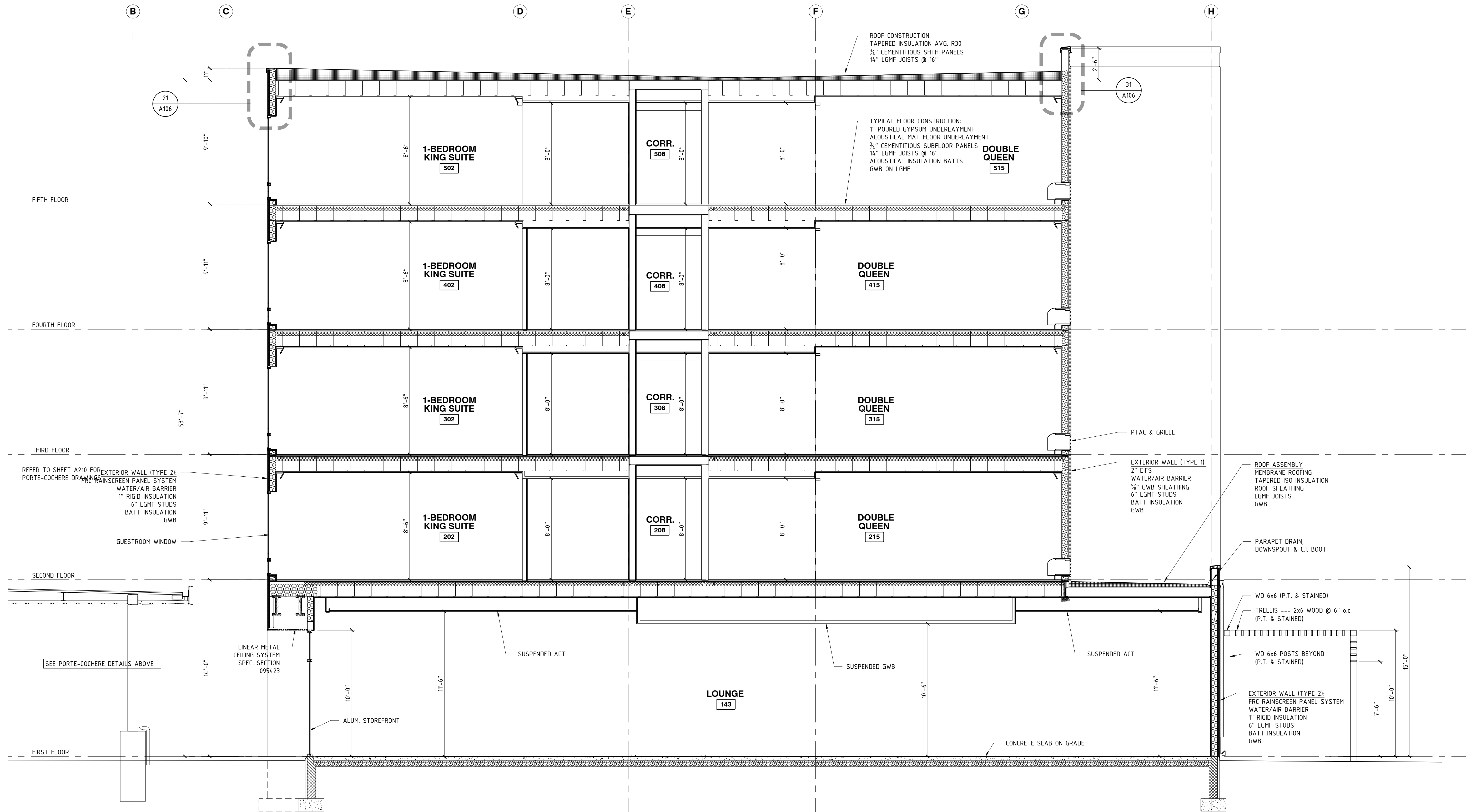
14 BUILDING SECTION A202 1/4" = 1'-0"
