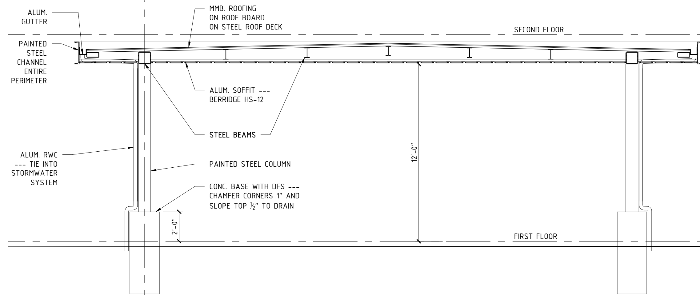
21 PORTE-COCHERE SECTION A202 1/4" = 1'-0"
