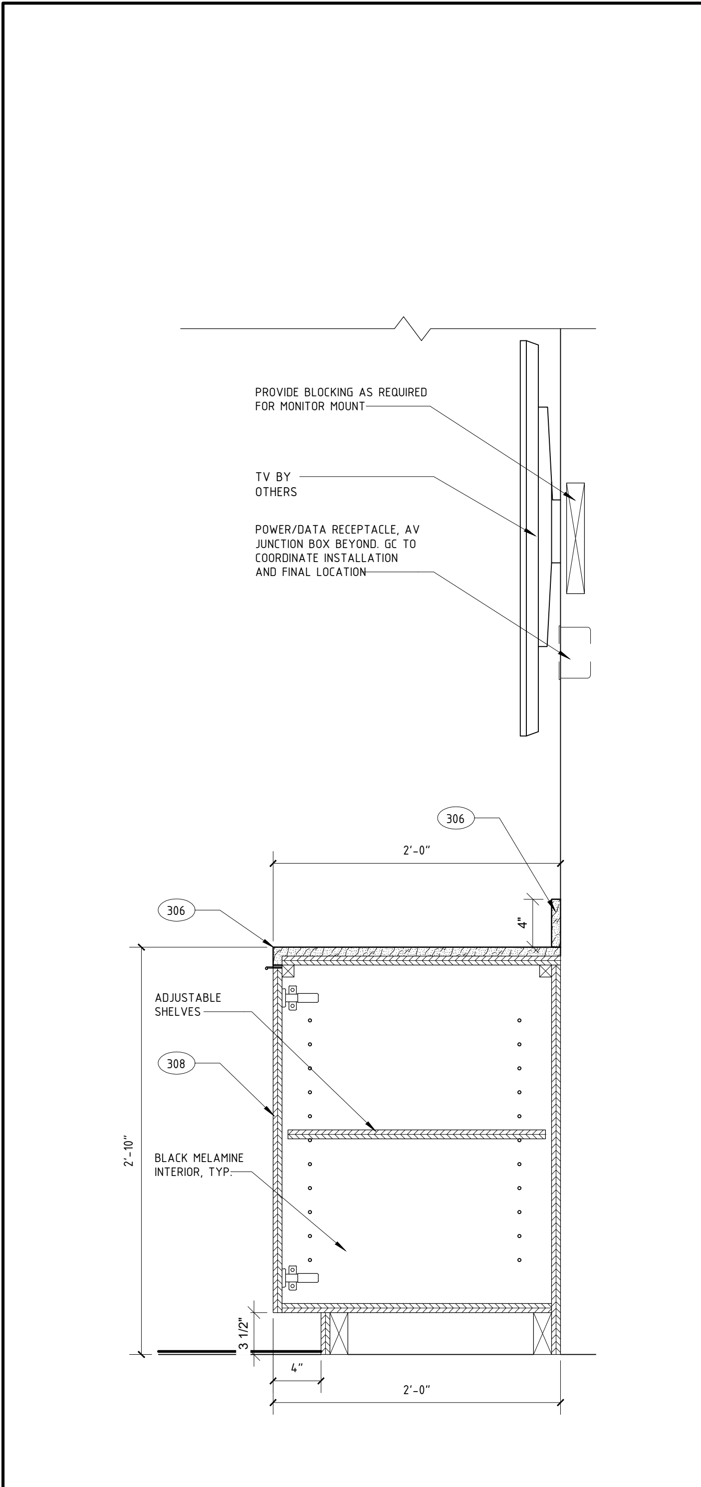
13 TV & CASEWORK @ COLLABORATION A512 SCALE: 1 1/2" = 1'-0"
