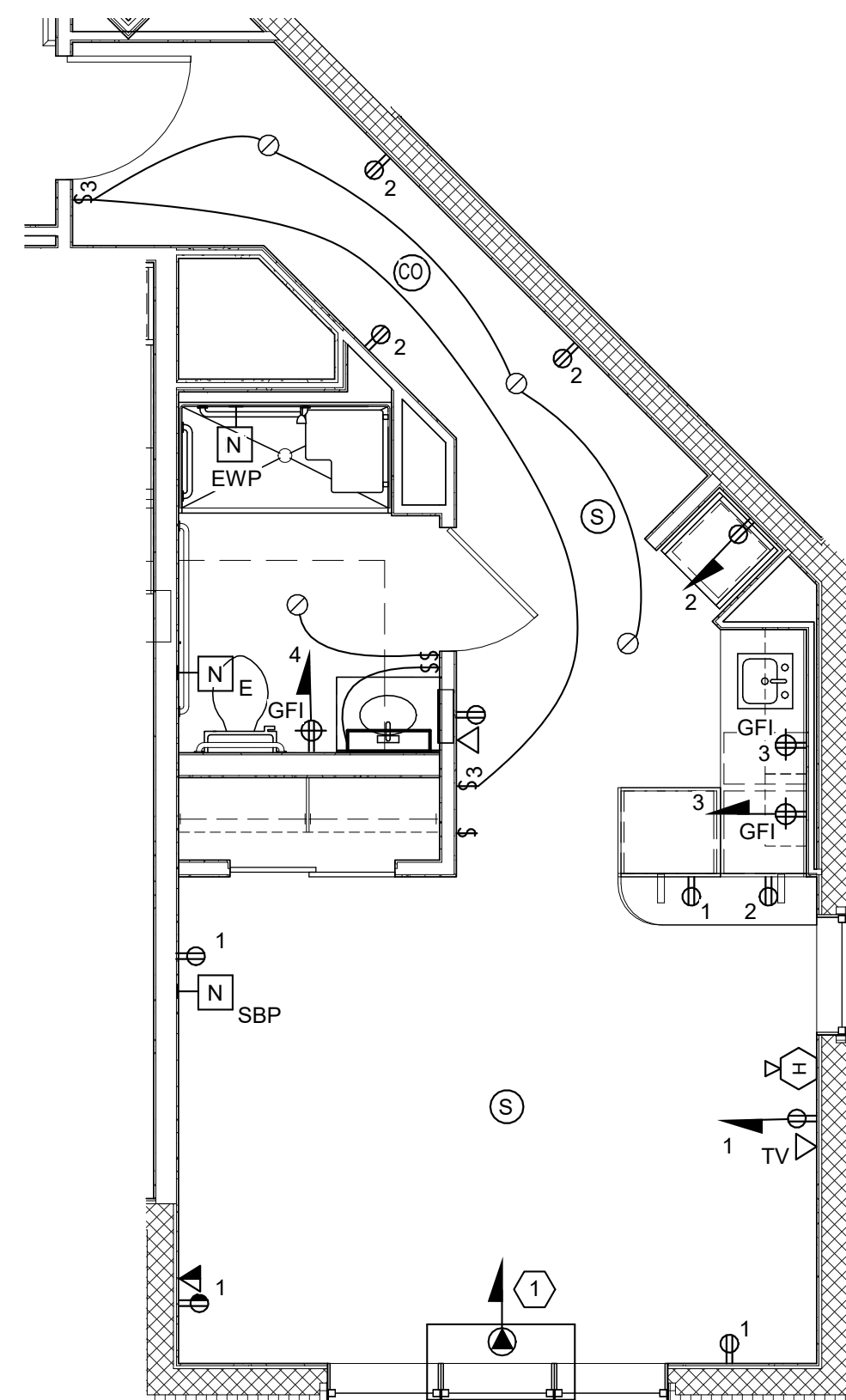
6 TYPICAL TYPE 6 - PRIVATE ELECTRICAL & FIRE ALARM PLAN SCALE: 1/4" = 1'-0"
