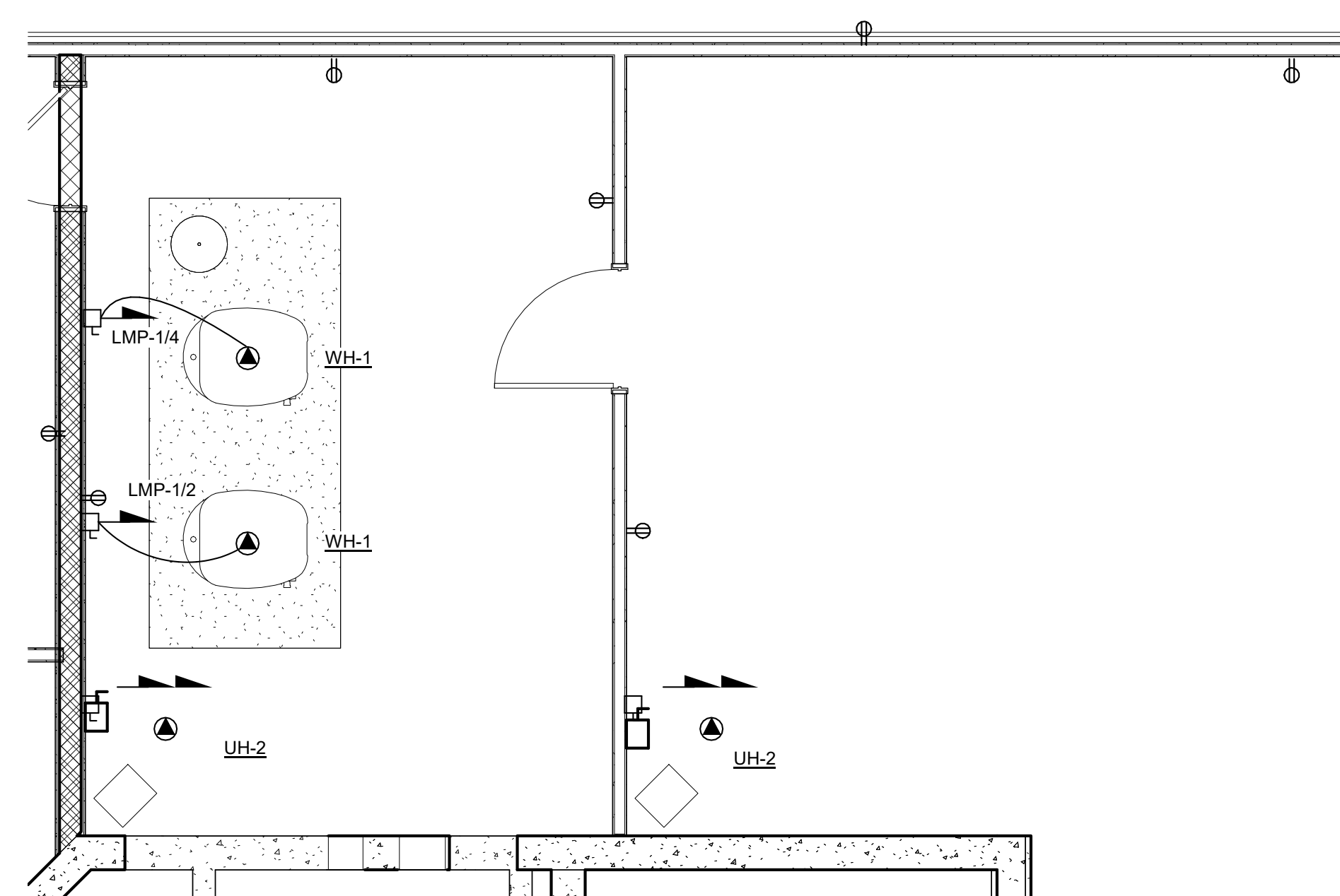
2 ENLARGED BOILER ROOM POWER PLAN SCALE: 1/4" = 1'-0"
