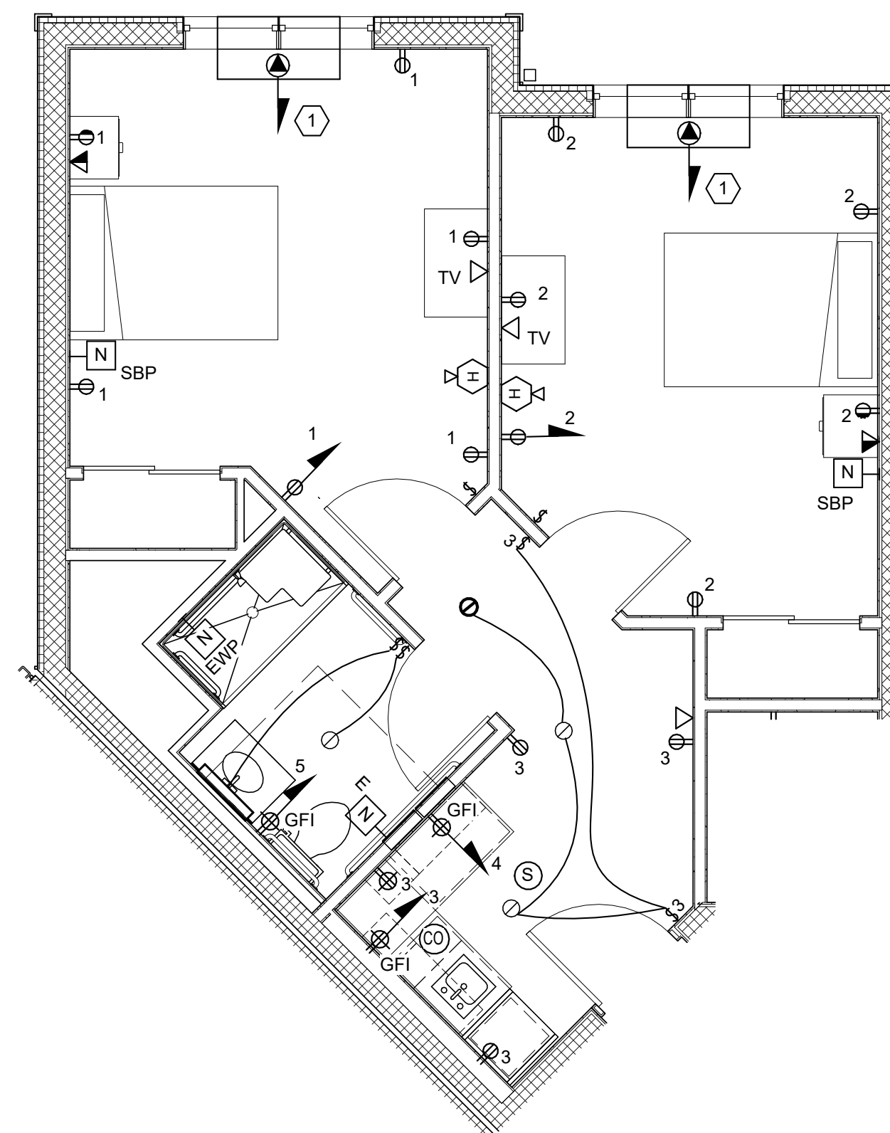
7 TYPICAL TYPE 7 - SEMI-PRIVATE ELECTRICAL & FIRE ALARM PLAN SCALE: 1/4" = 1'-0"
