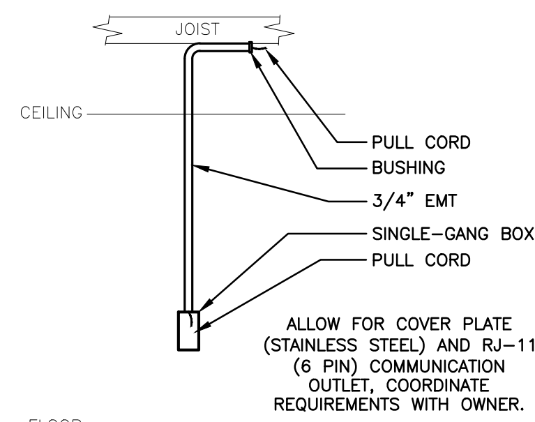
6 COMMUNICATION DETAIL N.T.S.
