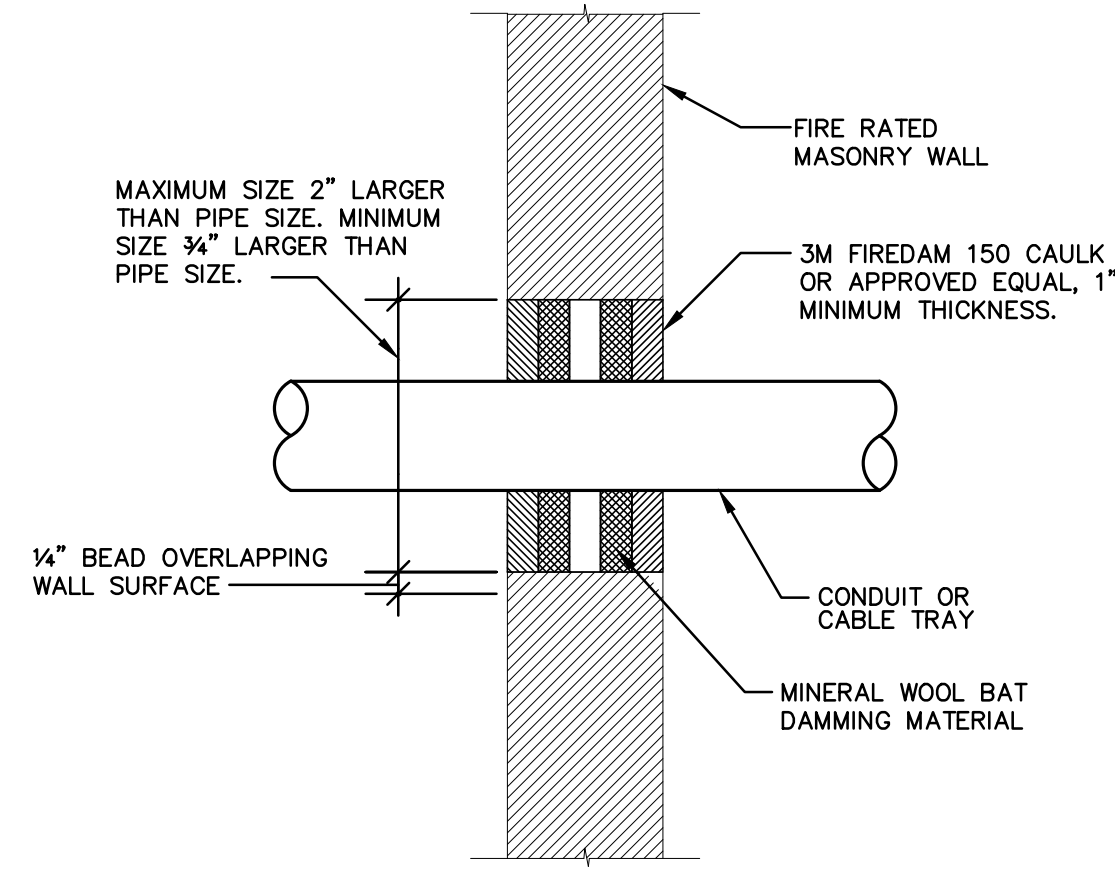
3 CONDUIT PENETRATION IN FIRE RATED MASONRY PARTITION N.T.S.
