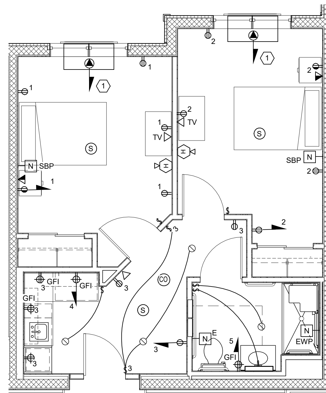
3 TYPICAL TYPE 3 & 3A - SEMI-PRIVATE ELECTRICAL & FIRE ALARM PLAN SCALE: 1/4" = 1'-0"
