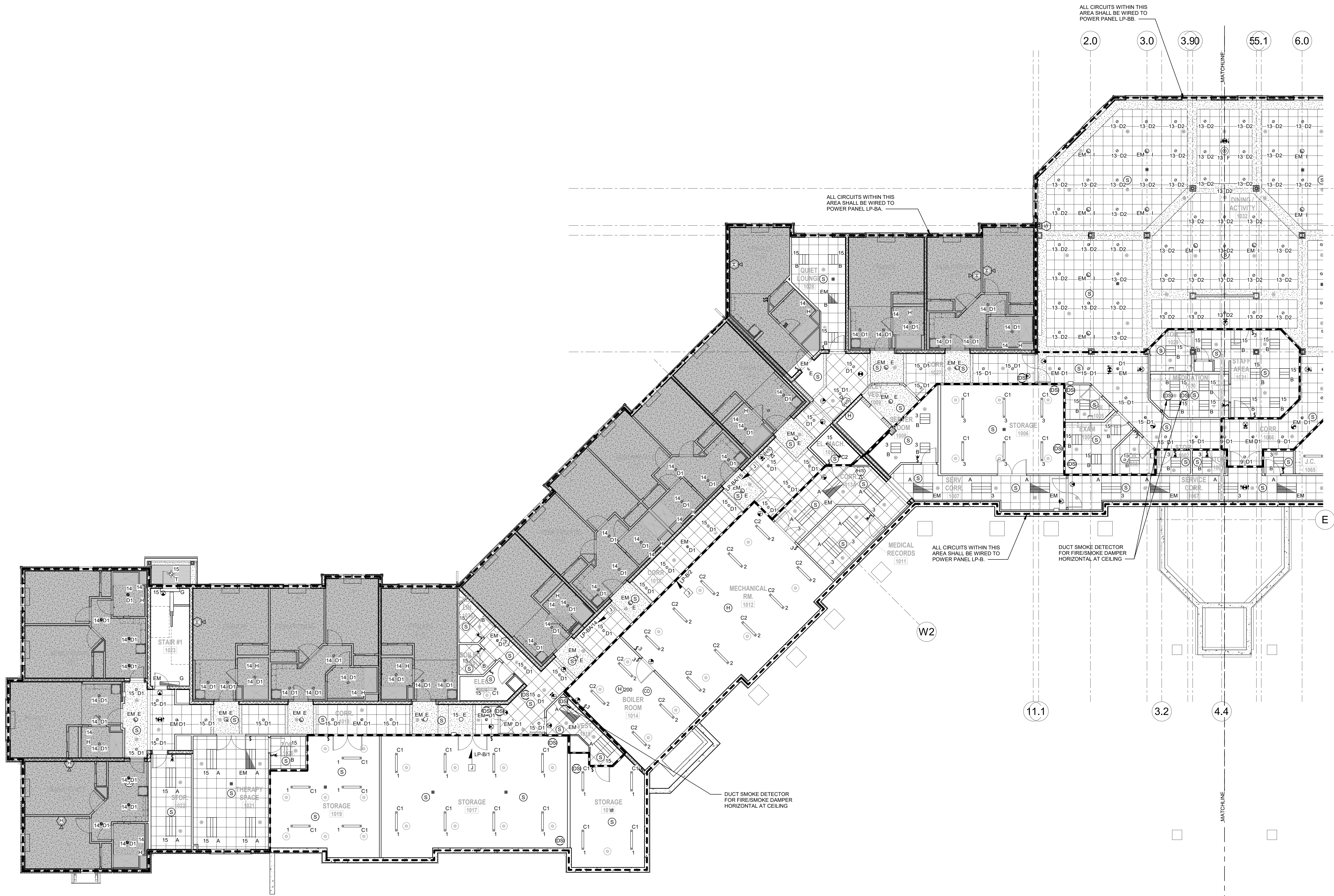
1 ELECTRICAL BASEMENT FLOOR LIGHTING PLAN - AREA A SCALE: 1/8" = 1'-0"
