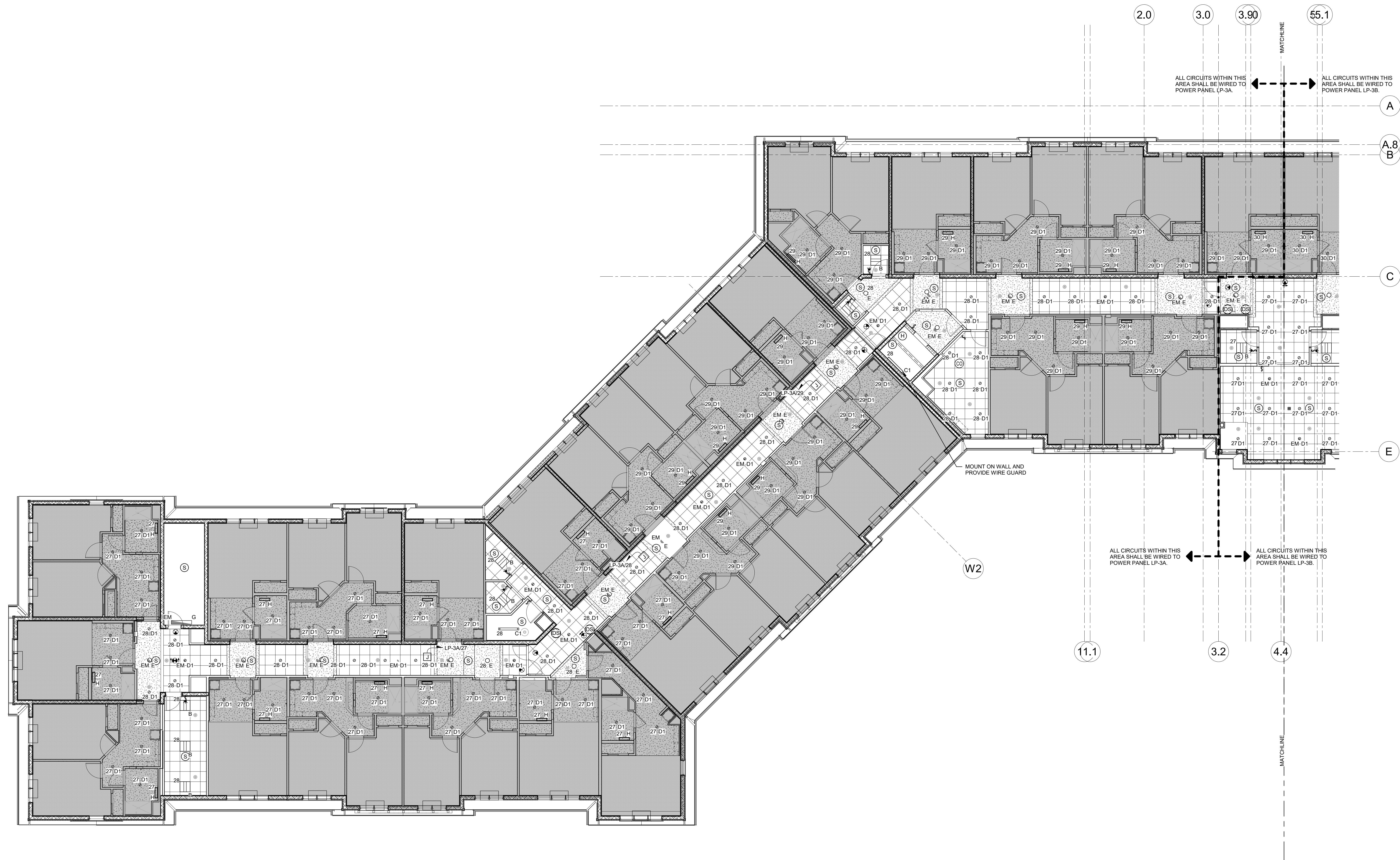
1 ELECTRICAL THIRD FLOOR LIGHTING PLAN - PART A SCALE: 1/8" = 1'-0"
