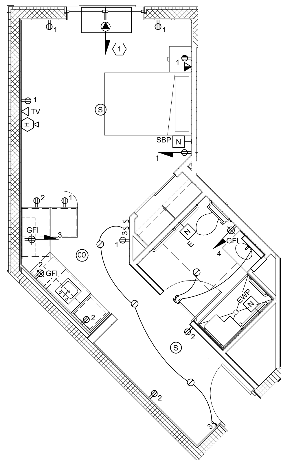
5 TYPICAL TYPE 5 - PRIVATE ELECTRICAL & FIRE ALARM PLAN SCALE: 1/4" = 1'-0"
