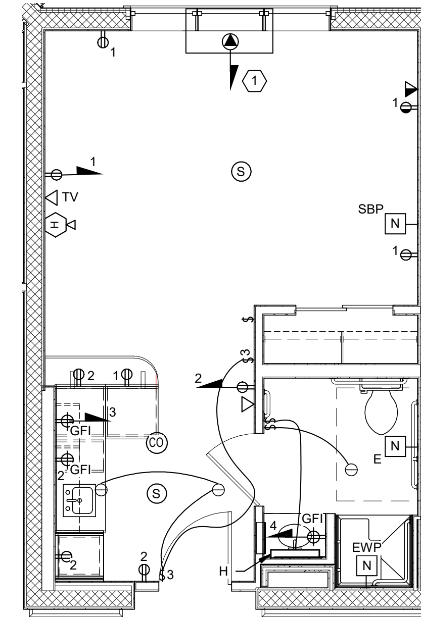
4 TYPICAL TYPE 4 - PRIVATE ELECTRICAL & FIRE ALARM PLAN SCALE: 1/4" = 1'-0"
