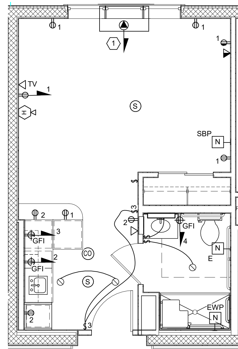
2 TYPICAL TYPE 2 - PRIVATE ELECTRICAL & FIRE ALARM PLAN SCALE: 1/4" = 1'-0"
