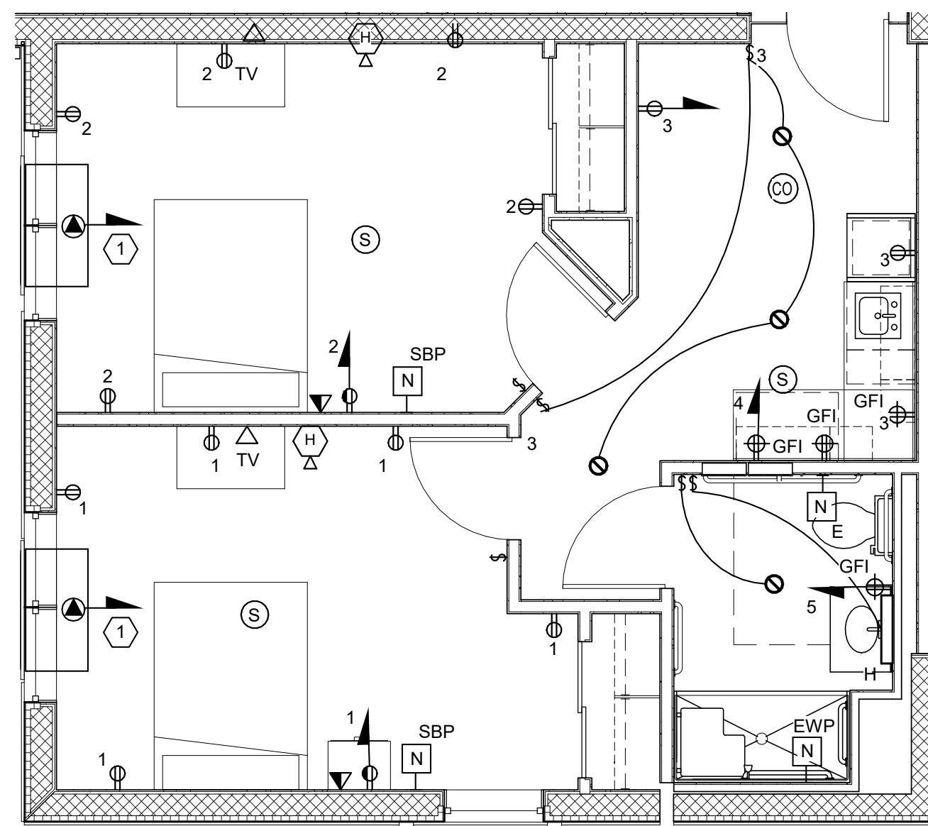
1 TYPICAL TYPE 1 - SEMI-PRIVATE ELECTRICAL & FIRE ALARM PLAN SCALE: 1/4" = 1'-0"
