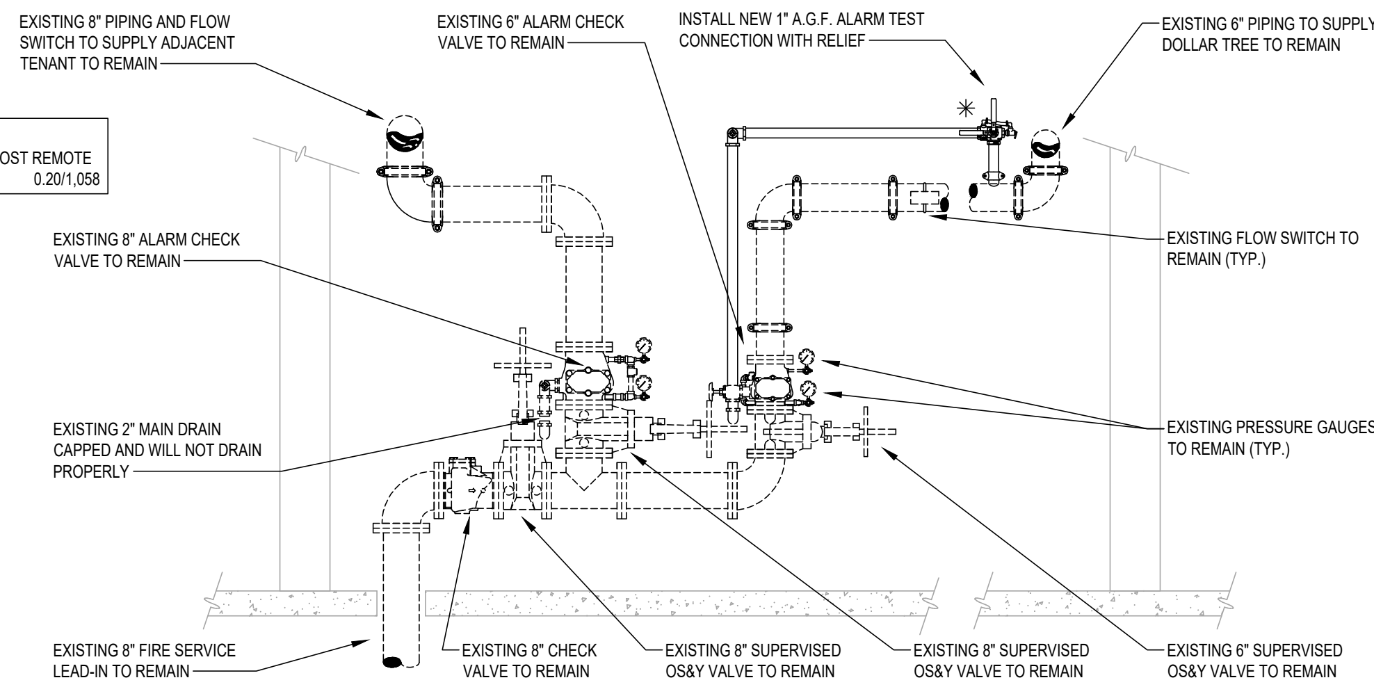
ELEVATION AT EXISTING BUILDING FIRE SPRINKLER RISER (FOR REFERENCE ONLY)
