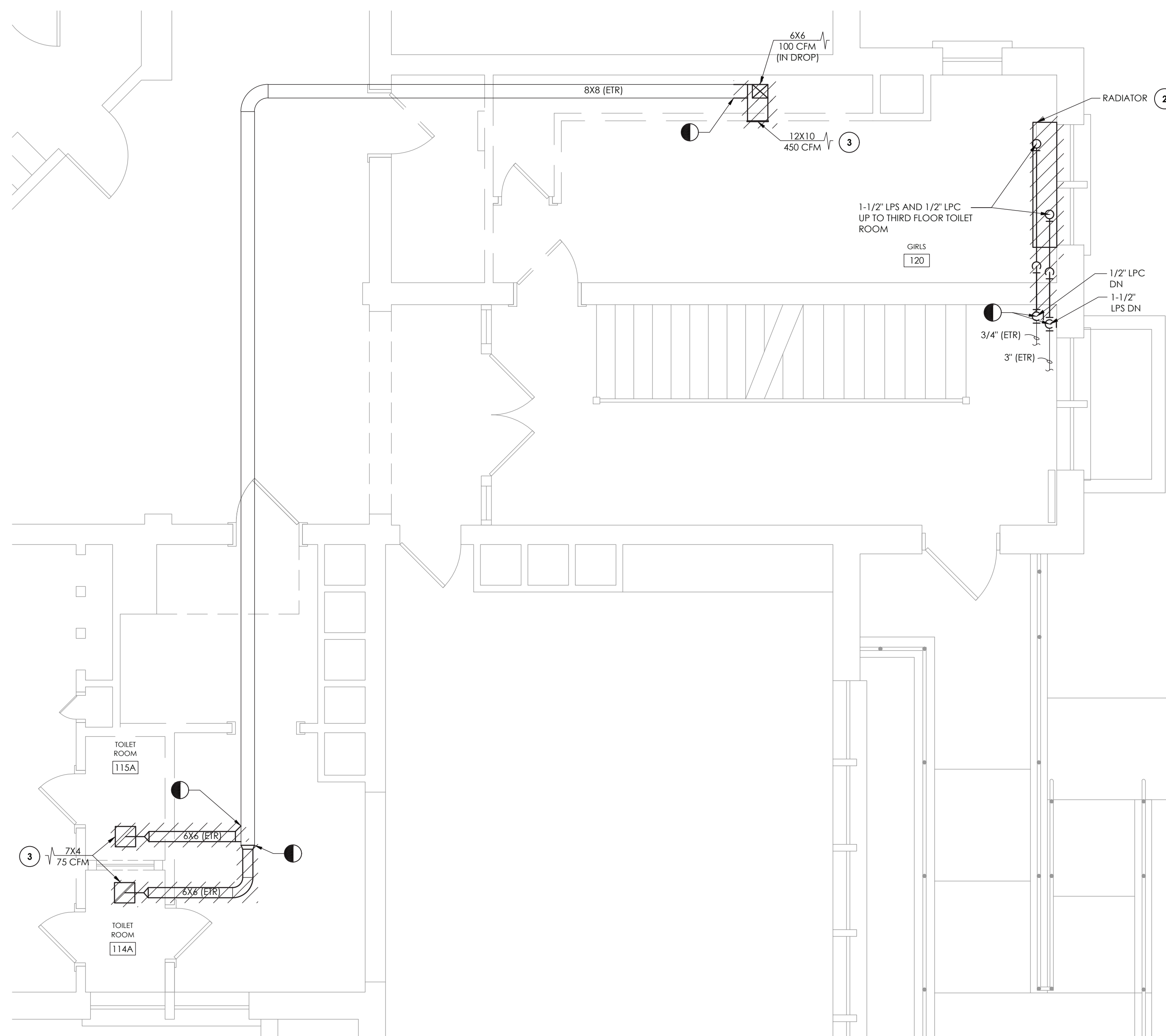
2 TOILET ROOM 120 DEMOLITION PLAN H101 SCALE: 1/4" = 1'-0"
