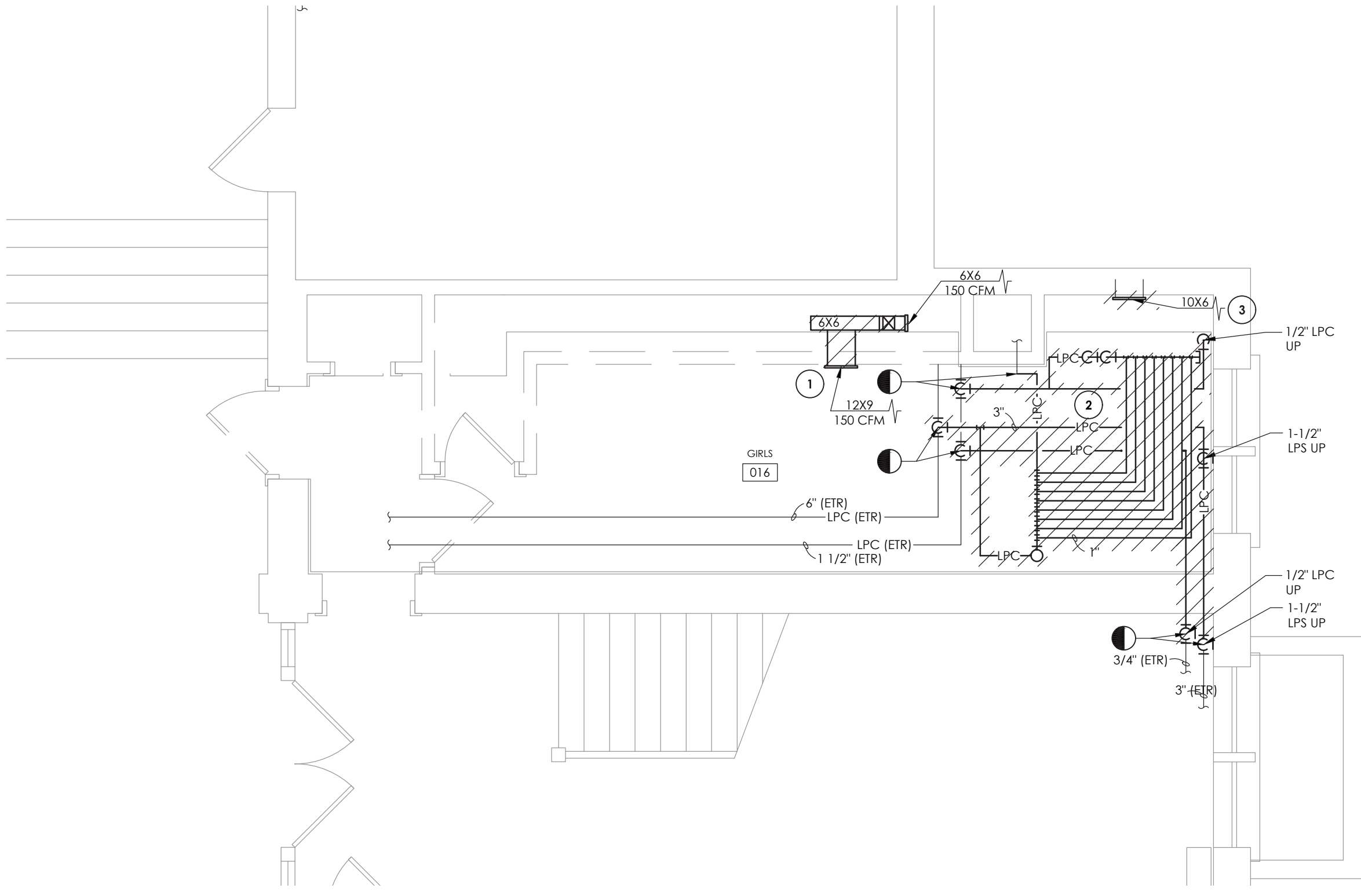
2 H100A TOILET ROOM 016 DEMOLITION SCALE: 1/4" = 1'-0"
