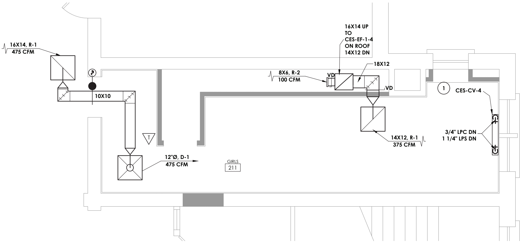
2 H202 TOILET ROOM 211 NEW WORK PLANS SCALE: 1/4" = 1'-0"
