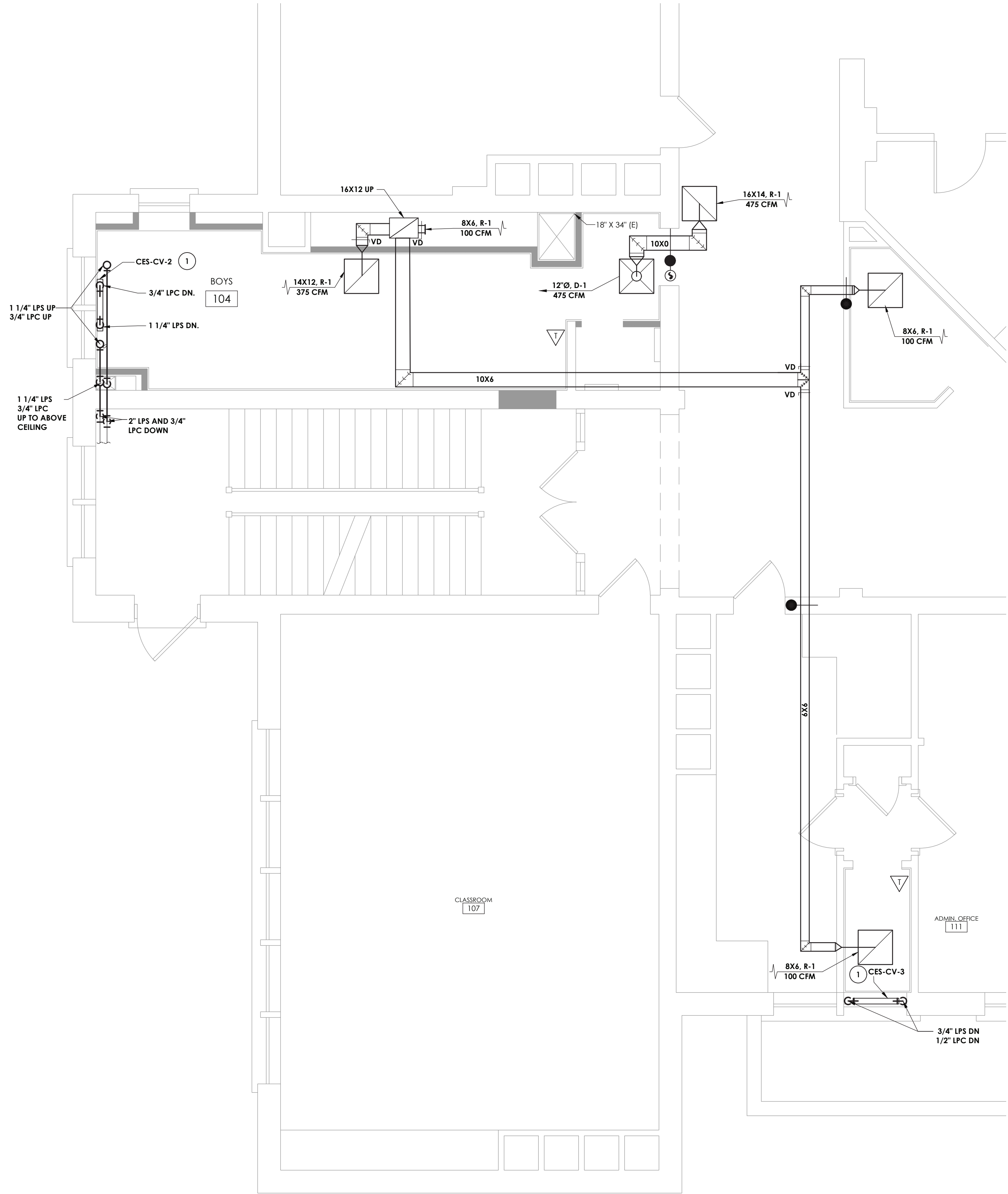
1 TOILET ROOMS 104,111, & 4 NEW WORK PLAN SCALE: 1/4" = 1'-0"
