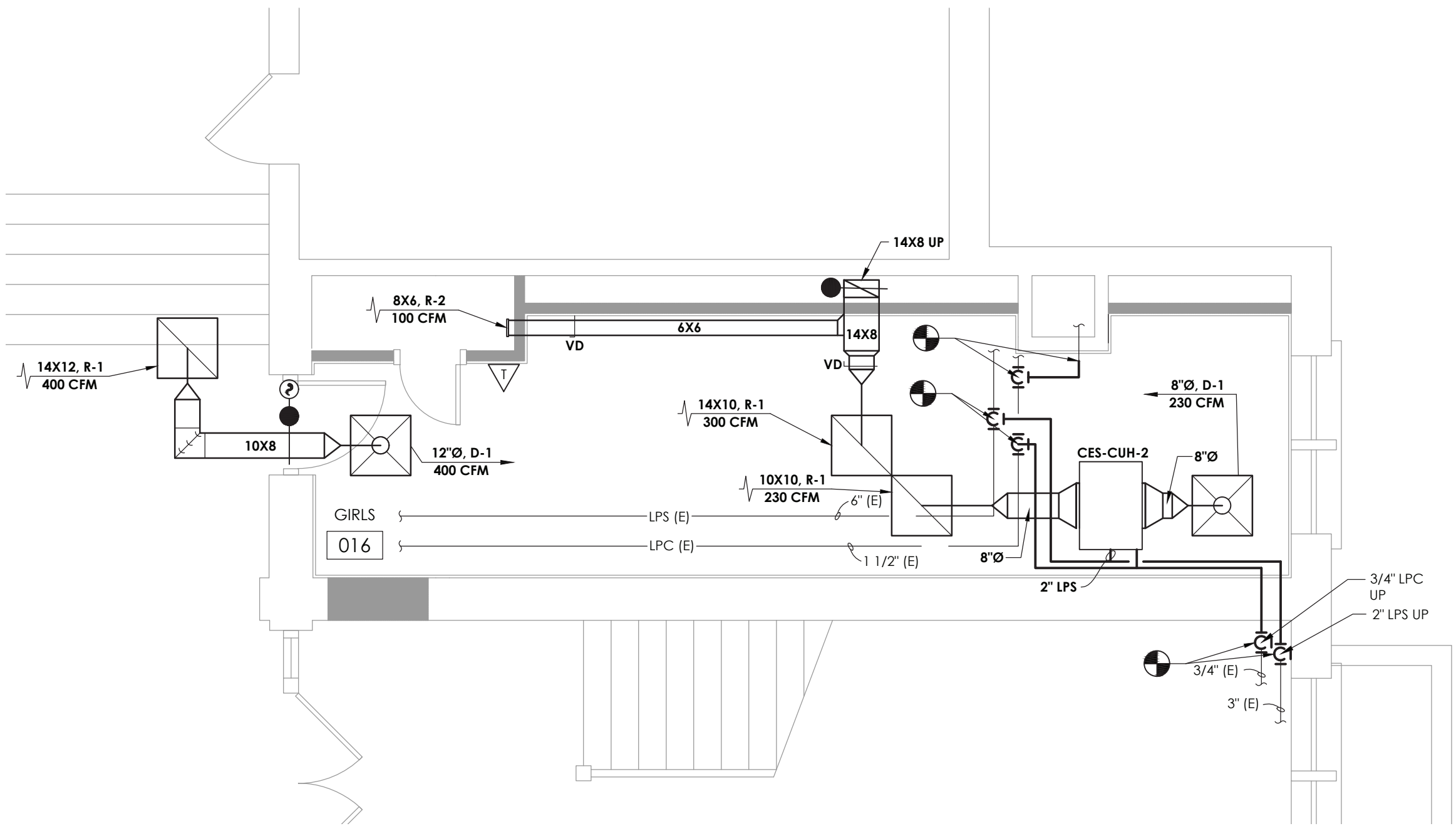
2 H200A TOILET ROOM 16 NEW WORK PLAN SCALE: 1/4" = 1'-0"
