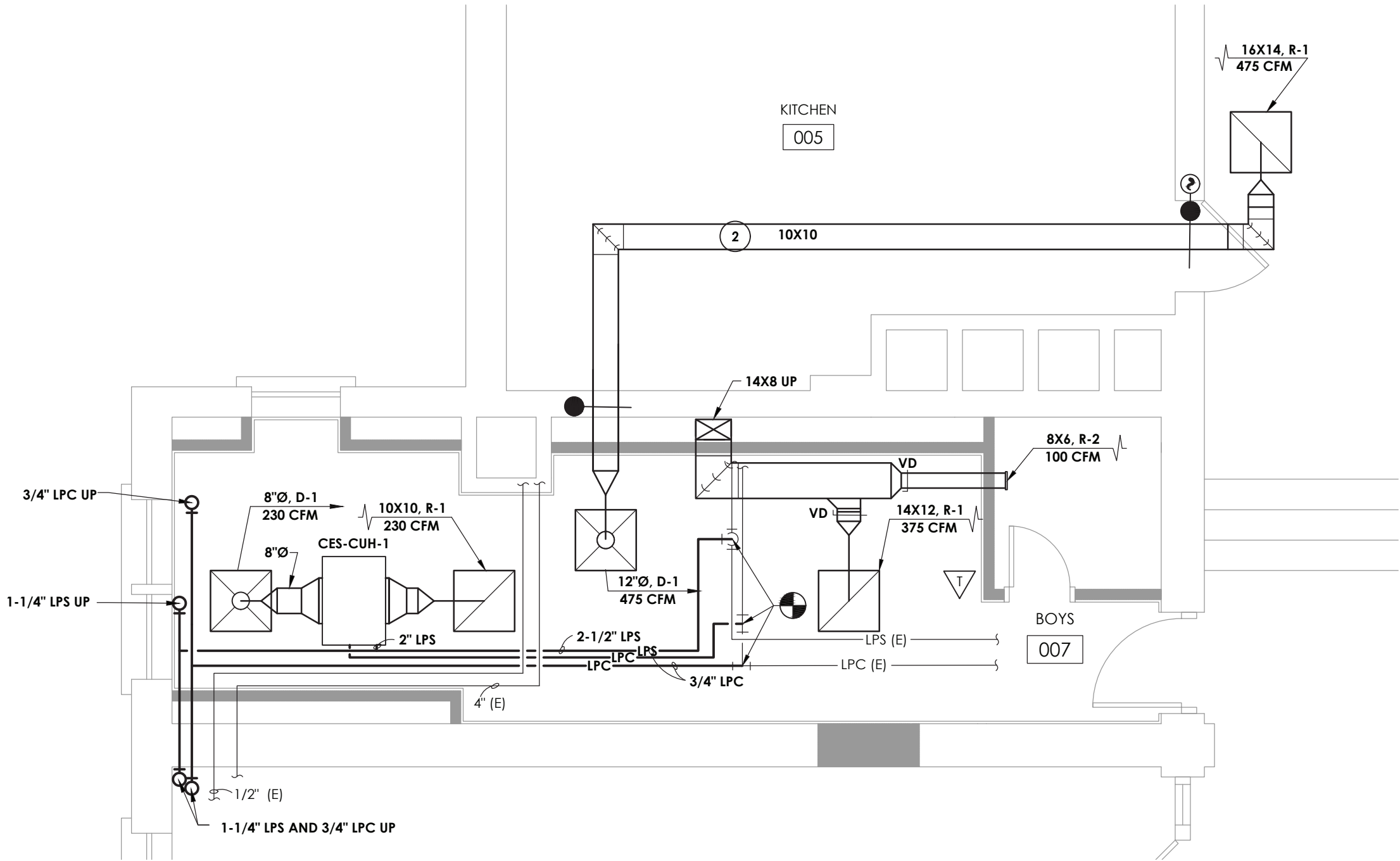
1 H200A TOILET ROOM 007 NEW WORK PLAN SCALE: 1/4" = 1'-0"
