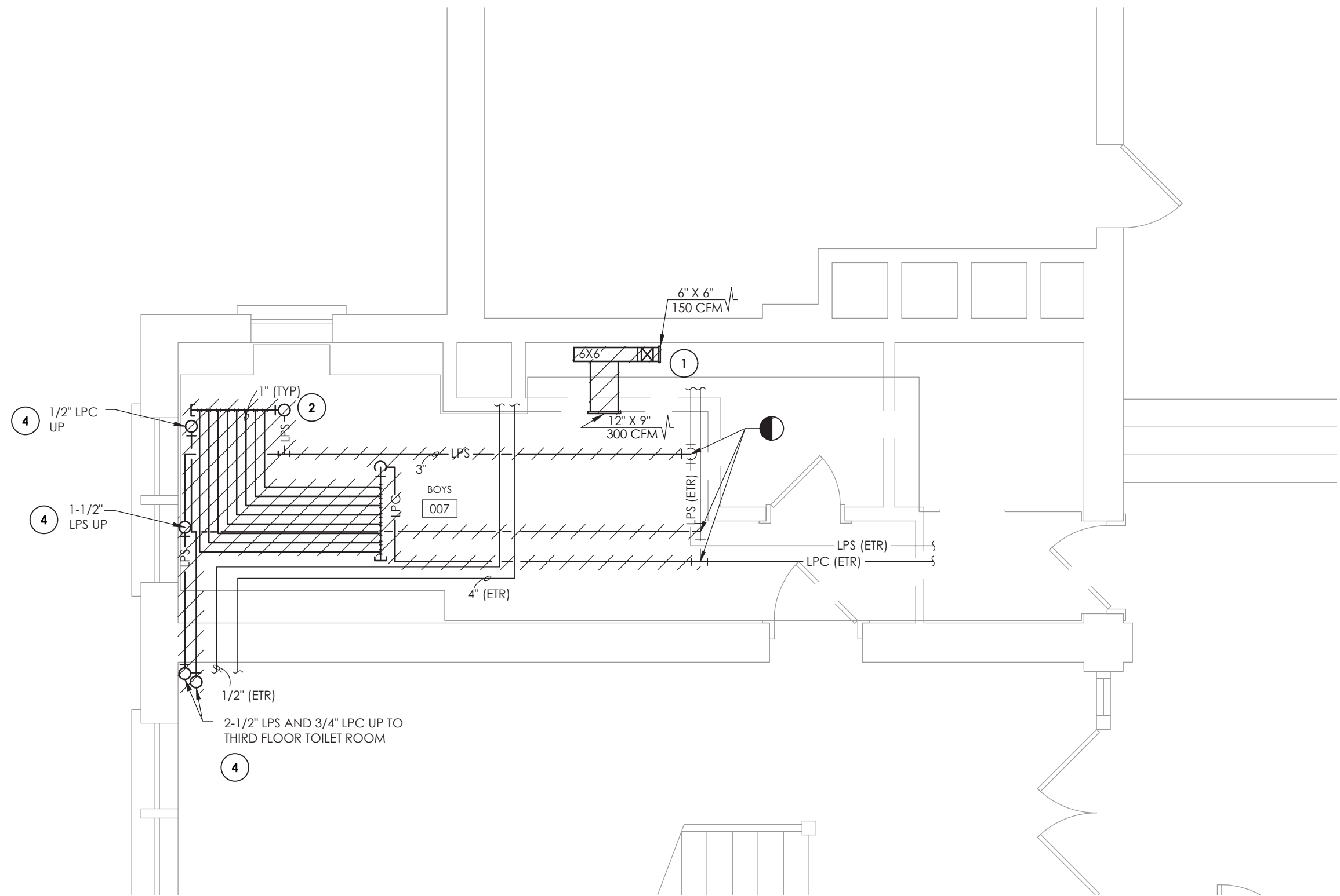
1 H100A TOILET ROOM 007 DEMOLITION SCALE: 1/4" = 1'-0"
