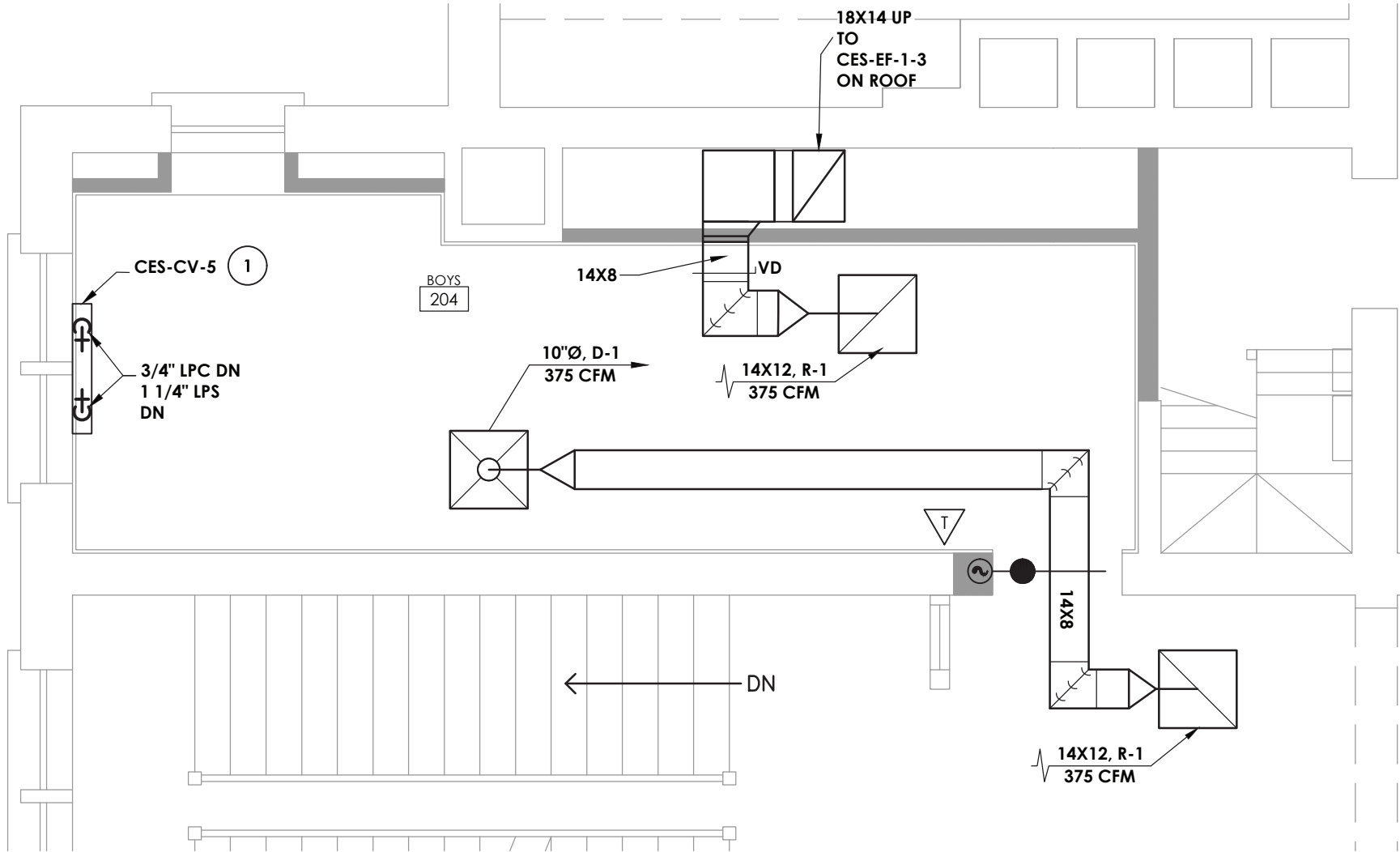
1 H202 TOILET ROOM 204 NEW WORK PLANS SCALE: 1/4" = 1'-0"
