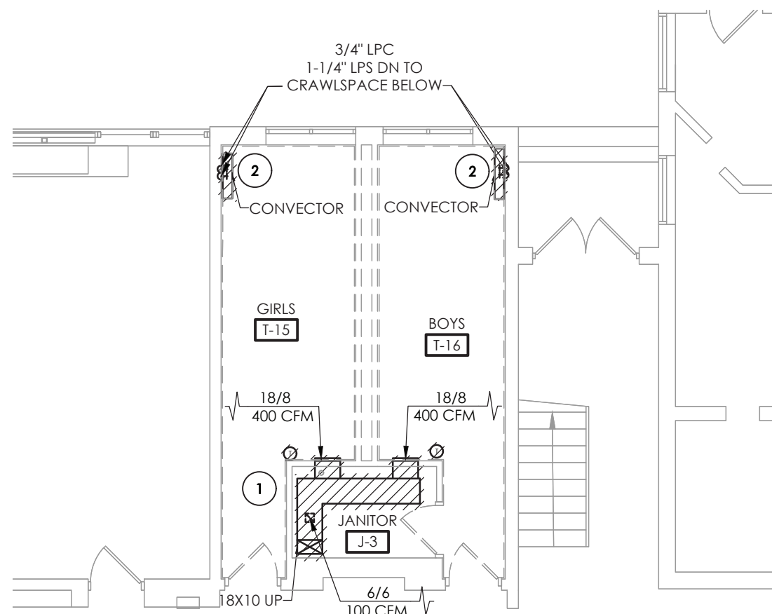
5 H101A TOILET ROOMS T-15 AND T-16 DEMOLITION PLAN SCALE: 1/8" = 1'-0"
