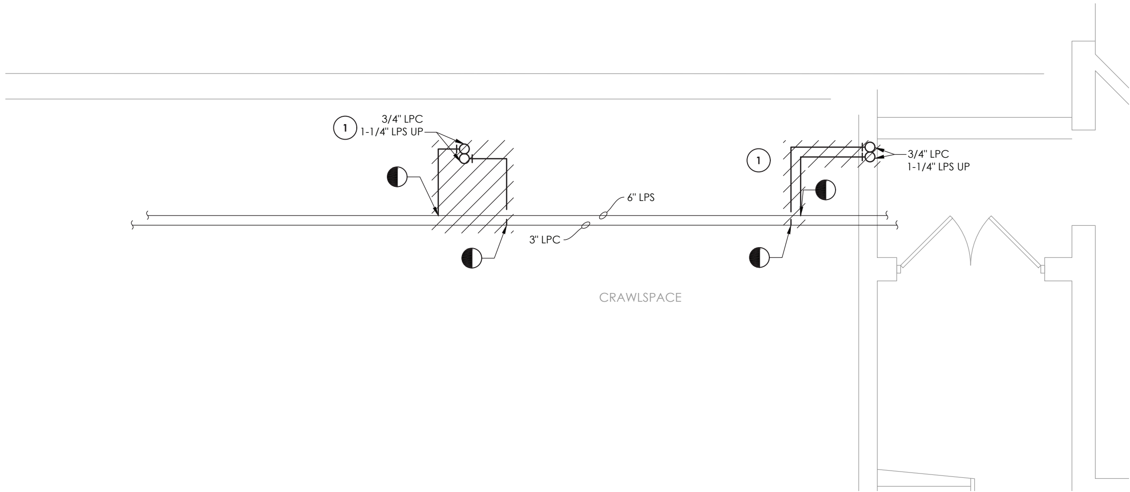
3 CRAWLSPACE BELOW T-15 AND T-16 HVAC DEMOLITION PLAN SCALE: 1/4" = 1'-0"
