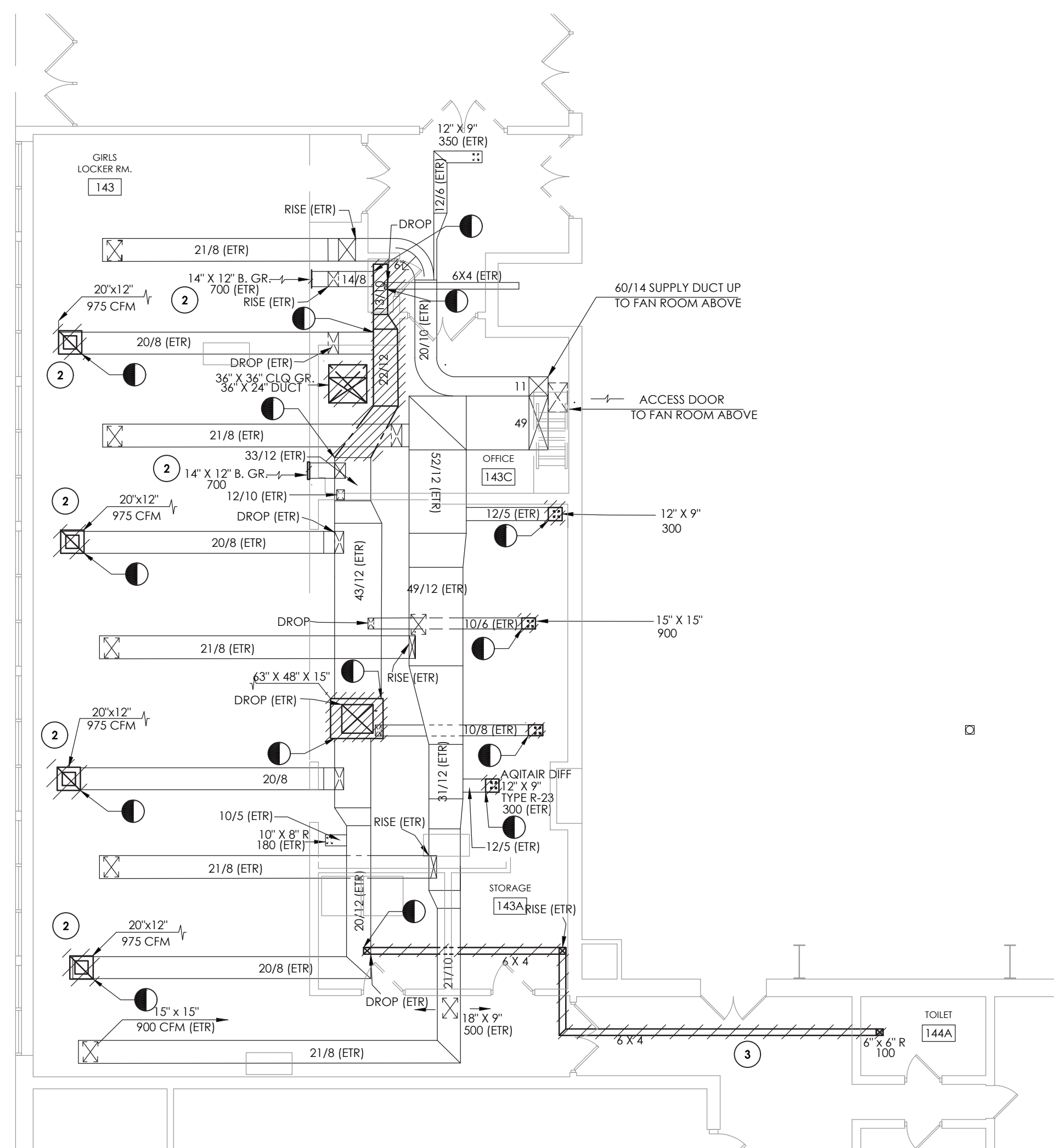
7 H101B GIRLS' LOCKER ROOM HVAC DEMOLITION PLAN SCALE: 1/8" = 1'-0"
