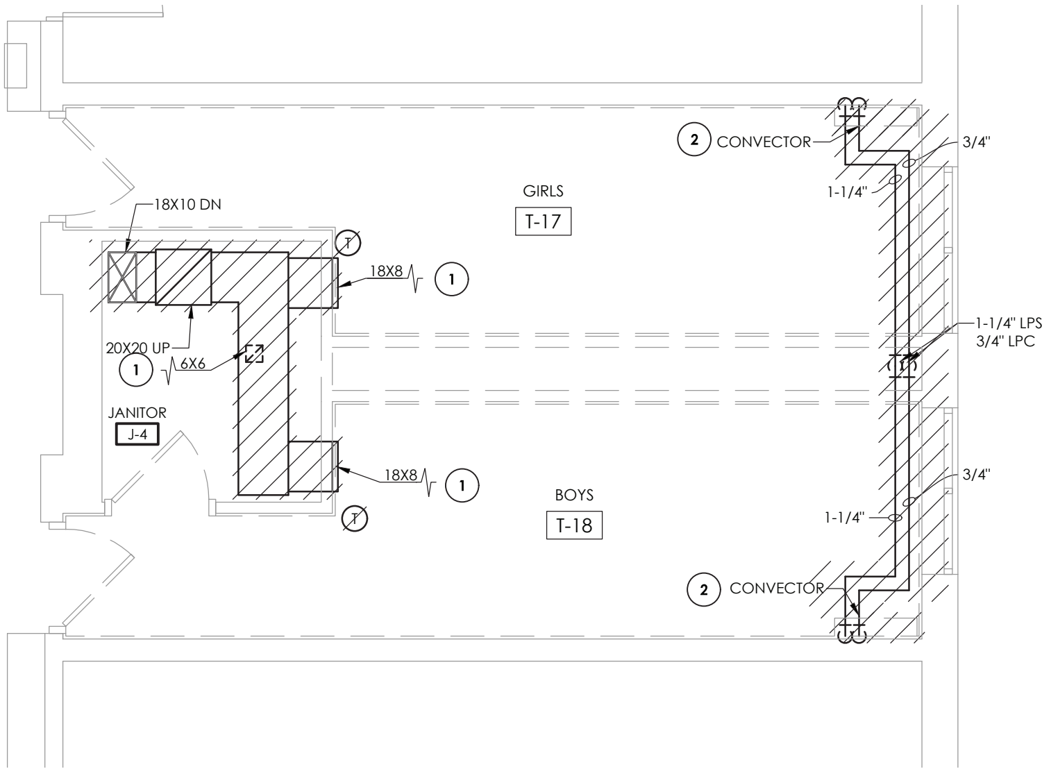
1 H102 TOILET ROOMS T-17 AND T-18 DEMOLITION PLAN SCALE: 1/4" = 1'-0"
