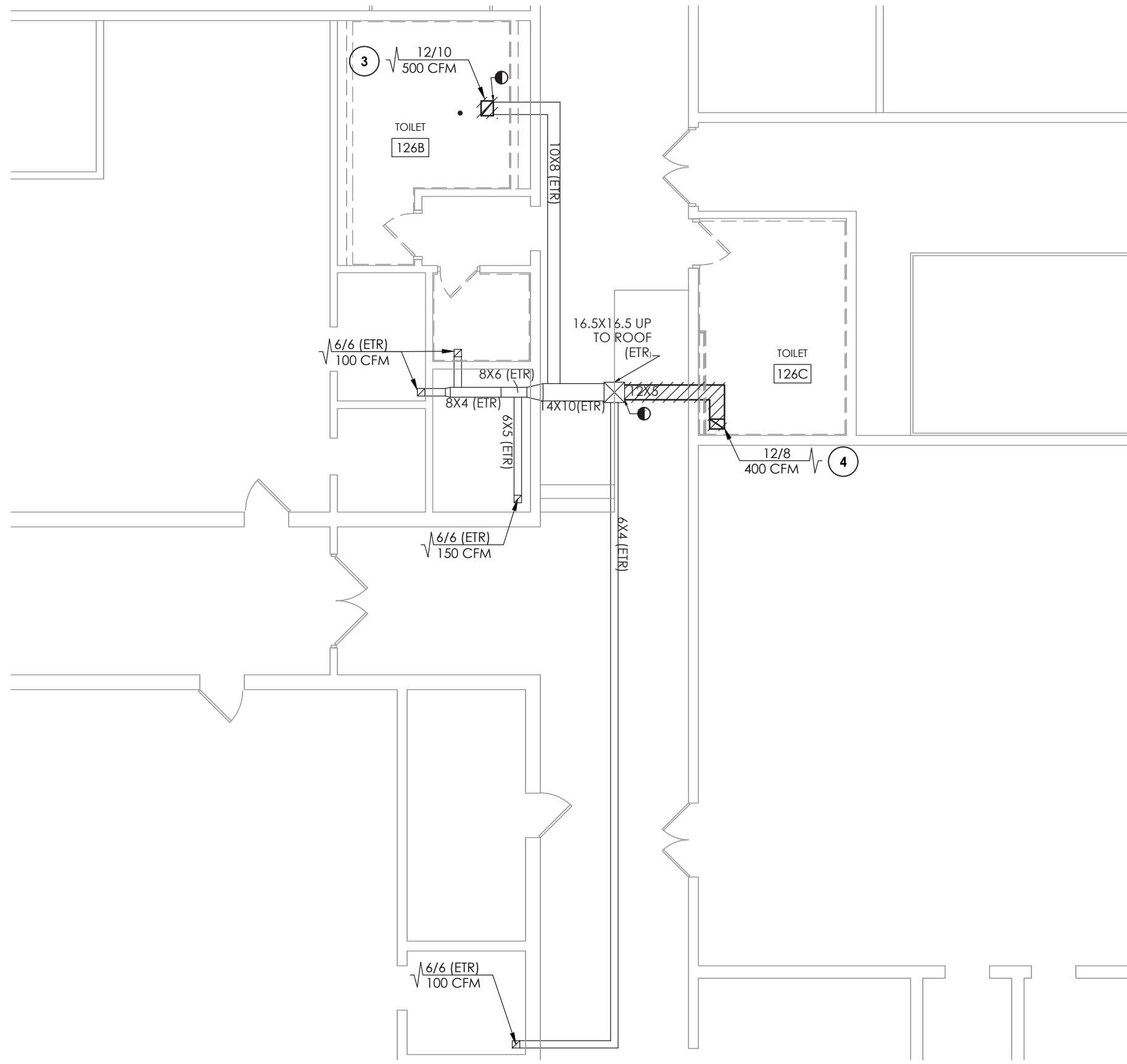
1 H101A TOILET ROOMS T-9 AND T-10 DEMOLITION PLAN SCALE: 1/8" = 1'-0"
