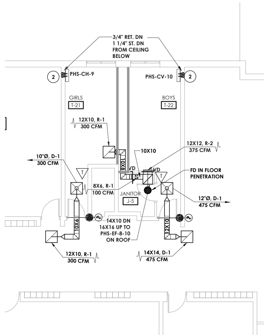
4 H202 SECOND FLOOR TOILET ROOMS T-21 & T-22 HVAC NEW WORK PLAN SCALE: 1/8" = 1'-0"
