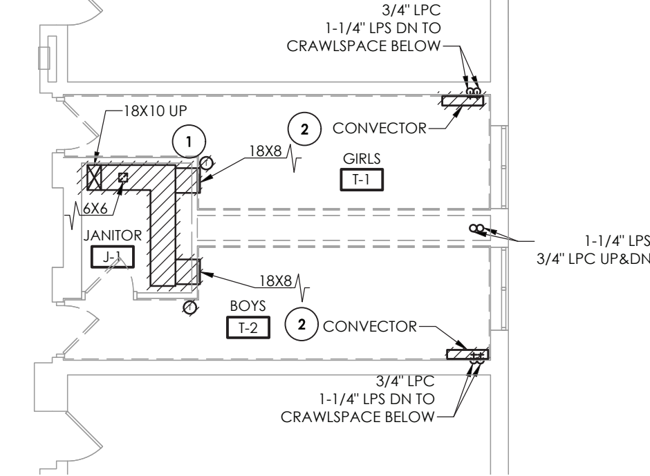
2 H101A TOILET ROOMS T-1 AND T-2 DEMOLITION PLAN SCALE: 1/8" = 1'-0"
