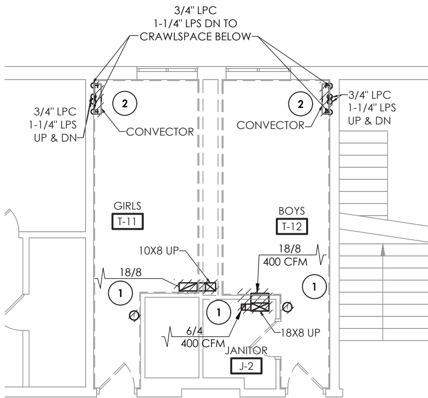
3 H101A TOILET ROOMS T-11 AND T-12 DEMOLITION PLAN SCALE: 1/8" = 1'-0"
