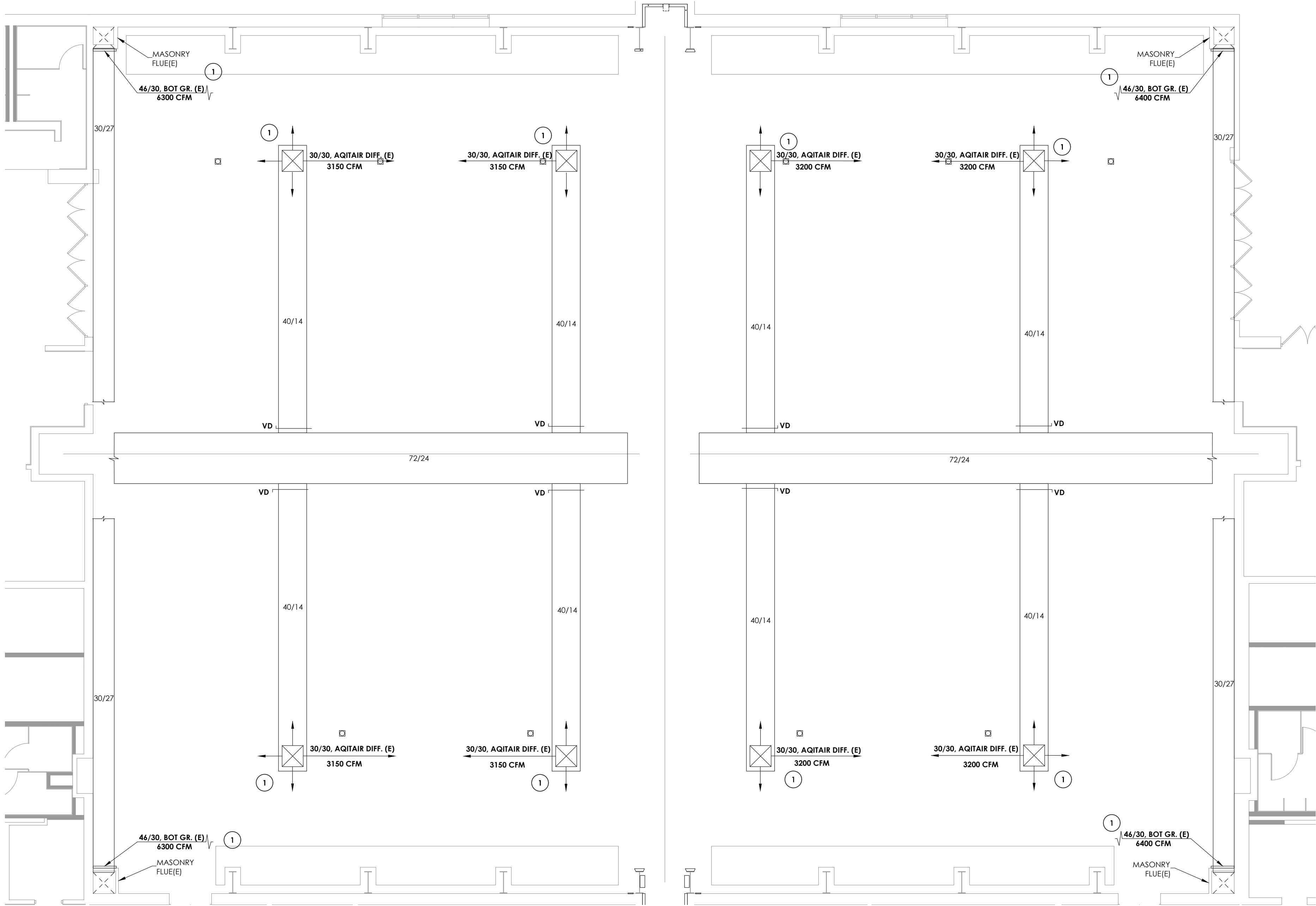
1 H201C GYM HVAC NEW WORK PLAN SCALE: 1/8" = 1'-0"
