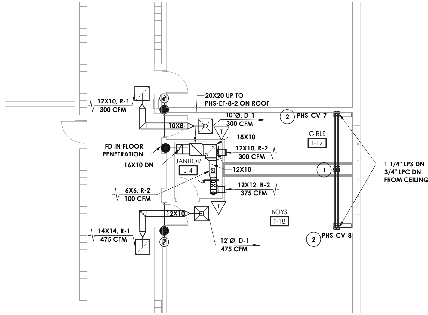
1 H202 SECOND FLOOR TOILET ROOMS T-17 & T-18 HVAC NEW WORK PLAN SCALE: 1/8" = 1'-0"
