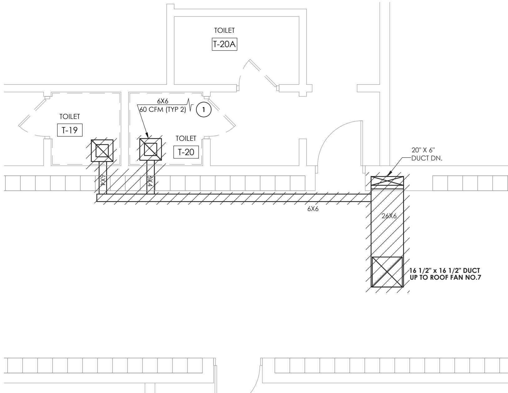
2 H102 TOILET ROOM 12 DEMOLITION PLAN SCALE: 1/4" = 1'-0"
