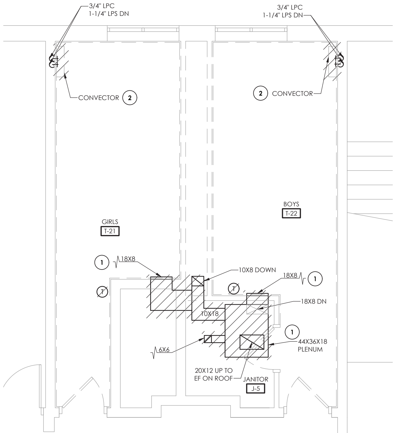
3 H102 TOILET ROOMS T-21 AND T-22 DEMOLITION PLAN SCALE: 1/8" = 1'-0"
