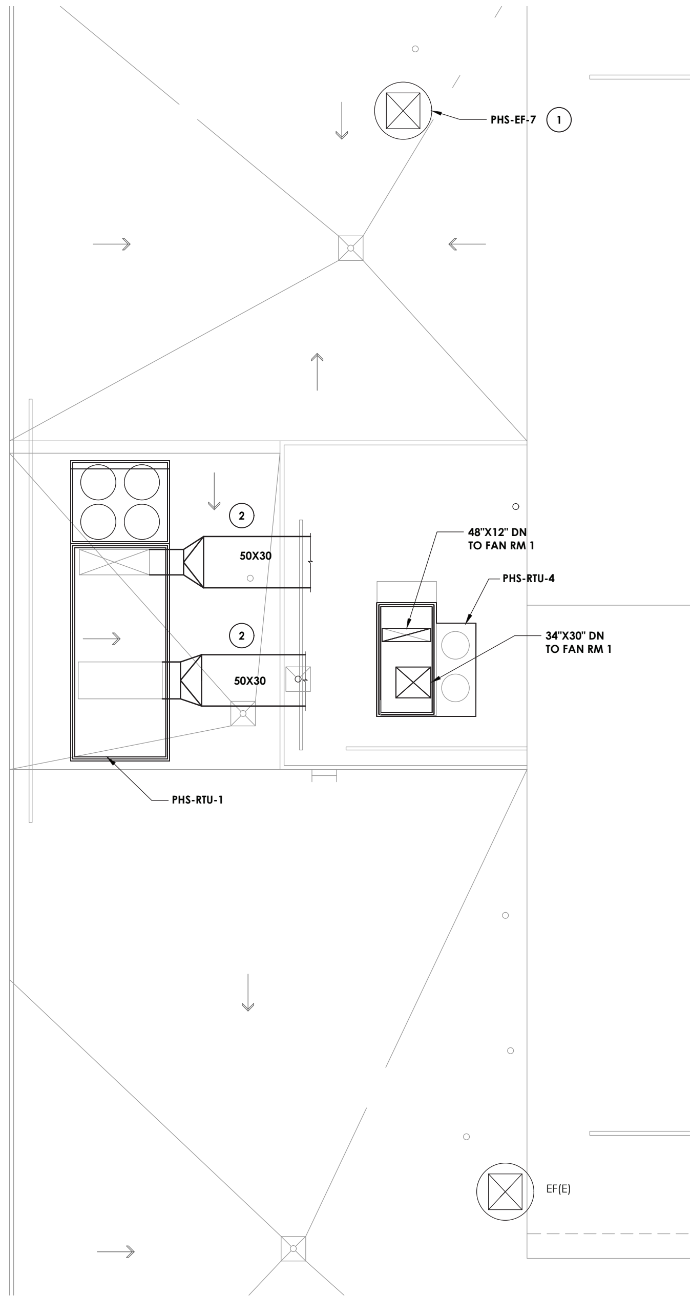
3 H203 SCALE: 1/8" = 1'-0" ROOF HVAC NEW WORK PLAN
