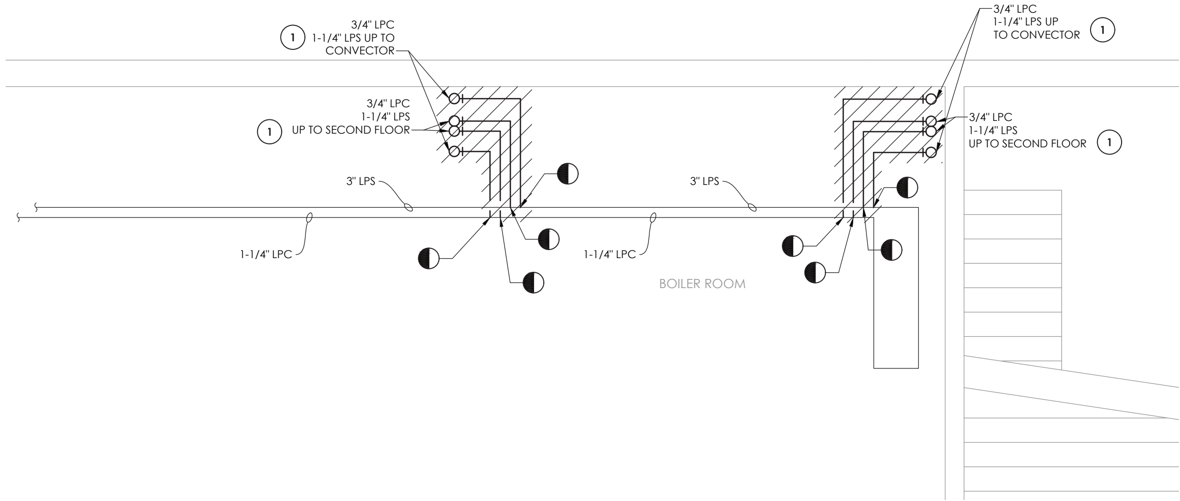
2 BOILER ROOM BELOW T-11 AND T-12 HVAC DEMOLITION PLAN SCALE: 1/4" = 1'-0"
