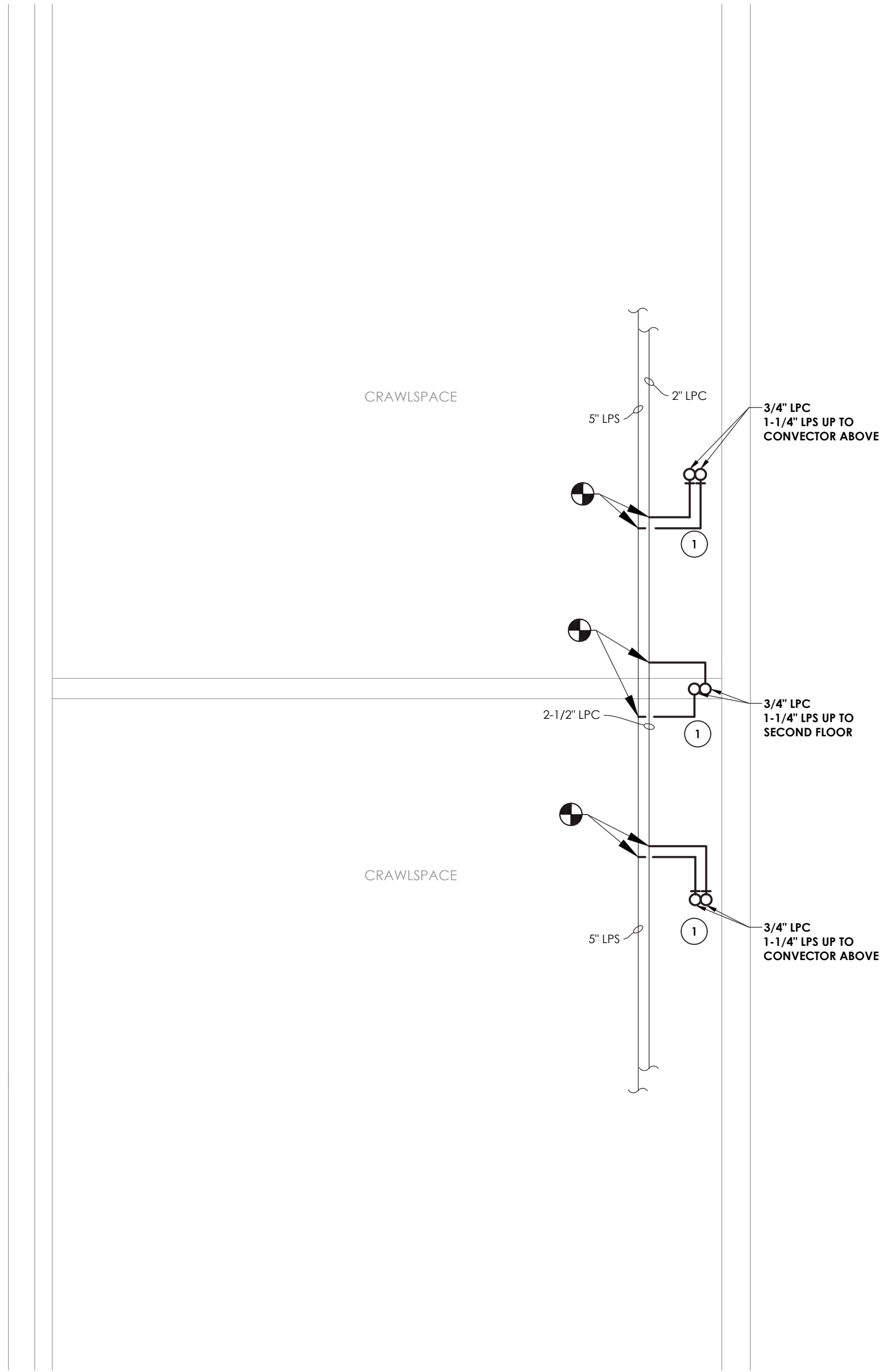
1 H200 CRAWLSPACE BELOW T-1 AND T-2 HVAC NEW WORK PLAN SCALE: 1/4" = 1'-0"
