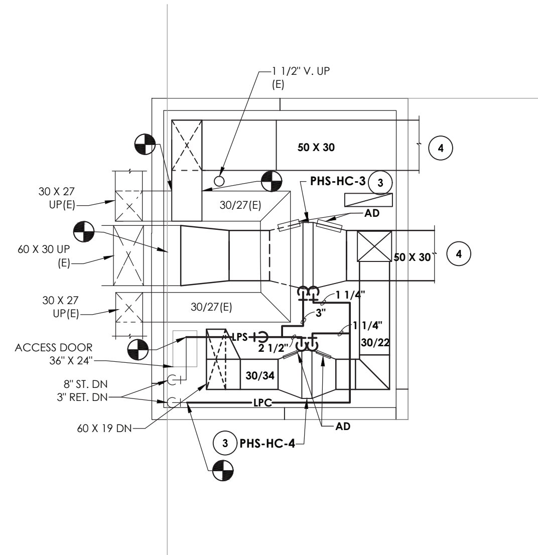
6 H202 FAN ROOM 2 HVAC NEW WORK PLAN (BOYS) SCALE: 1/4" = 1'-0"
