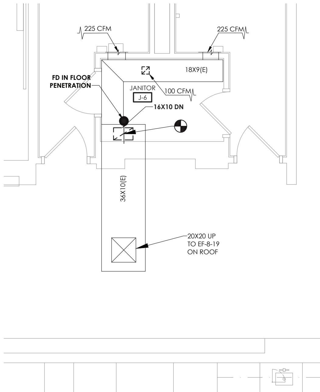
5 H202 SECOND FLOOR TOILET ROOMS T-23 & T-24 HVAC NEW WORK PLAN SCALE: 1/4" = 1'-0"
