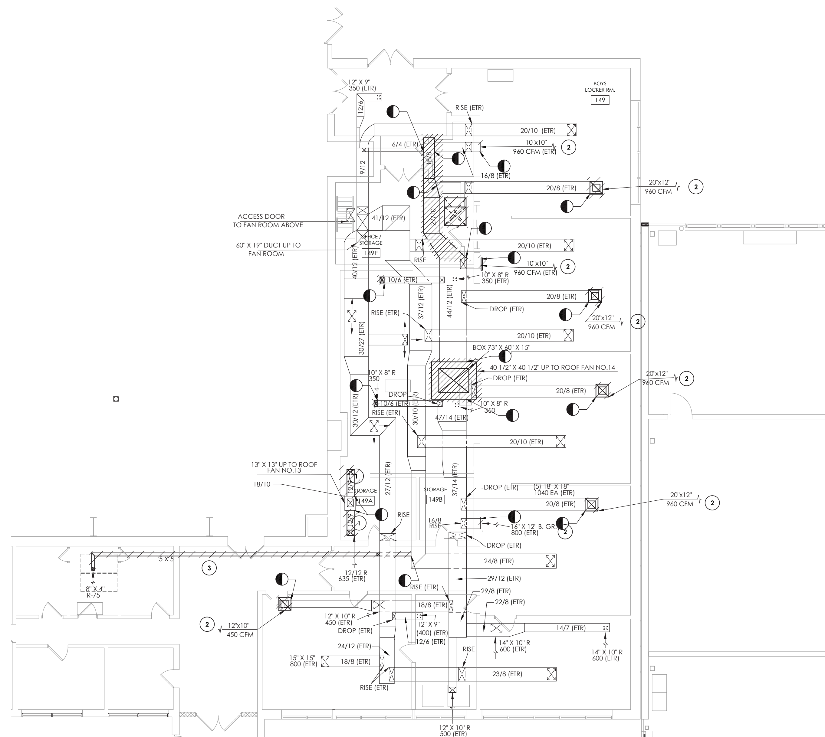
8 BOYS' LOCKER ROOM HVAC DEMOLITION PLAN H101B SCALE: 1/8" = 1'-0"
