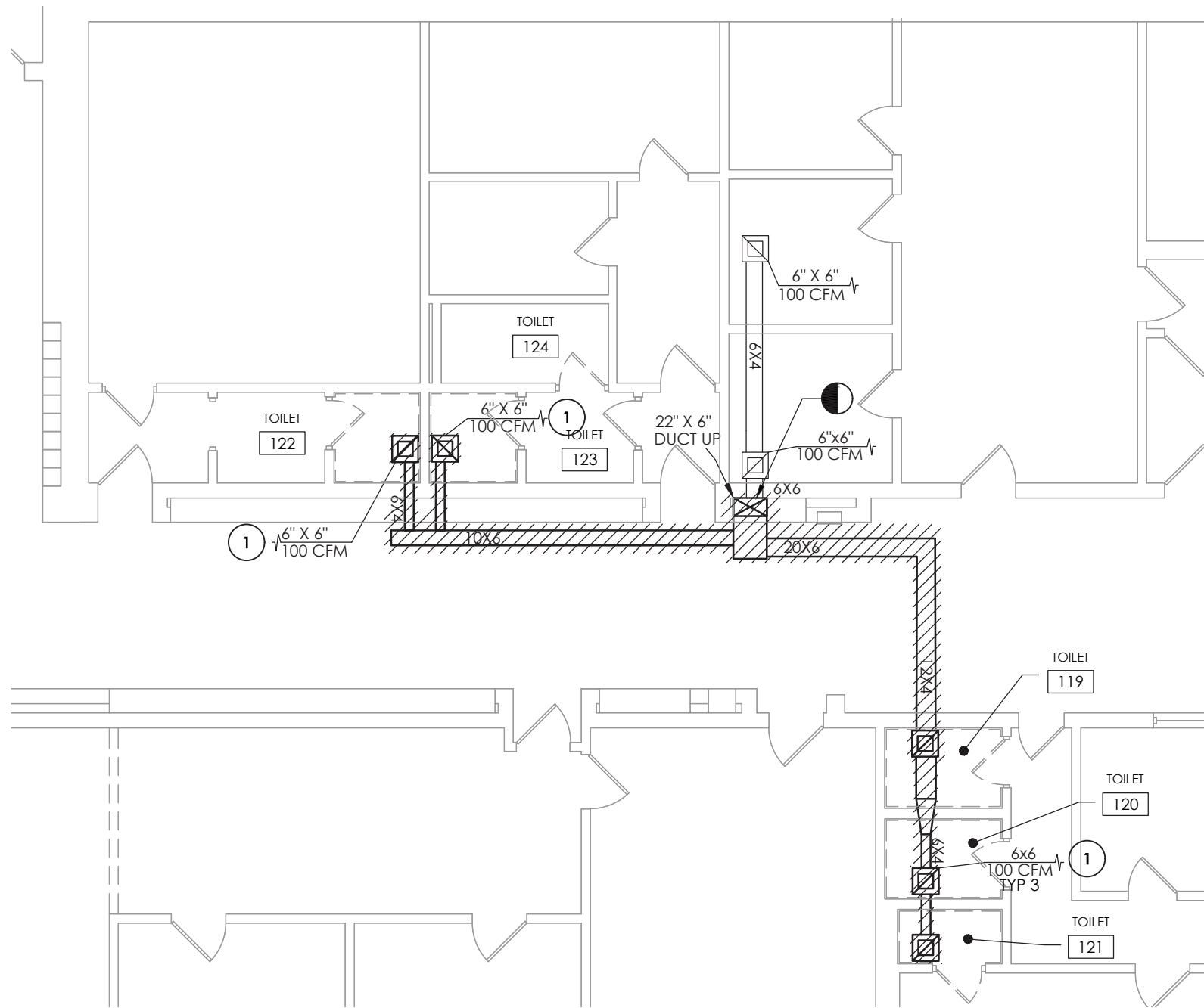
6 H101A TOILET ROOM 5 DEMOLITION PLAN SCALE: 1/8" = 1'-0"
