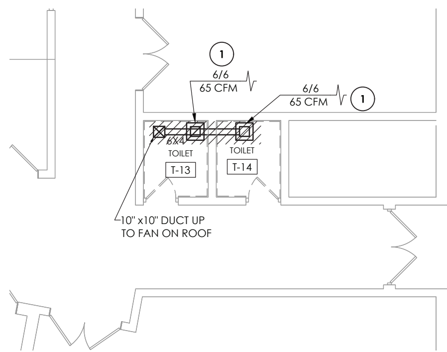
7 H101A TOILET ROOMS T-13 AND T-14 DEMOLITION PLAN SCALE: 1/8" = 1'-0"
