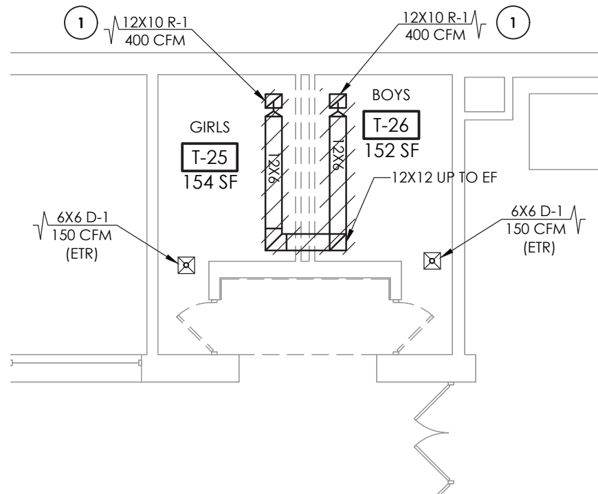
4 H101A TOILET ROOM DEMOLITION PLAN SCALE: 1/8" = 1'-0"
