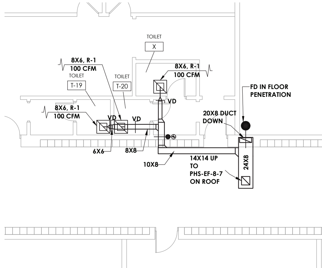
2 H202 SECOND FLOOR TOILET ROOMS T-19 & T-20 HVAC NEW WORK PLAN SCALE: 1/8" = 1'-0"
