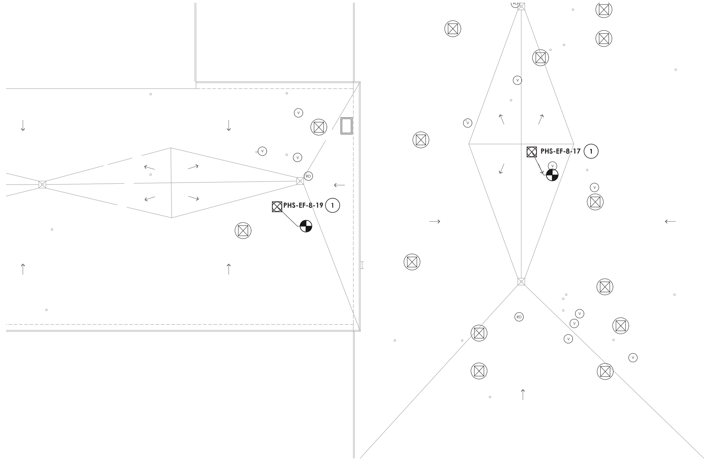
2 H203 SCALE: 1/16" = 1'-0" ROOF HVAC NEW WORK PLAN
