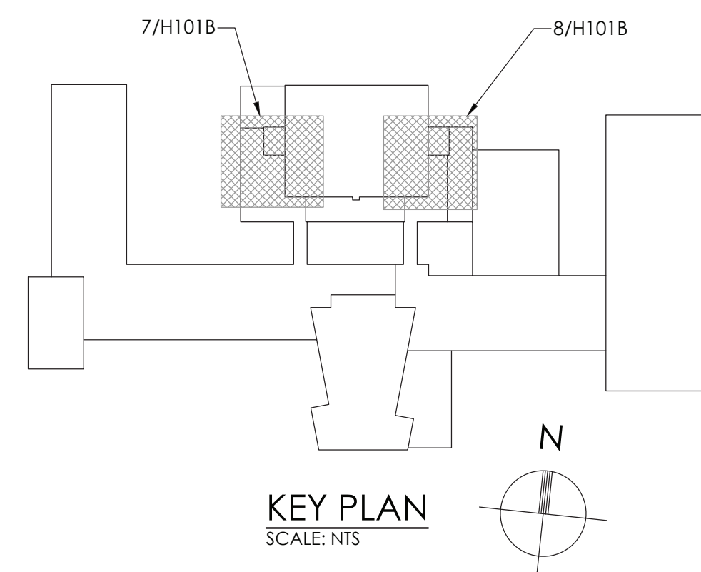
8 BOYS' LOCKER ROOM HVAC DEMOLITION PLAN H101B SCALE: 1/8" = 1'-0"
