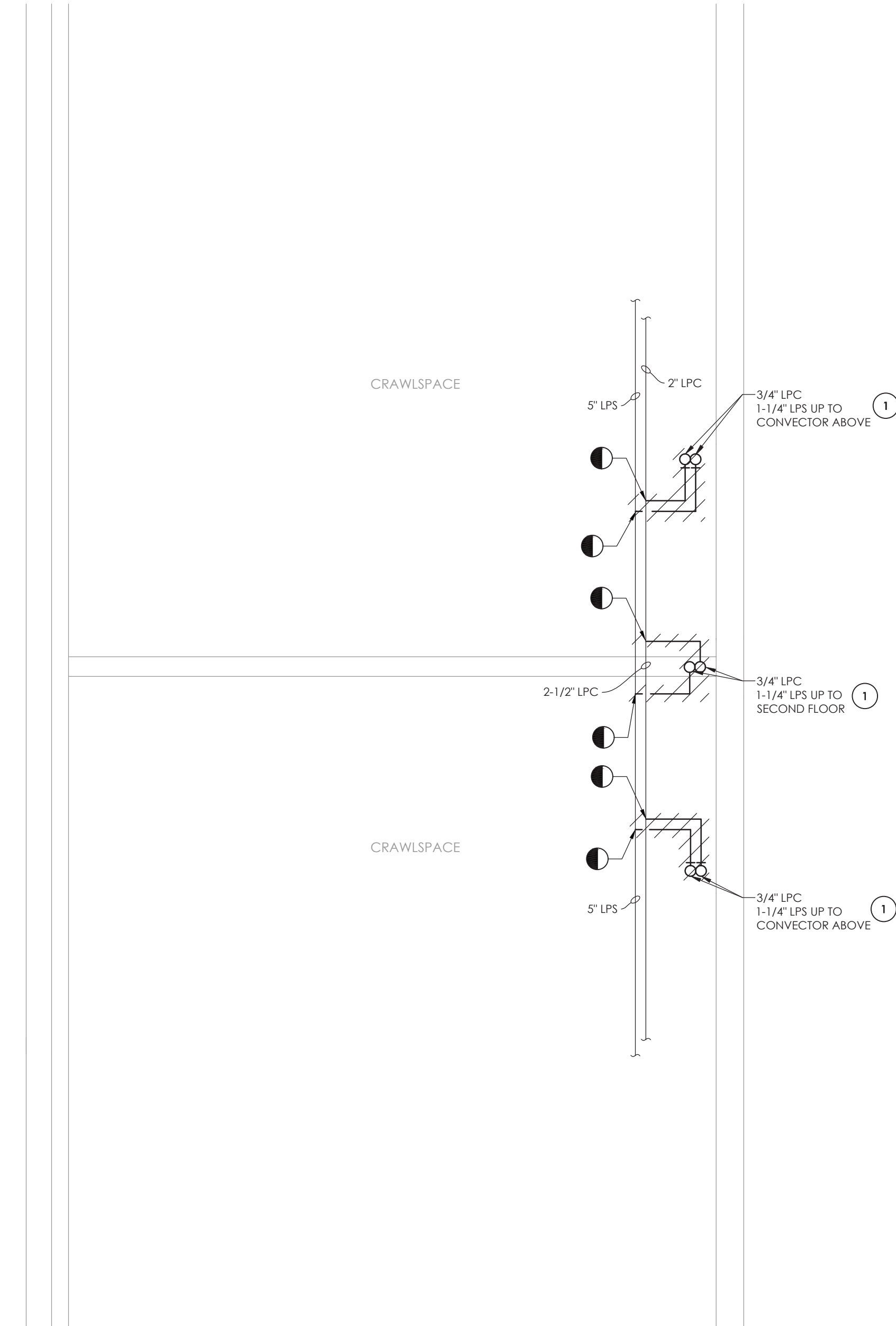
1 CRAWLSPACE BELOW T-1 AND T-2 HVAC DEMOLITION PLAN SCALE: 1/4" = 1'-0"
