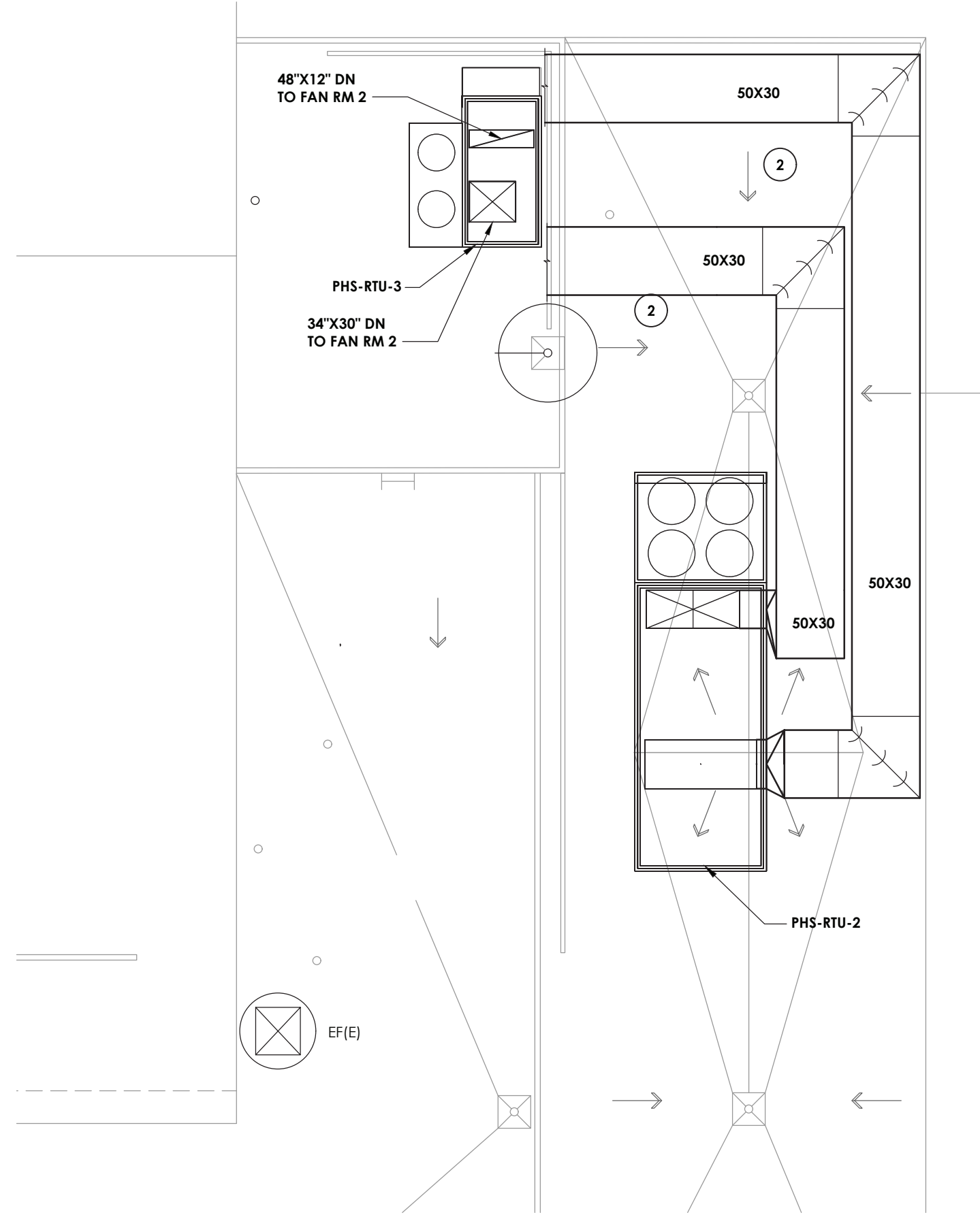
4 H203 SCALE: 1/8" = 1'-0" ROOF HVAC NEW WORK PLAN
