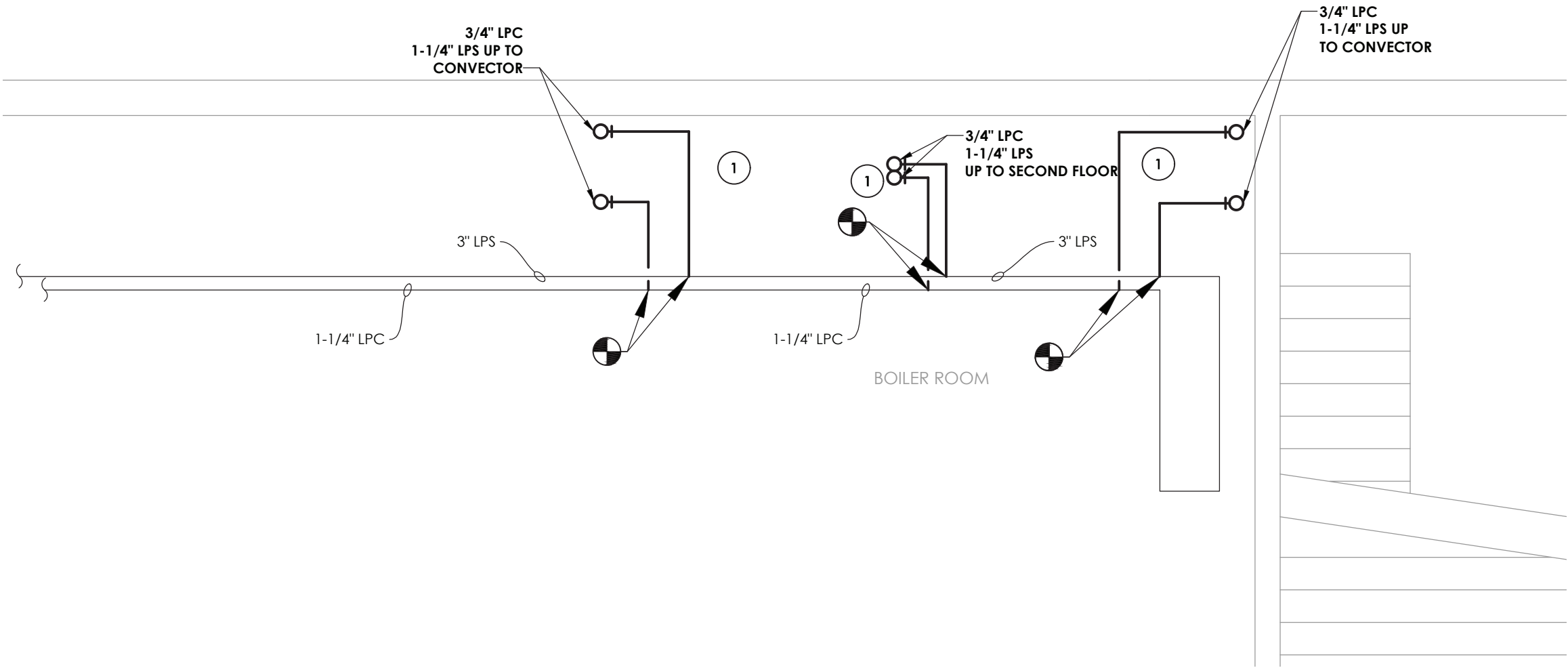
2 H200 CRAWLSPACE BELOW T-11 AND T-12 HVAC NEW WORK PLAN SCALE: 1/4" = 1'-0"
