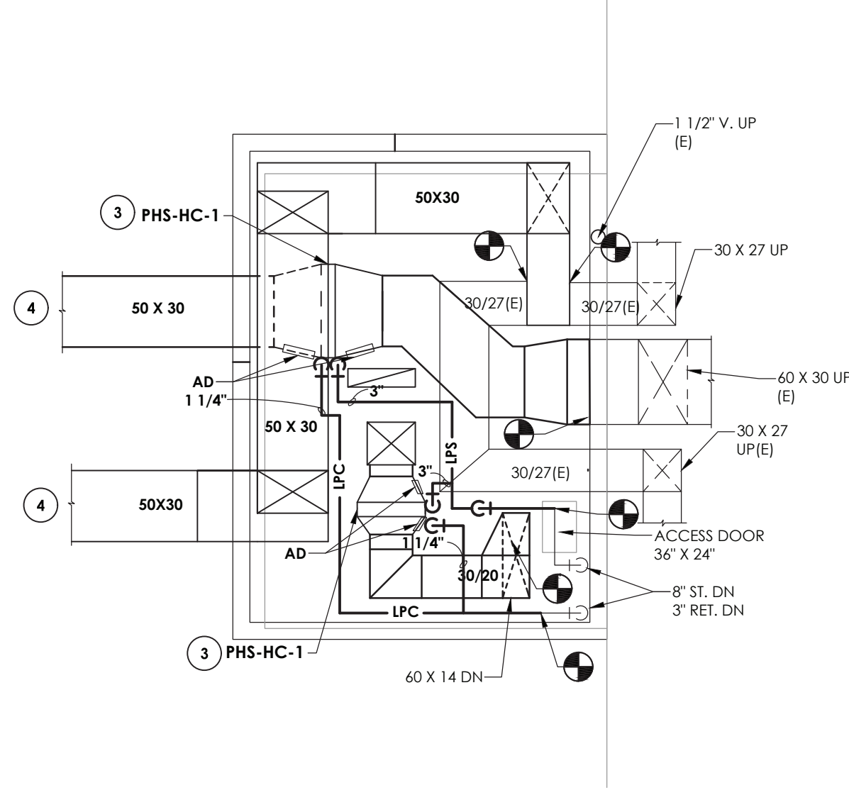
3 H202 FAN ROOM 1 HVAC NEW WORK PLAN (GIRLS) SCALE: 1/4" = 1'-0"
