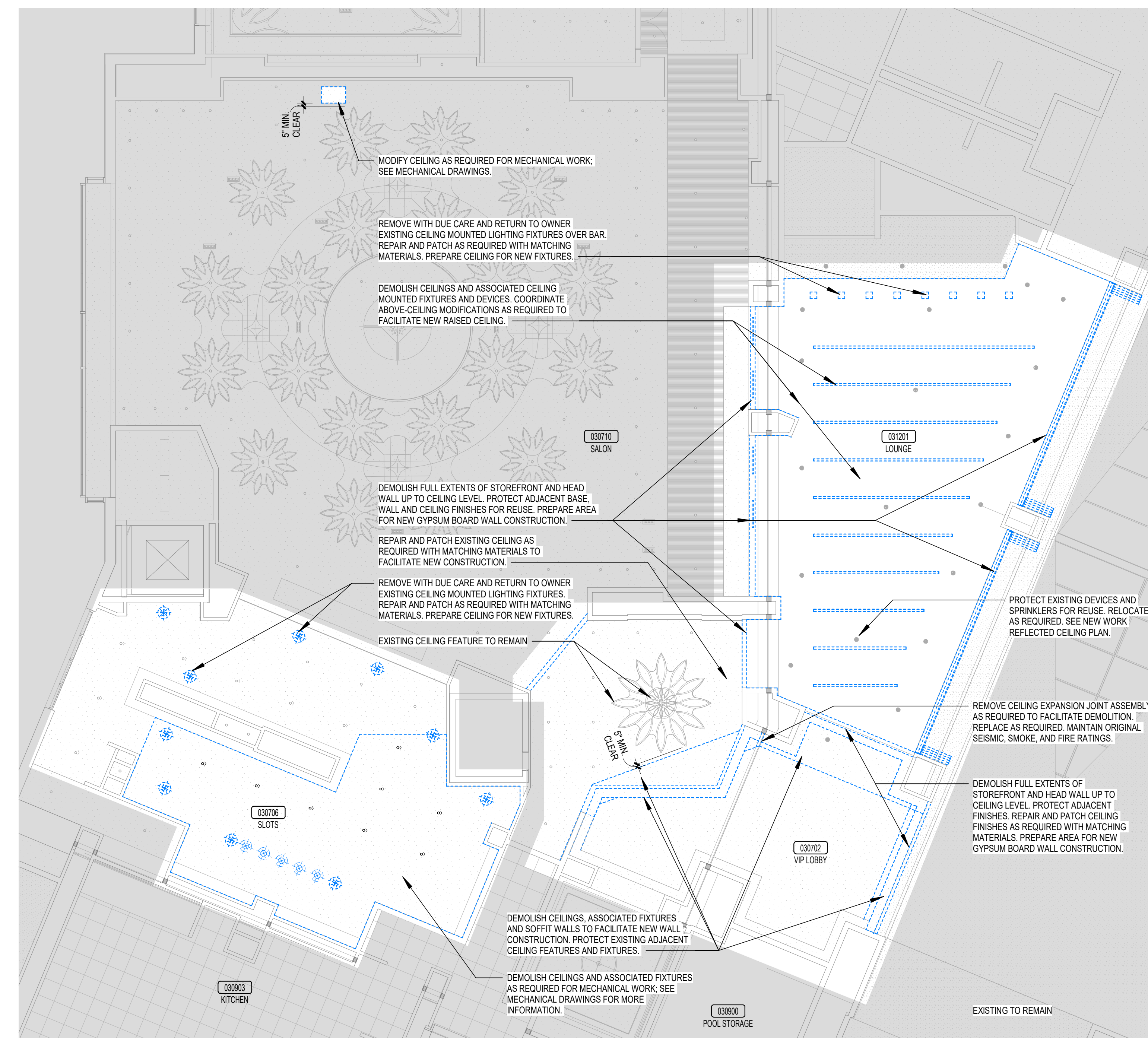
2 OVERALL CEILING DEMOLITION PLAN - THIRD FLOOR
