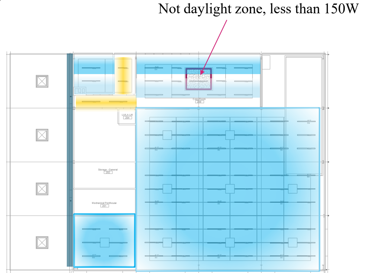
First Floor
