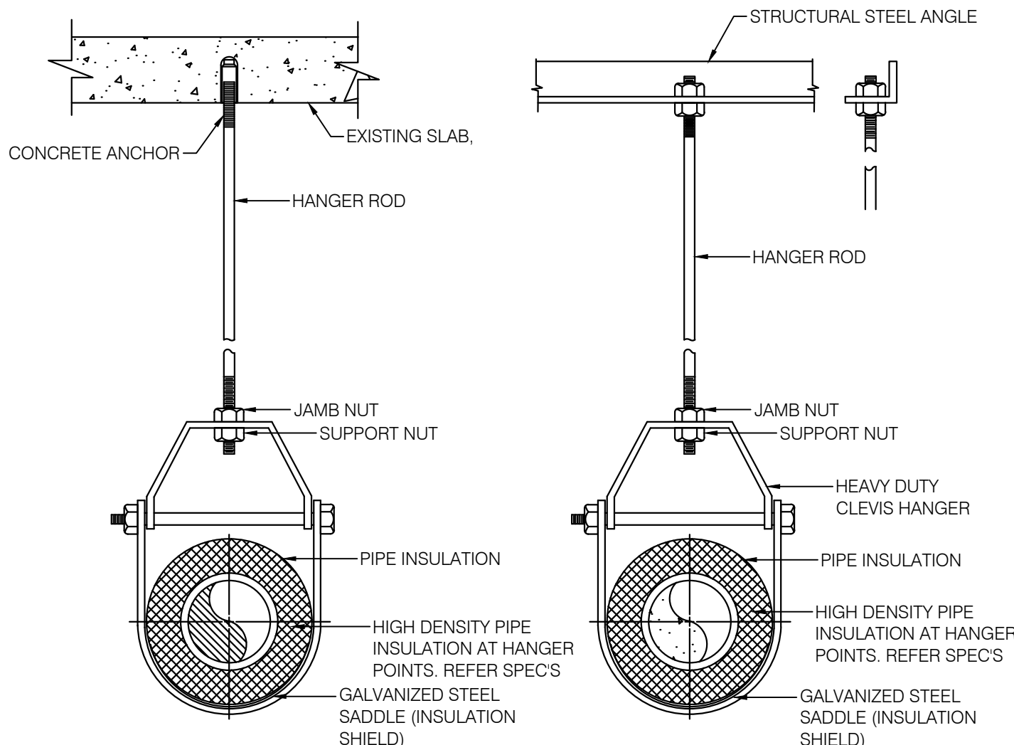
1 PIPE SUPPORT DETAIL
