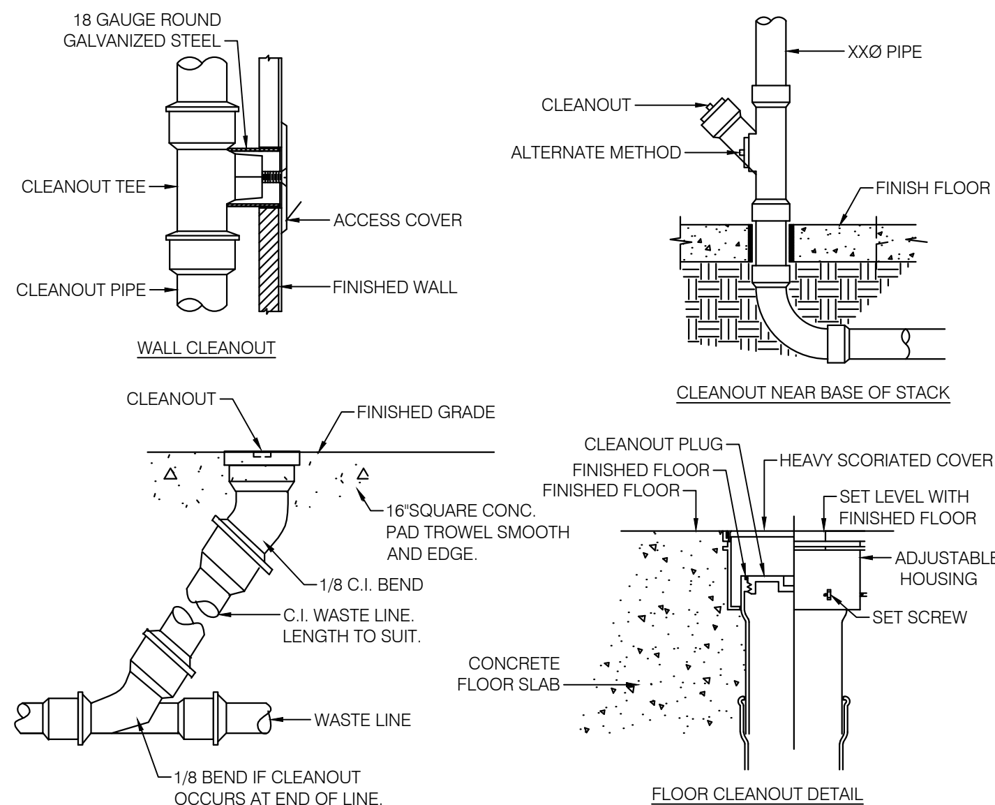
5 CLEANOUT DETAILS
