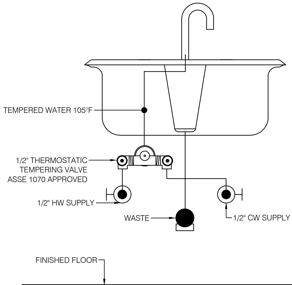
4 POINT OF USE MIXING VALVE DETAIL
