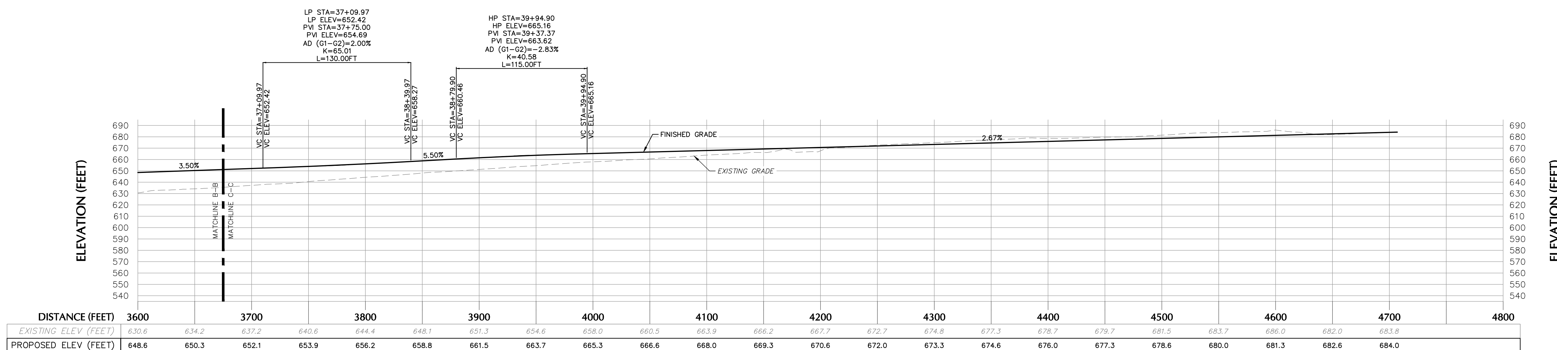
PUGSLEY ROAD PROFILE VERTICAL SCALE: 1" = 50' HORIZONTAL SCALE: 1" = 50'
