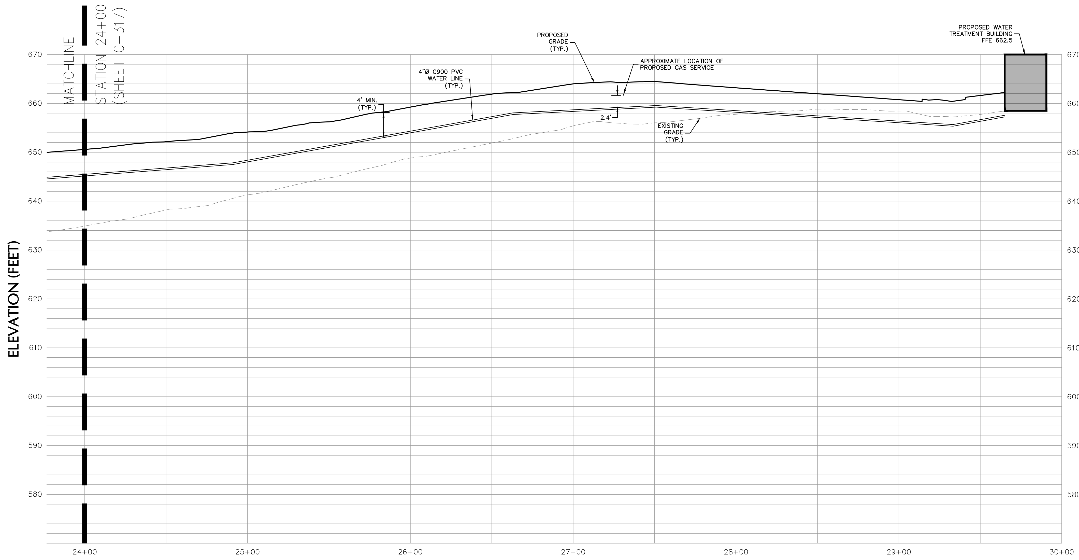
4 INCH FROM SOUTHERN WELL TO WATER TREATMENT (VIEW C: SEE PLAN C-302)
