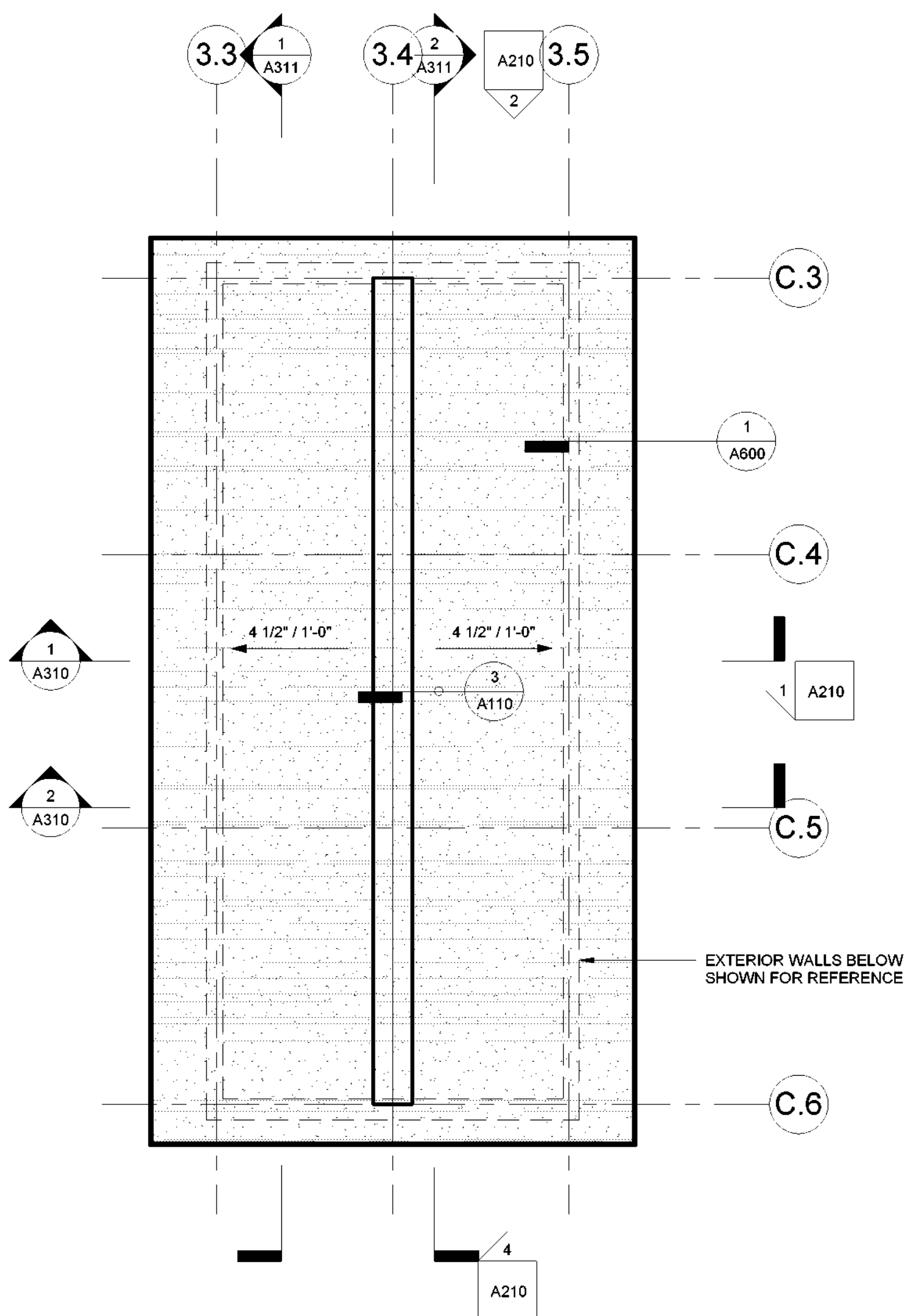
② LATRINE #427 ROOF PLAN 1/4" = 1'-0"
