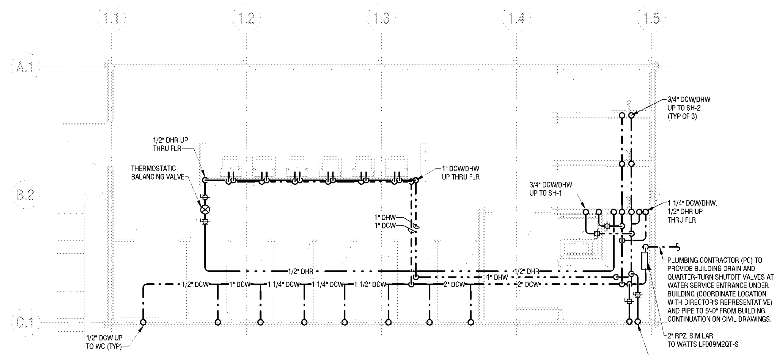
2 BATHHOUSE 231 & 322 PLUMBING PLAN - UNDERFLOOR DOMESTIC P102 1/4" = 1'-0"
