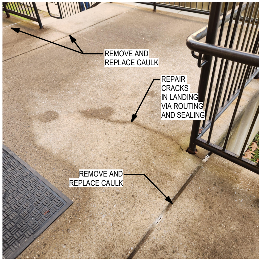
15 PHOTO AREA D - 006 A502 12" = 1'-0"
