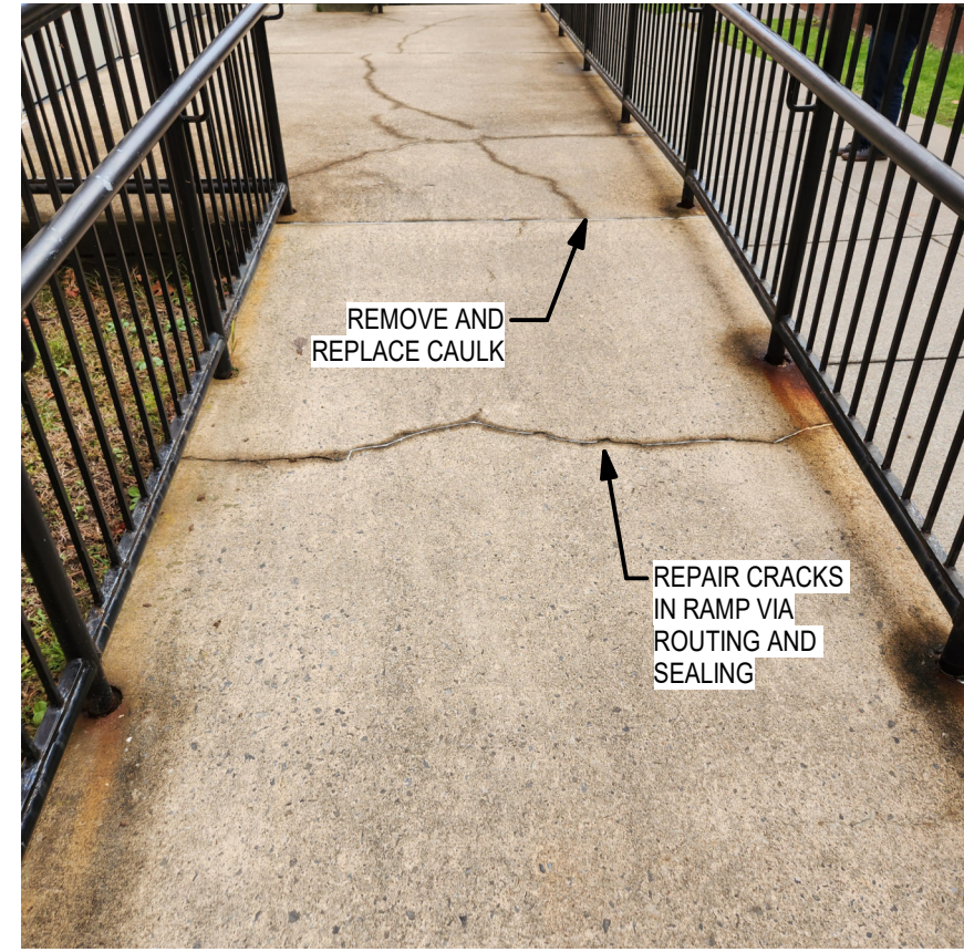
8 PHOTO AREA C - 001 A502 12" = 1'-0"
