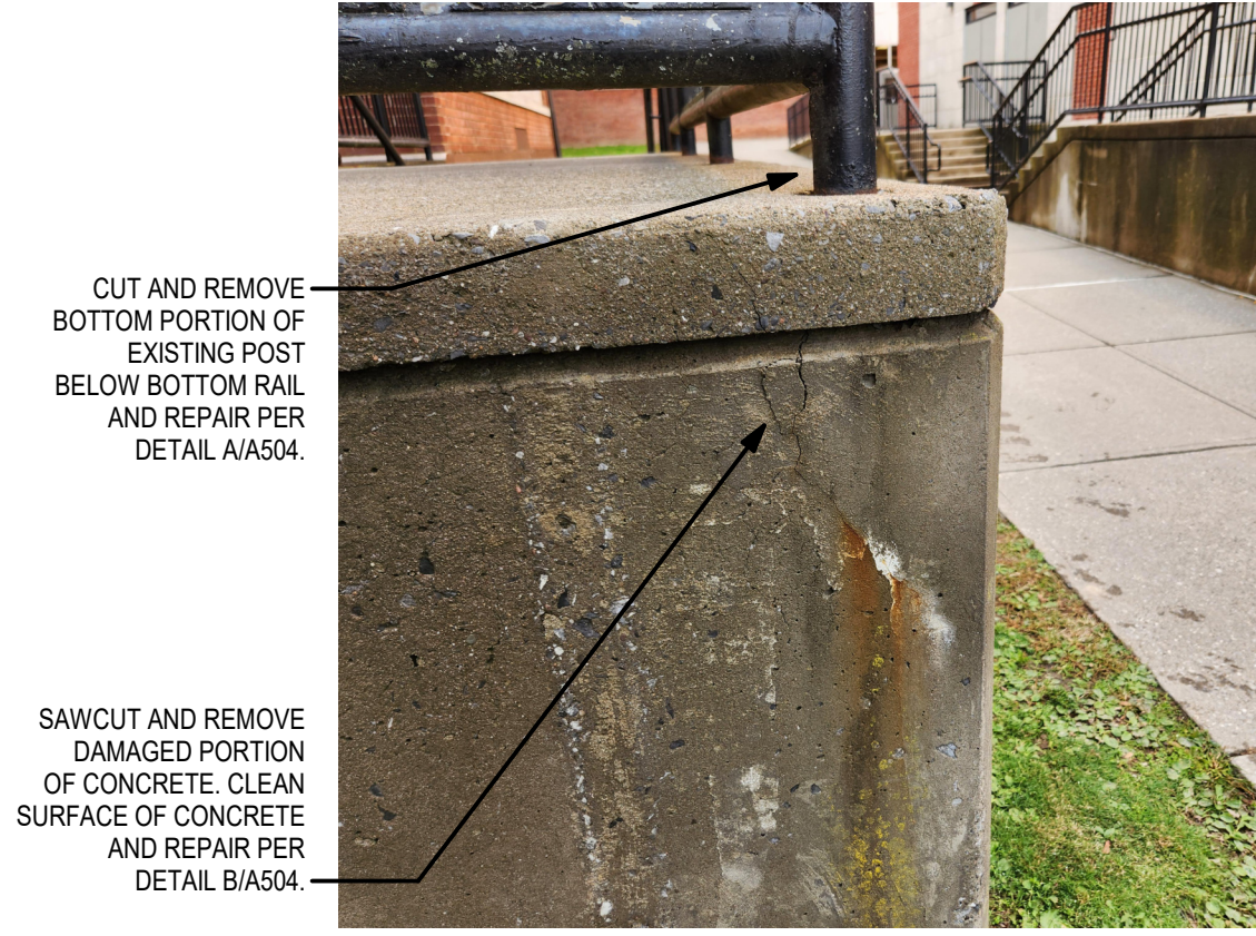
14 PHOTO AREA D - 005 A502 12" = 1'-0"
