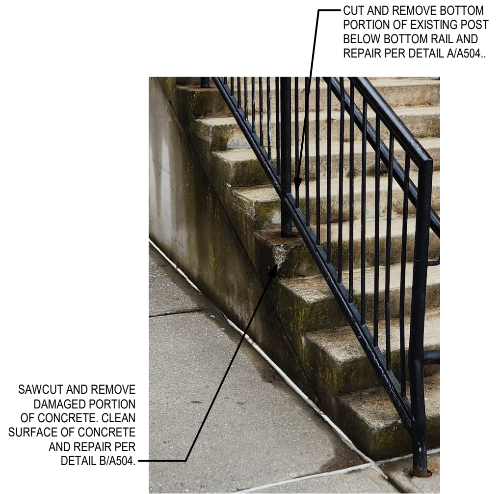
6 PHOTO AREA B - 002 A502 12" = 1'-0"
