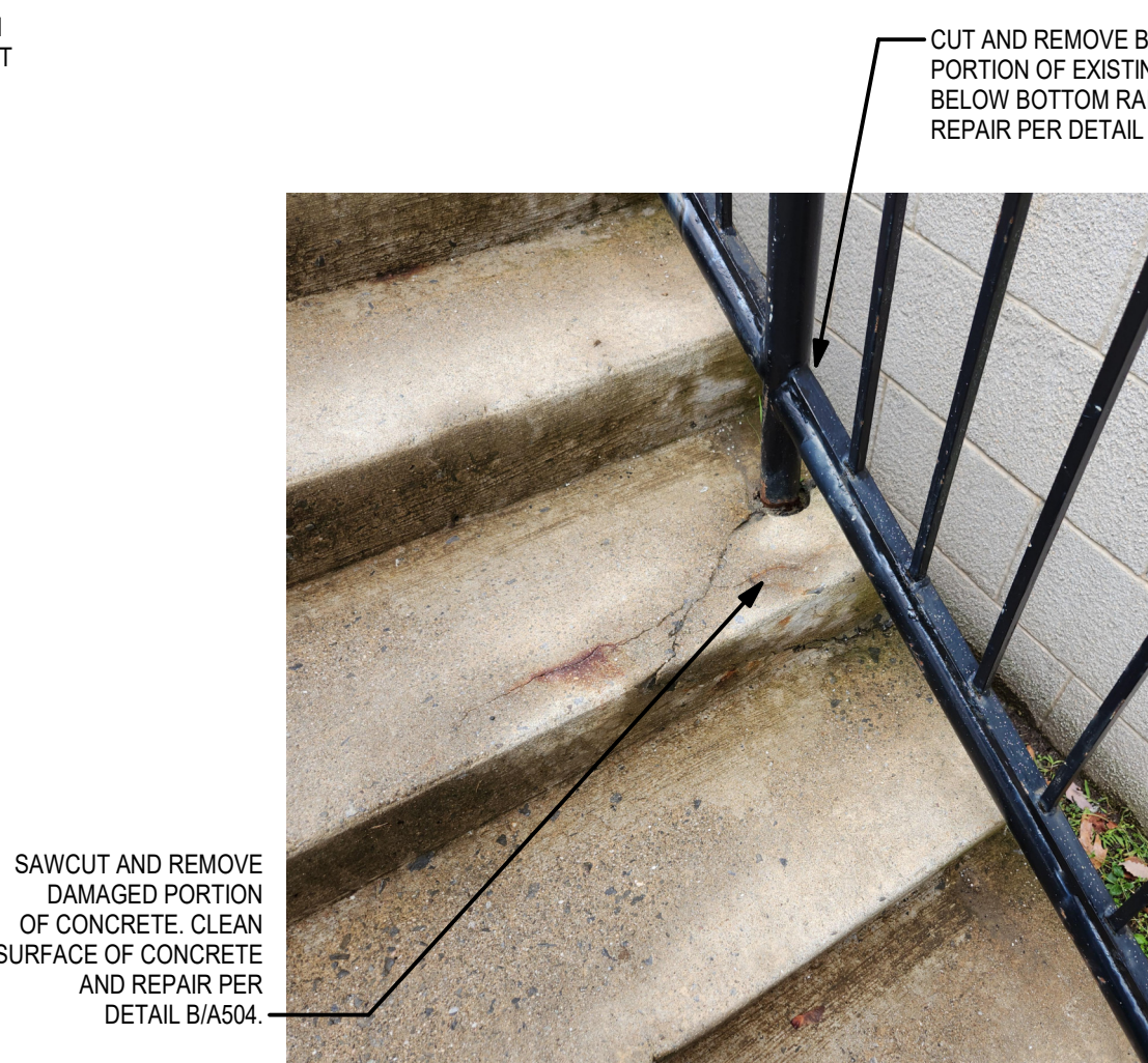
3 PHOTO AREA A - 003 A502 12" = 1'-0"
