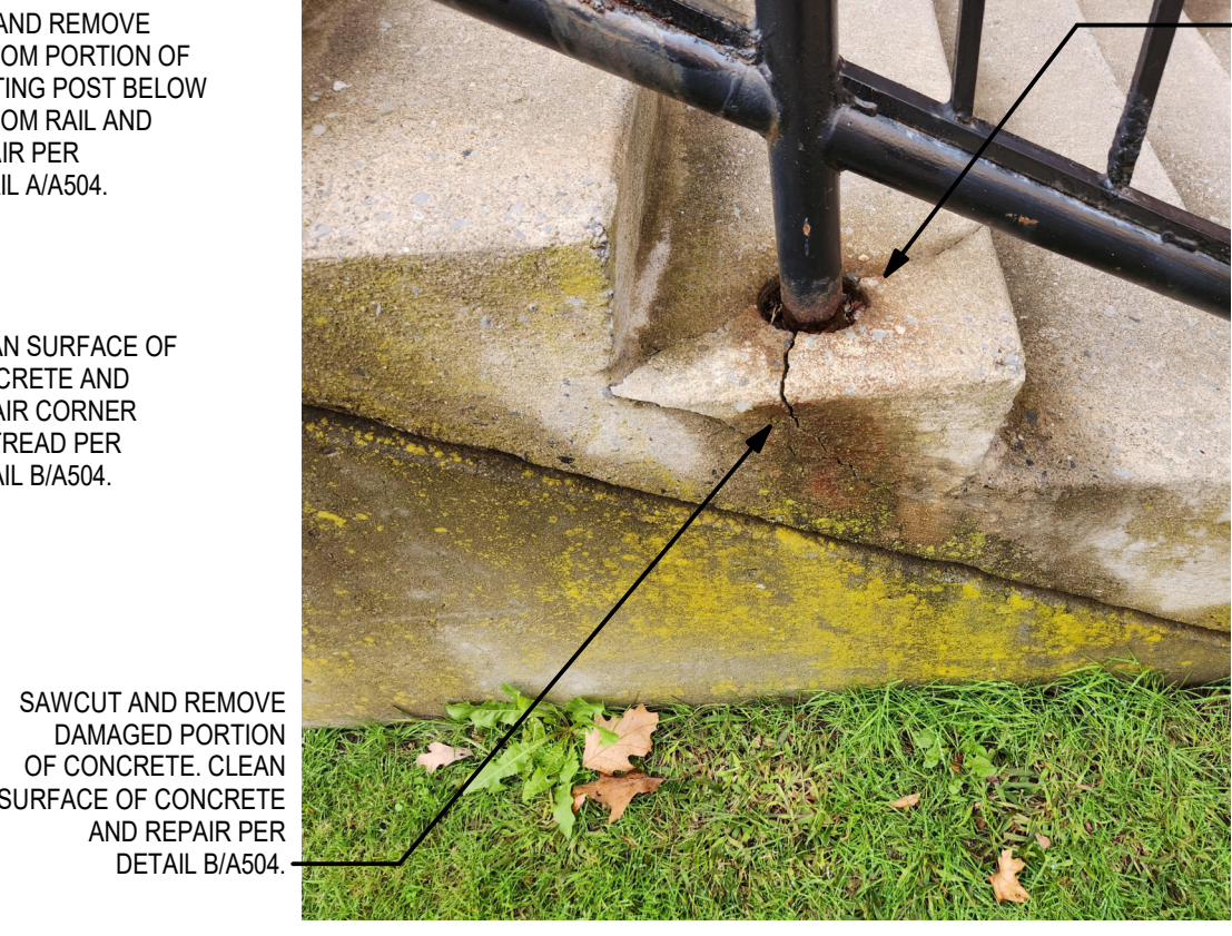
12 PHOTO AREA D - 003 A502 12" = 1'-0"
