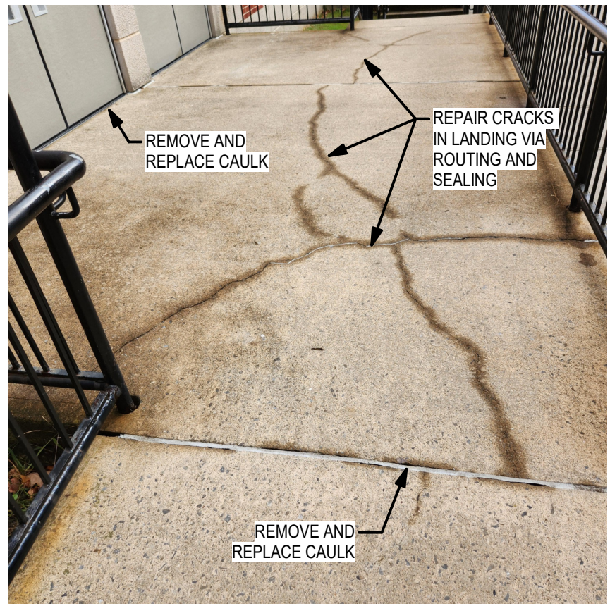
9 PHOTO AREA C - 002 A502 12" = 1'-0"
