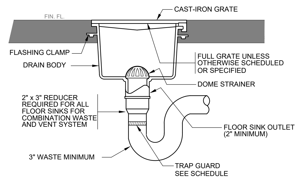
FLOOR SINK DETAIL
