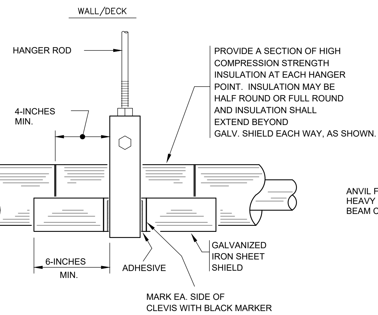
CLEVIS HANGER - PIPE WITH EXTERNAL INSULATION -
