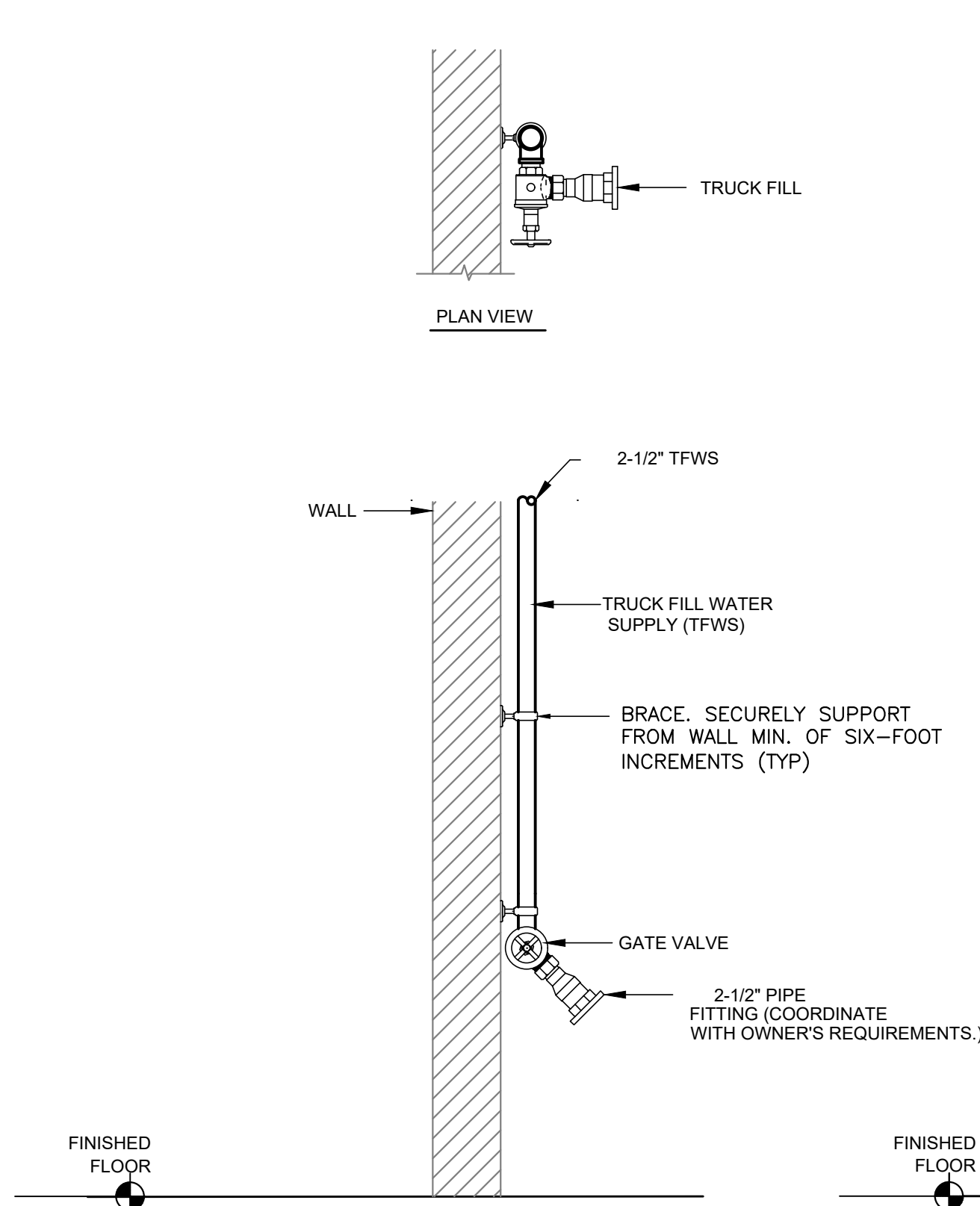
TRUCK FILL WALL HYDRANT DETAIL
