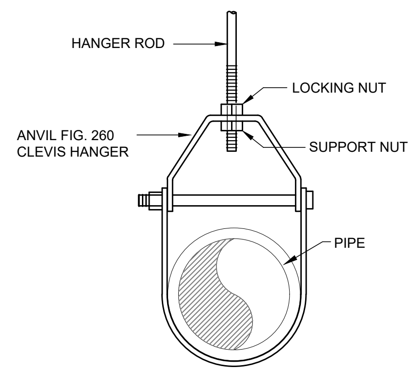
CLEVIS HANGER - PIPE WITH NO INSULATION -
