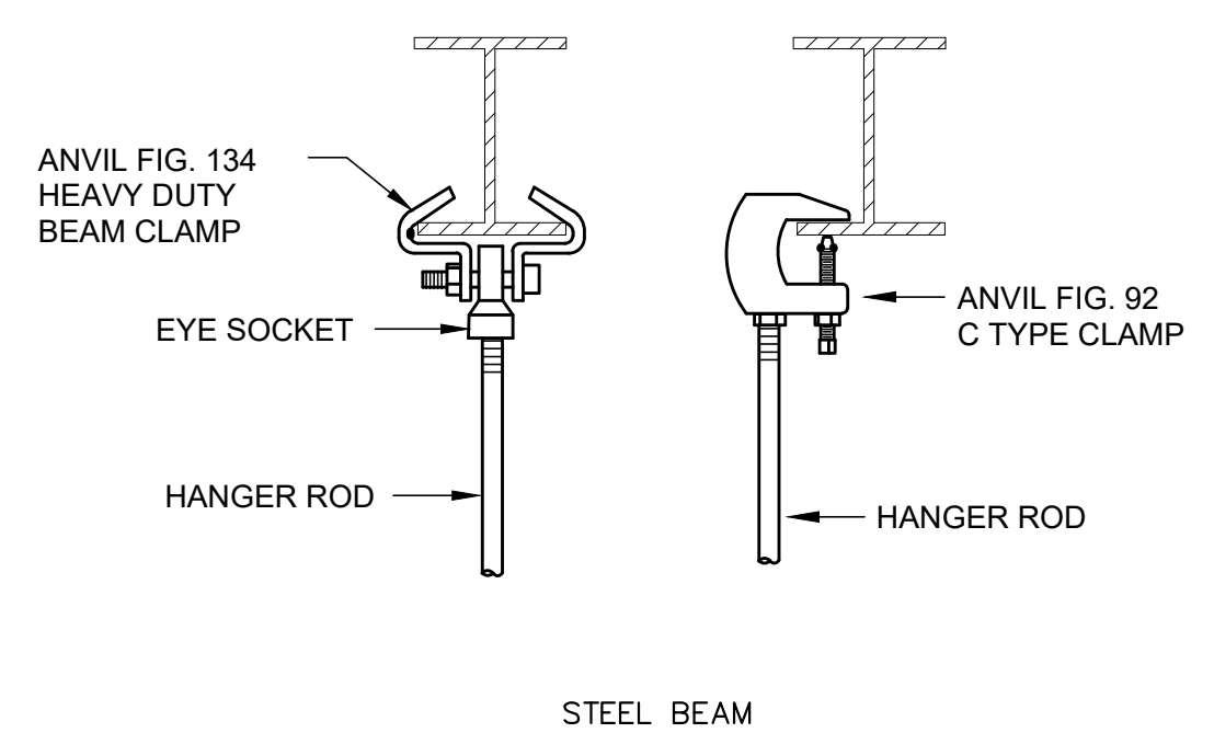
STEEL BEAM
