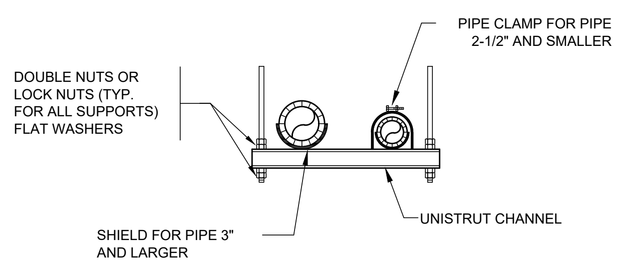
TYPICAL PIPE SUPPORT DETAILS
