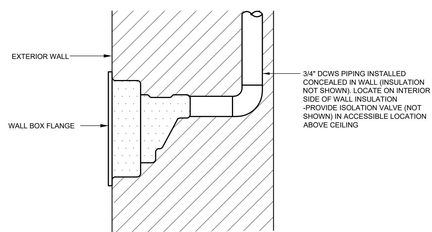
FREEZEPROOF WALL HYDRANT
