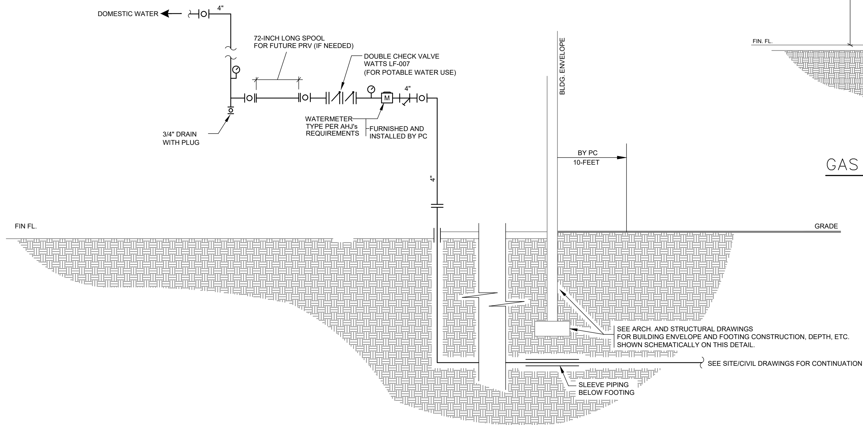
WATER SERVICE ENTRANCE DETAIL
