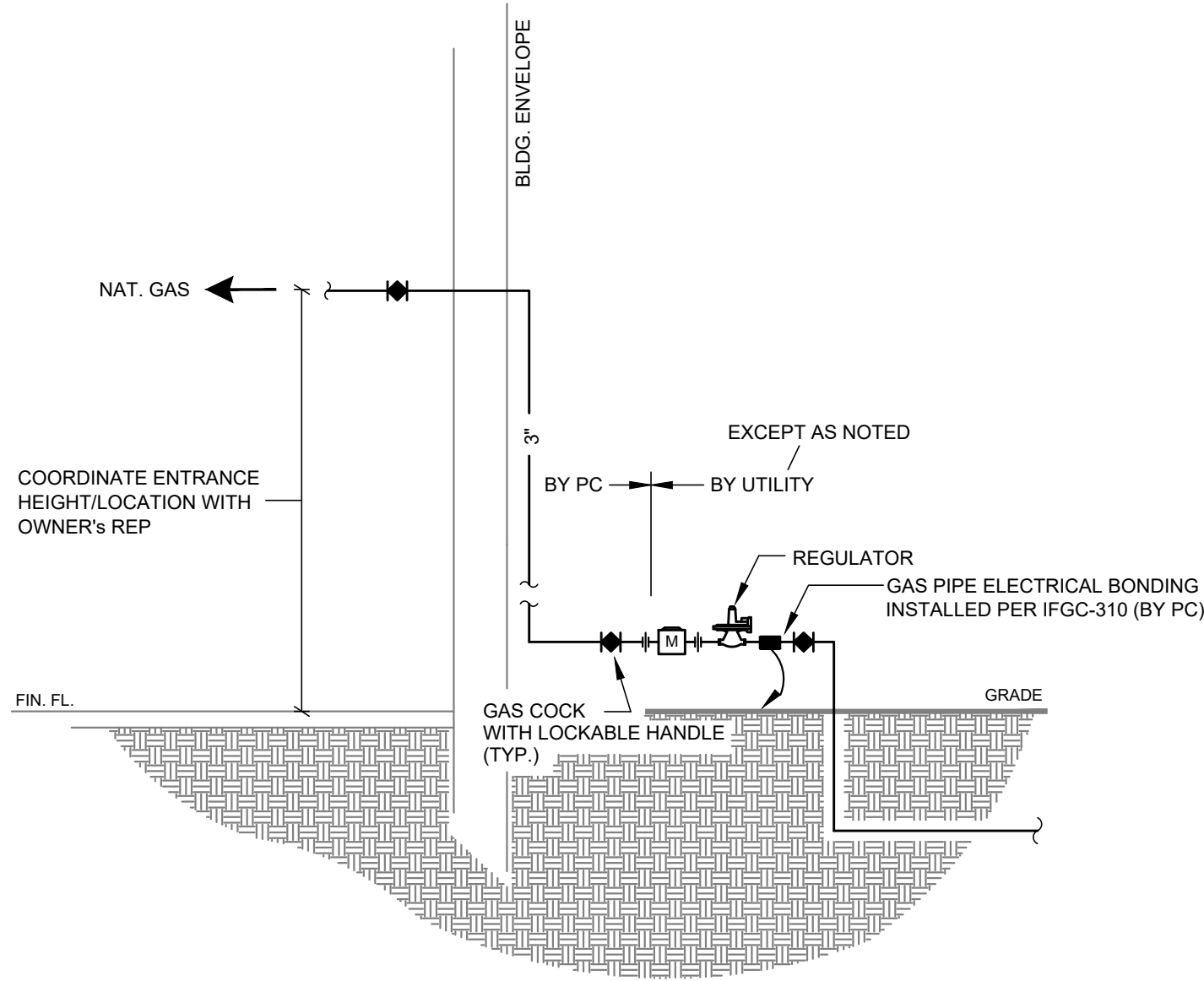
GAS SERVICE ENTRANCE DETAIL
