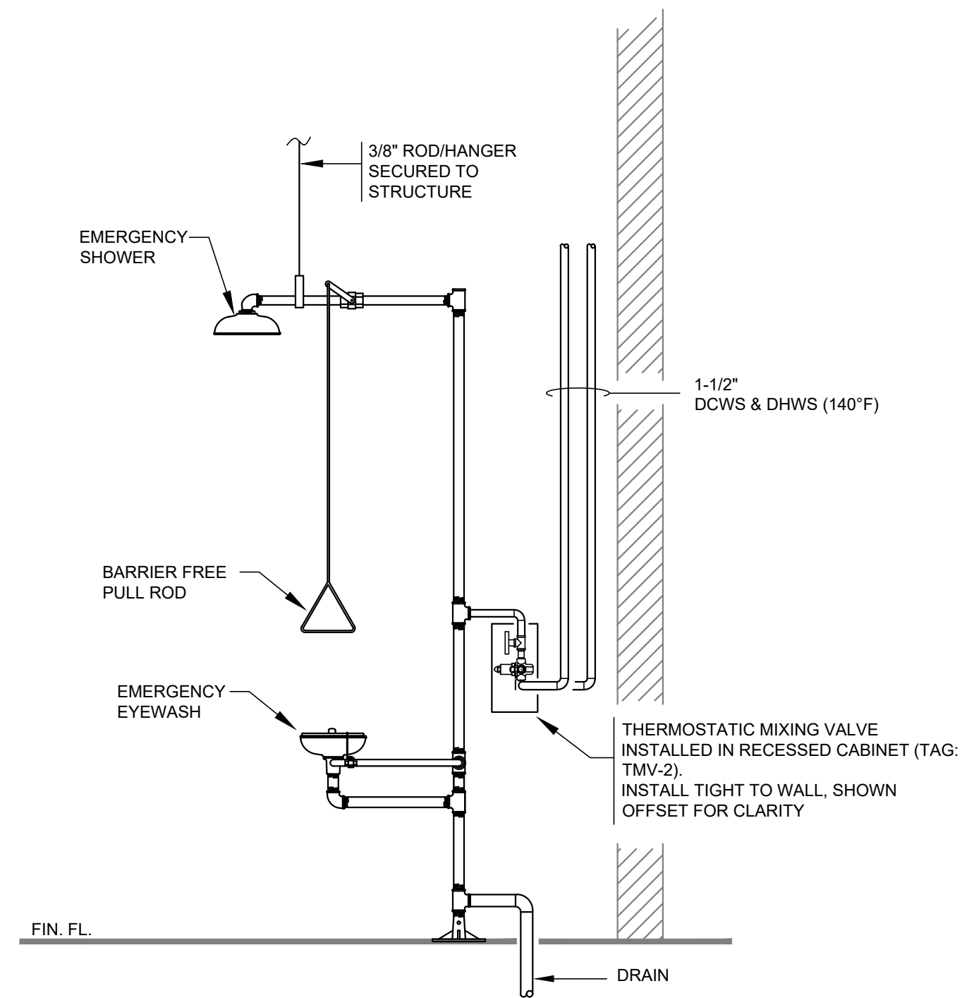
COMBINATION SHOWER/EYEWASH DETAIL
