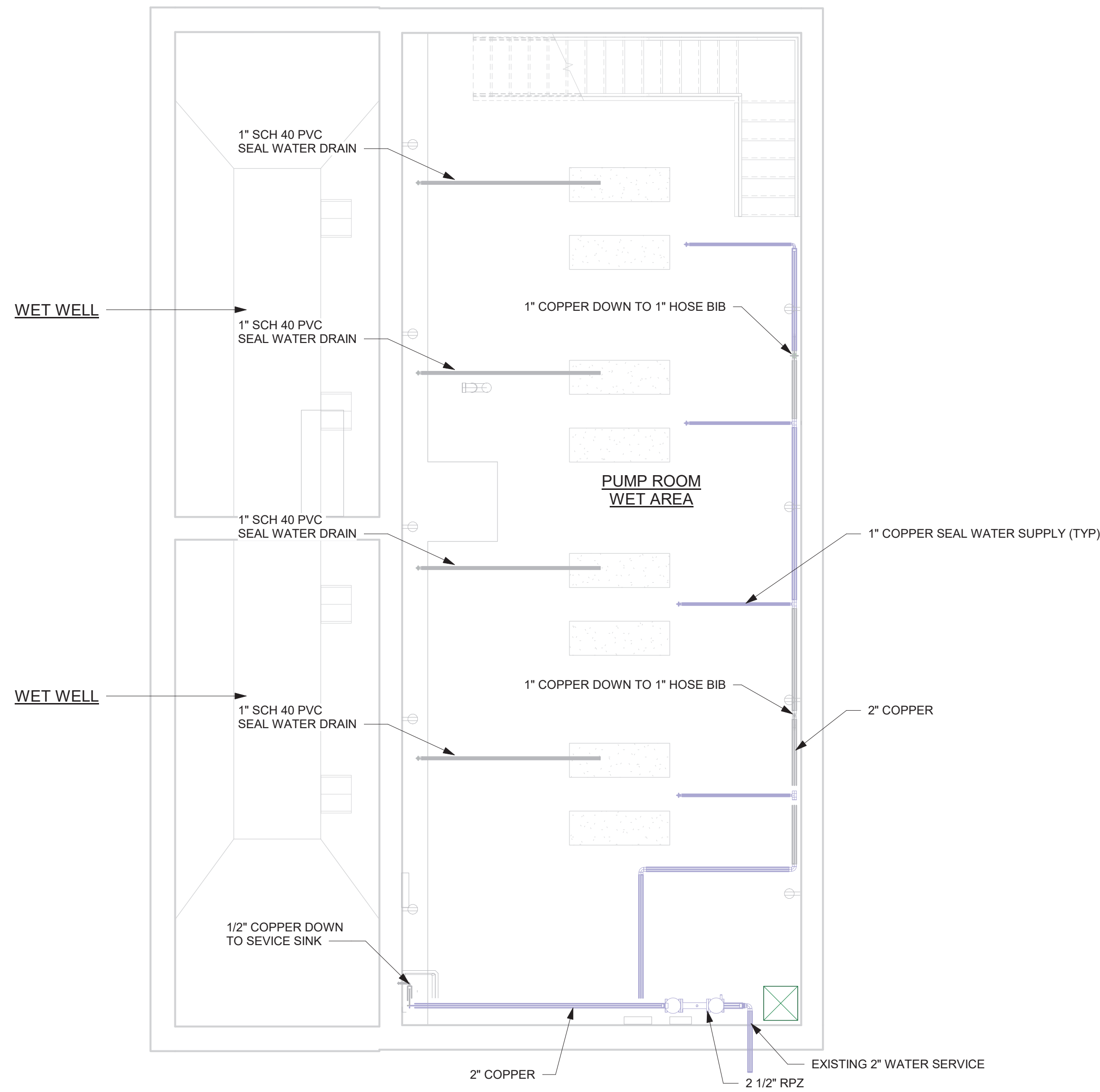
1 LOWER FLOOR - PLUMBING 1/4" = 1'-0"
