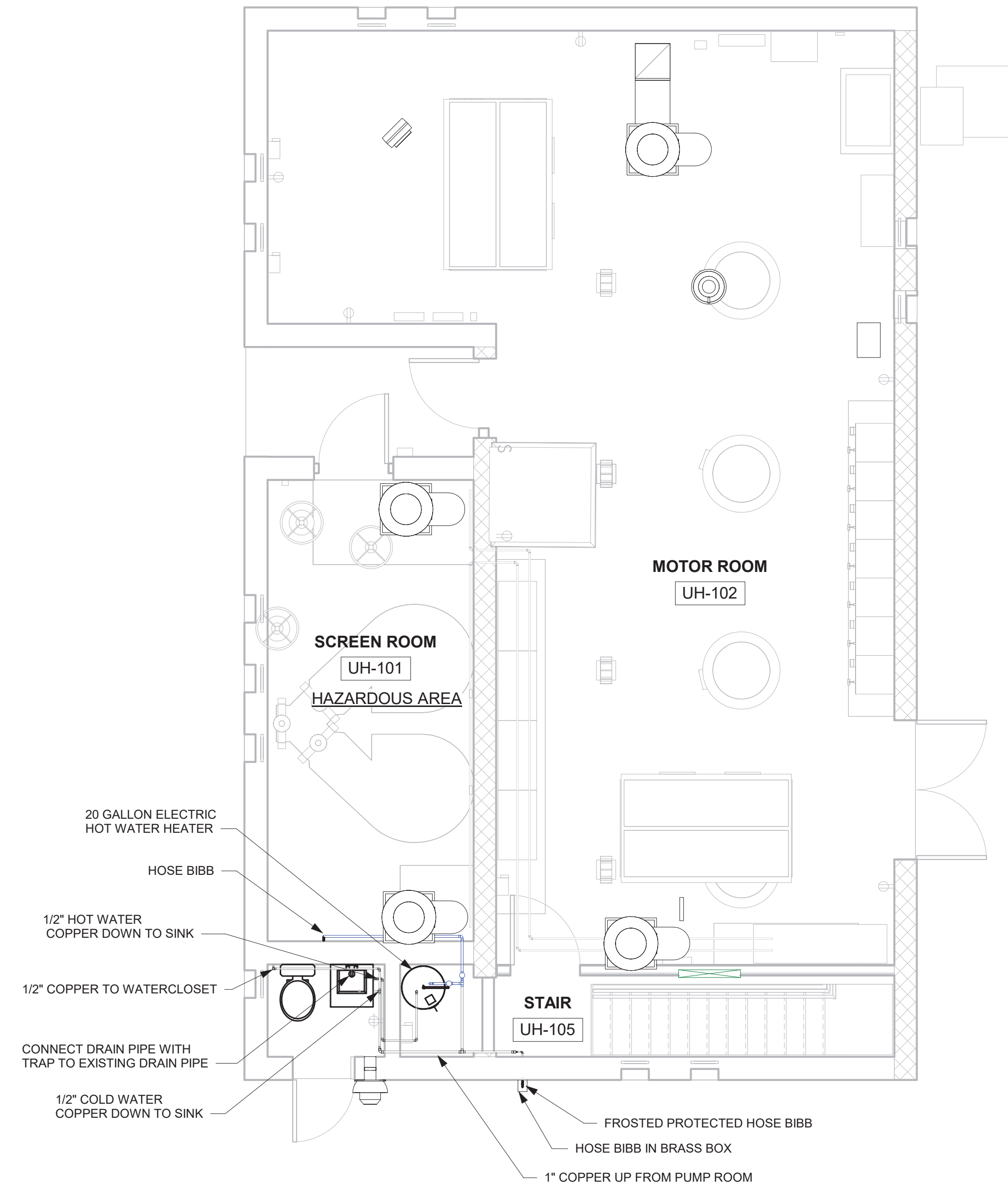
② GROUND FLOOR - PLUMBING 1/4" = 1'-0"
