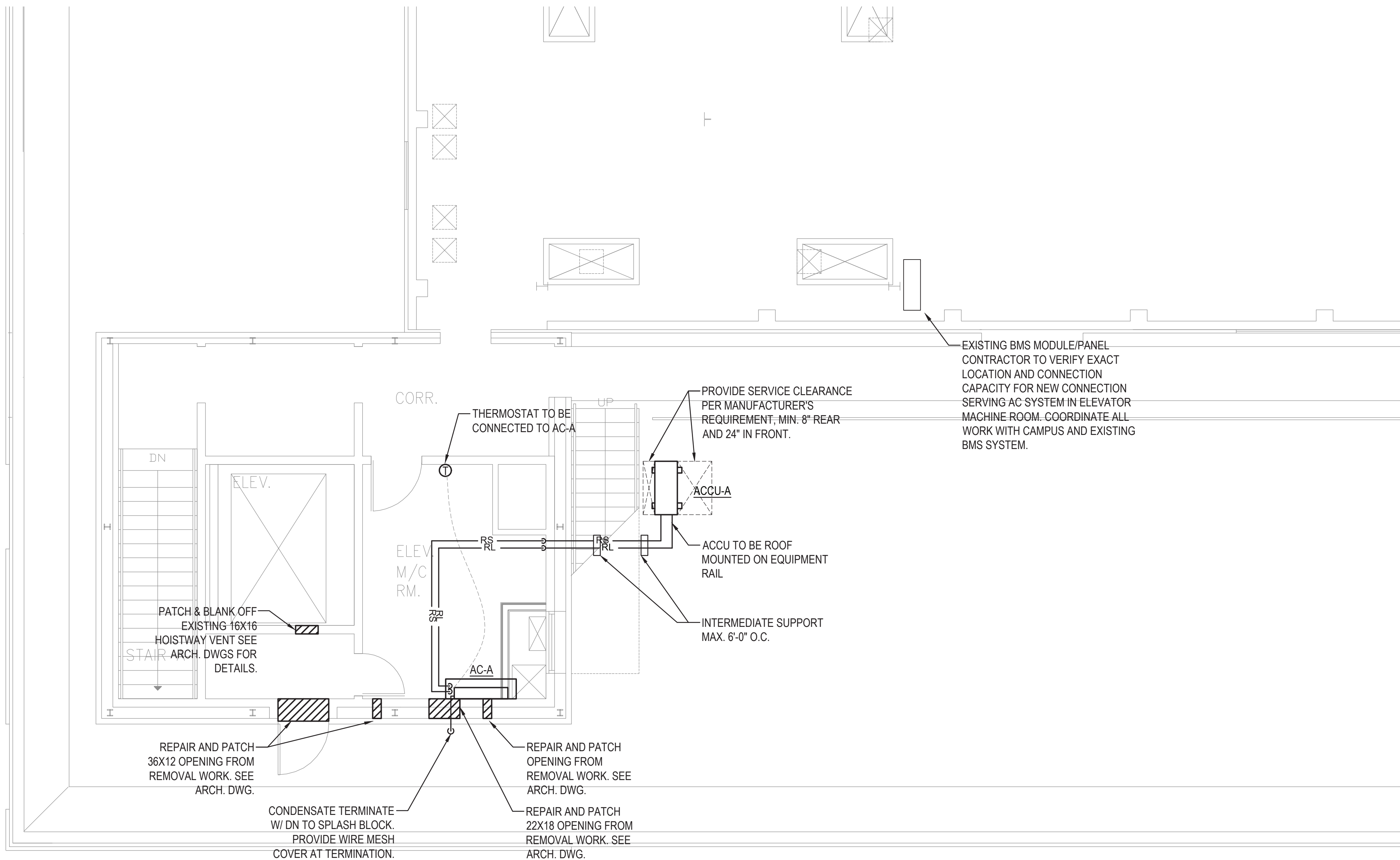
2 HVAC - COYKENDALL SCIENCE BUILDING PENTHOUSE PART PLAN SCALE: 1/4"=1'-0"
