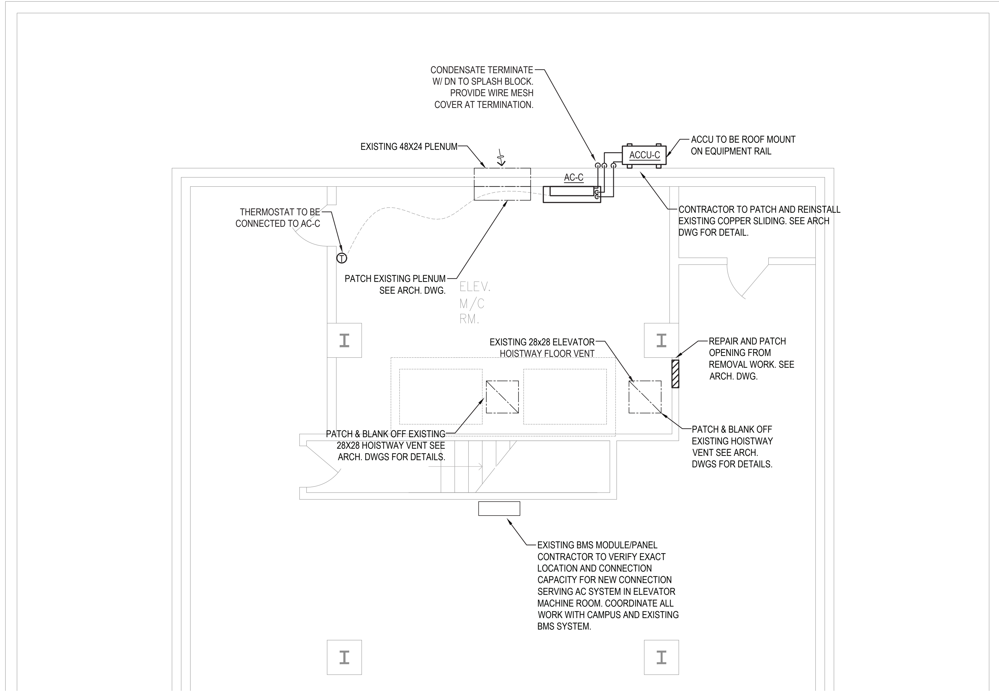
2 HVAC - HAGGERTY ADMINISTRATION BUILDING PENTHOUSE PART PLAN SCALE: 1/4"=1'-0"
