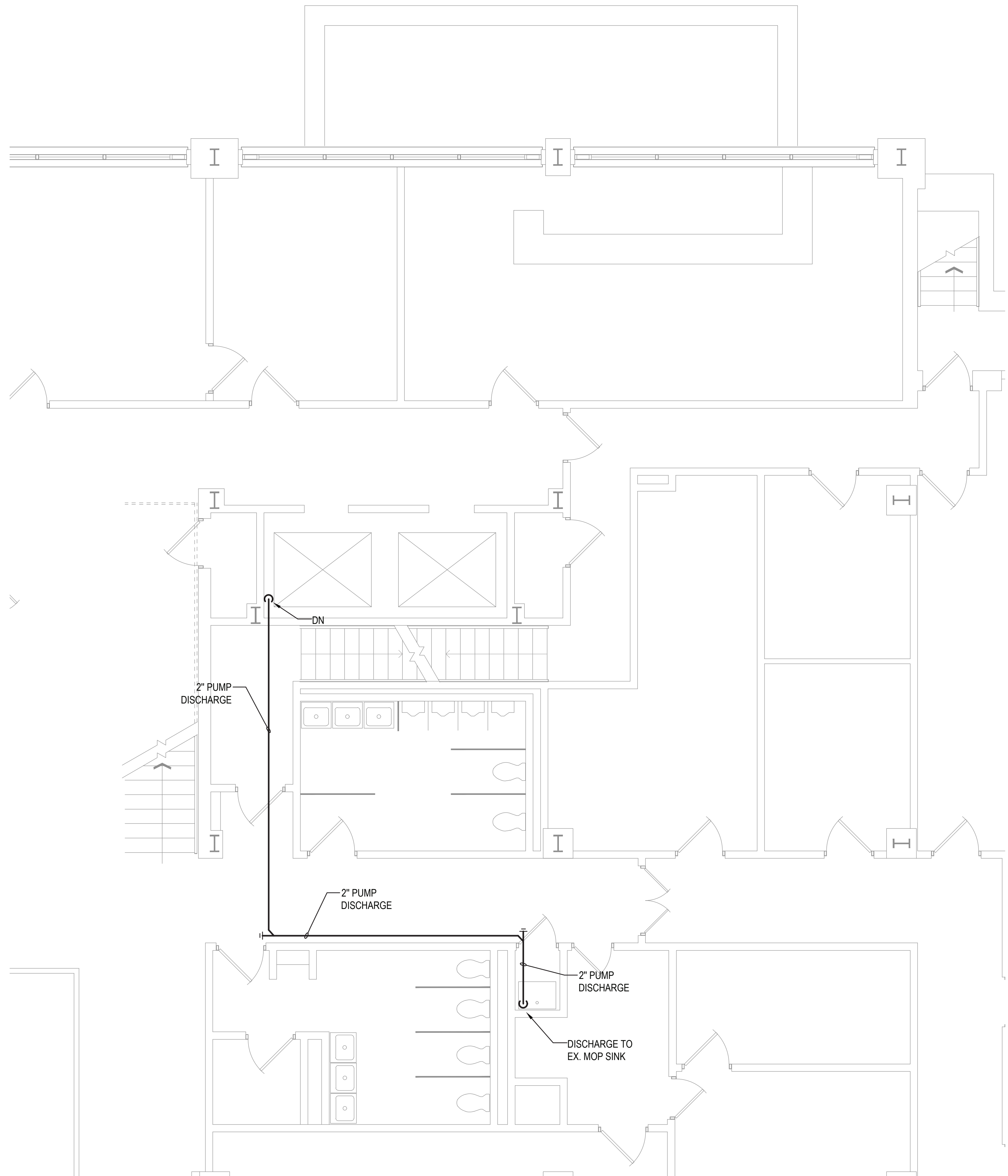
2 PLUMBING - HAGGERTY ADMINISTRATION BUILDING BASEMENT PART PLAN SCALE: 1/4"=1'-0"
