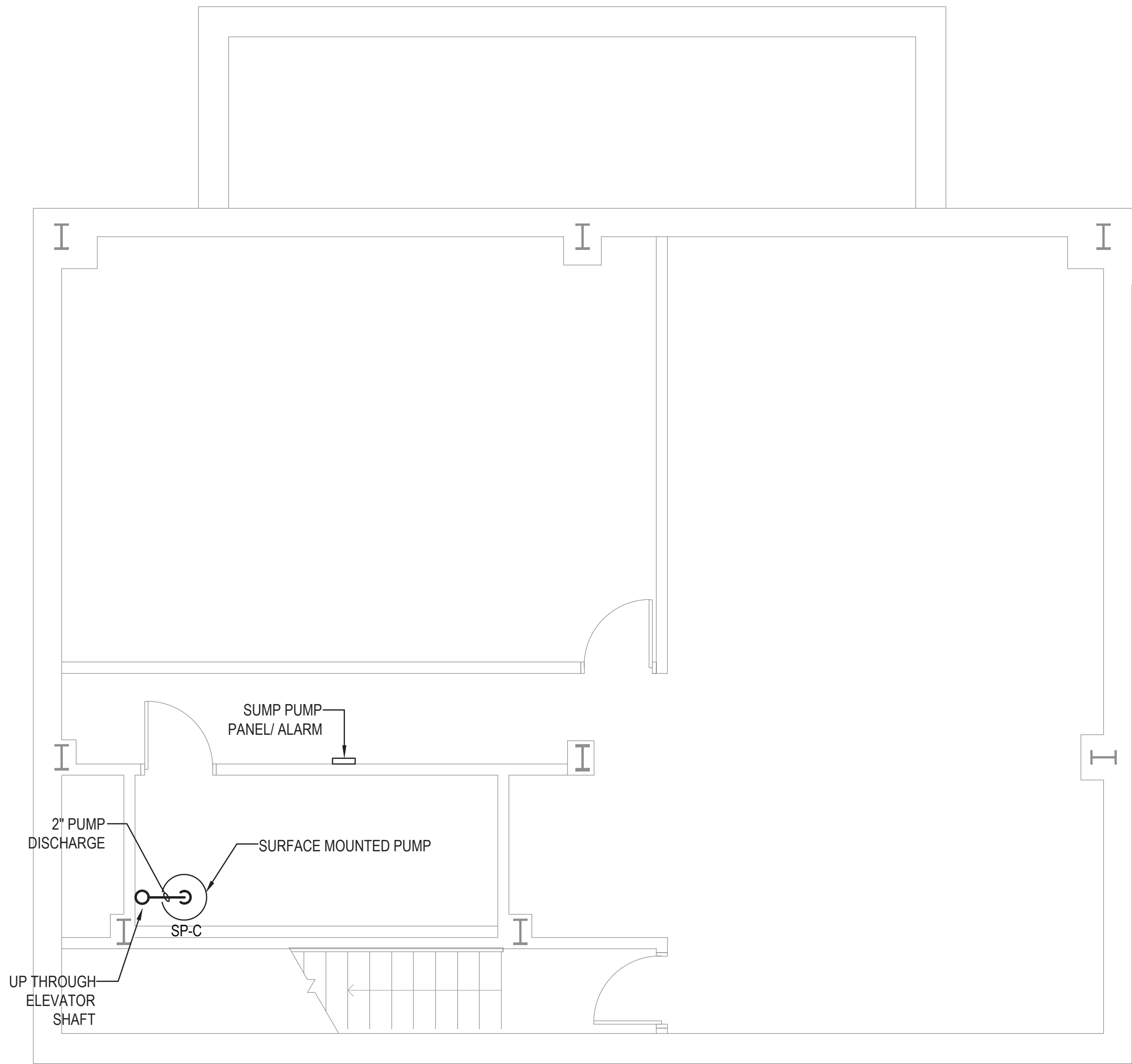
1 PLUMBING - HAGGERTY ADMINISTRATION BUILDING BASEMENT PART PLAN SCALE: 1/4"=1'-0"
