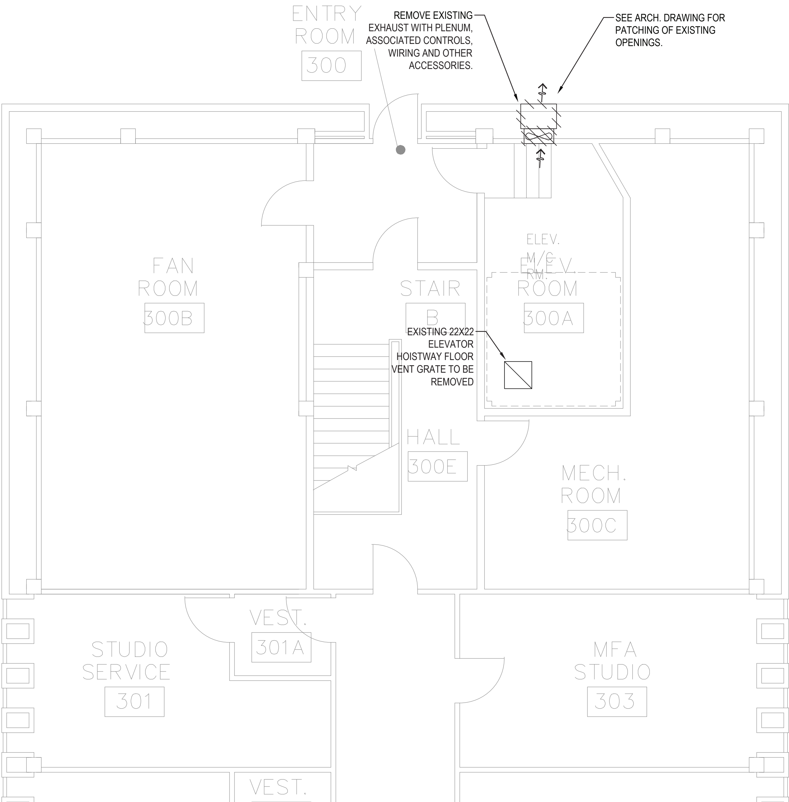
2 HVAC - SMILEY ART BUILDING THIRD FLOOR PART PLAN SCALE: 1/4"=1'-0"
