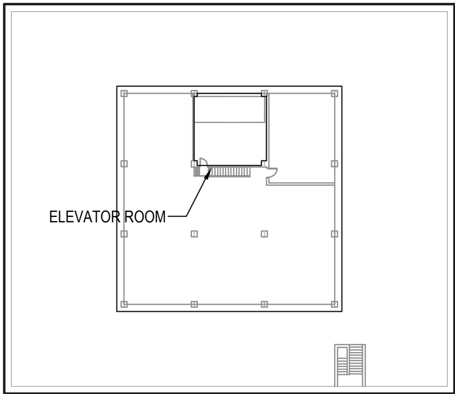
1 STUDENT UNION BUILDING PENTHOUSE ELEVATOR ROOM PART PLAN SCALE: 1/32"=1'-0"
