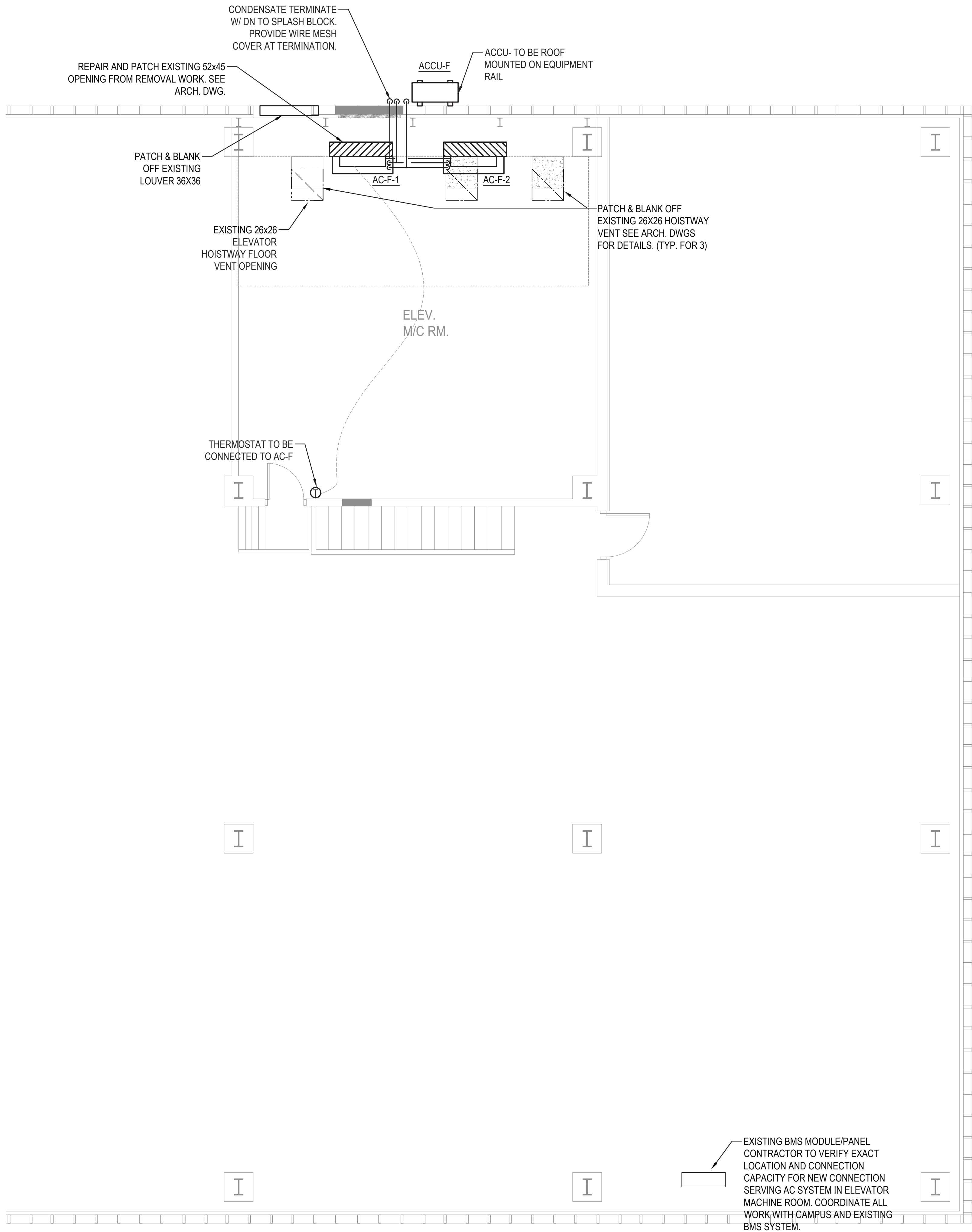
2 HVAC - STUDENT UNION BUILDING PENTHOUSE PART PLAN SCALE: 1/4"=1'-0"
