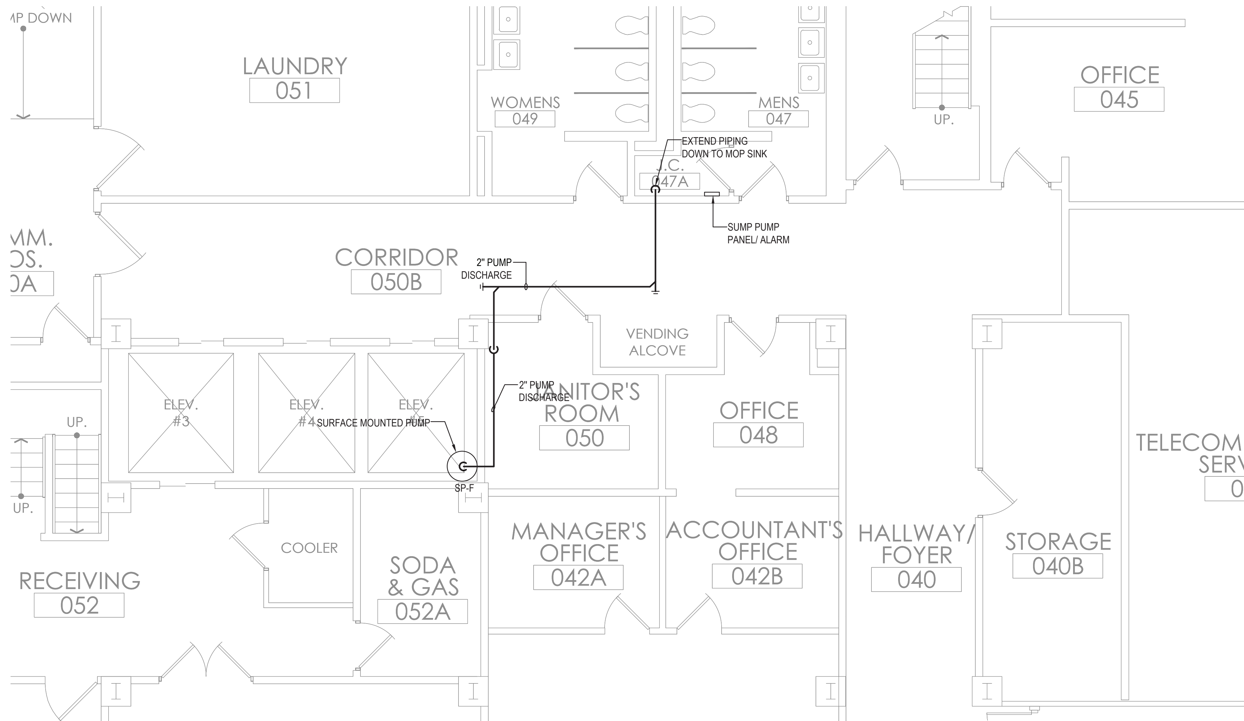
2 PLUMBING - STUDENT UNION BUILDING SOUTH END LOWER LEVEL PART PLAN SCALE: 1/4"=1'-0"
