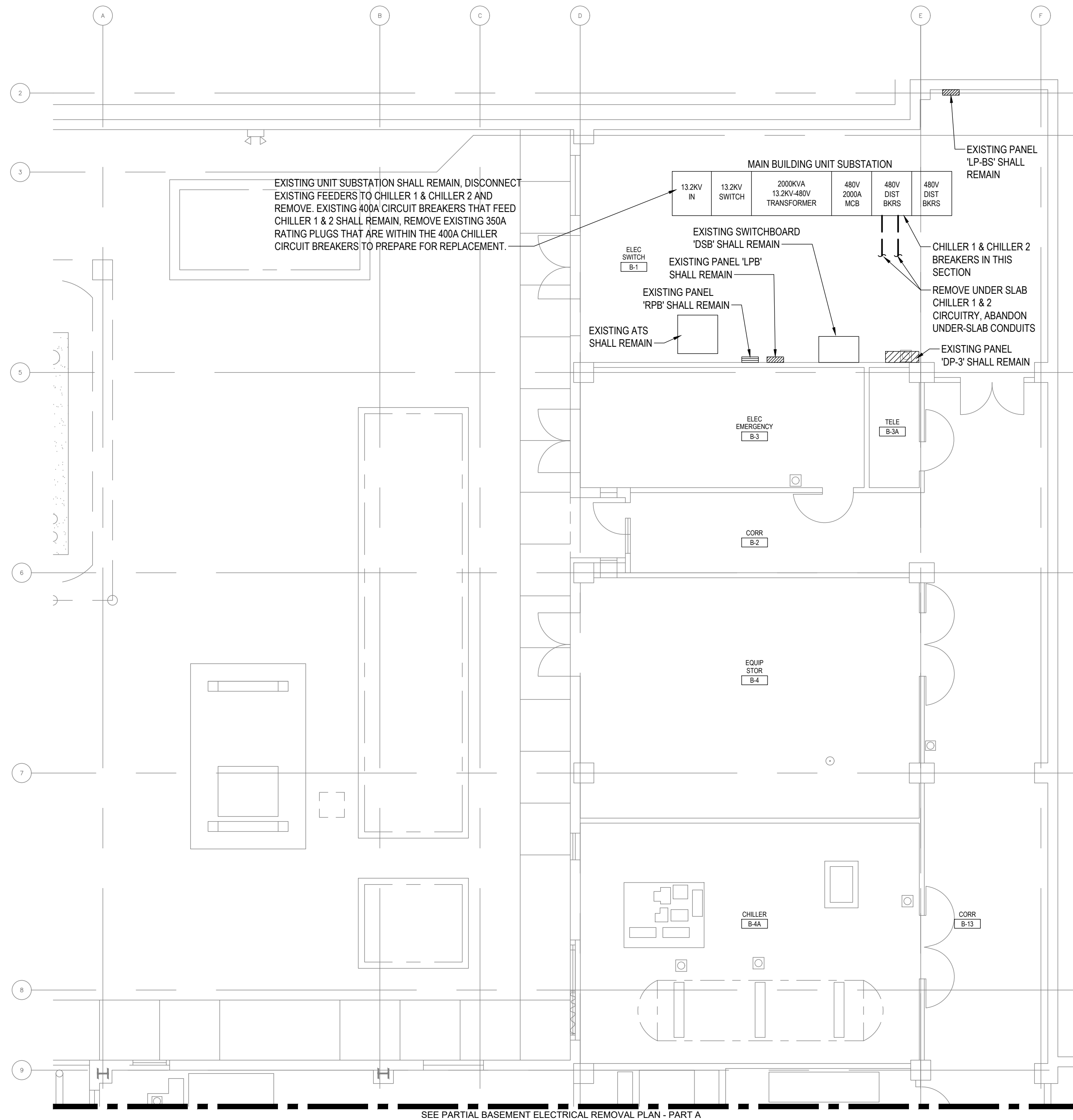
2 PARTIAL BASEMENT ELECTRICAL REMOVAL PLAN - PART B SCALE: 1/8" = 1'-0"
