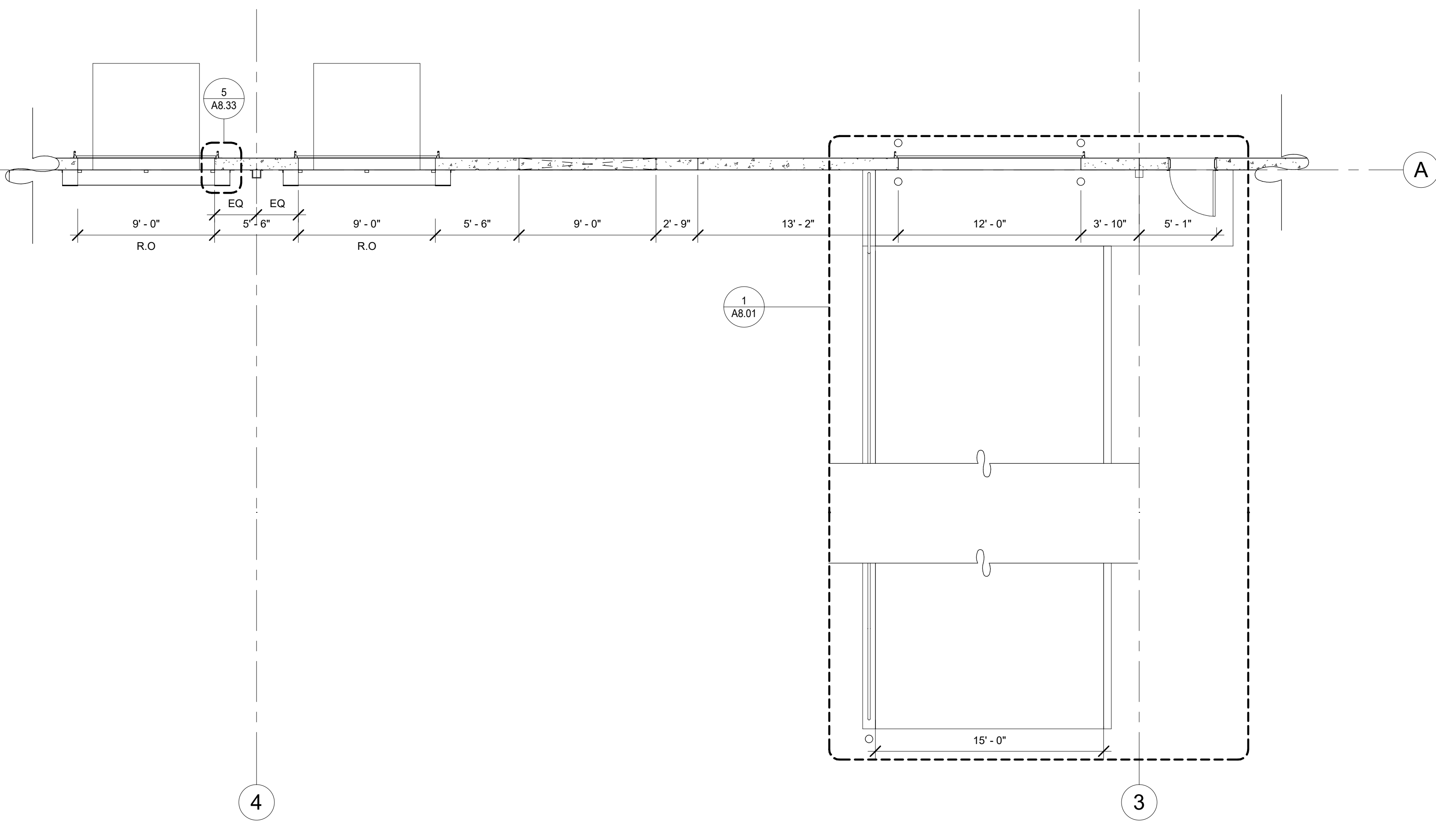
ENLARGED FLOOR PLAN - DOCK WALL
