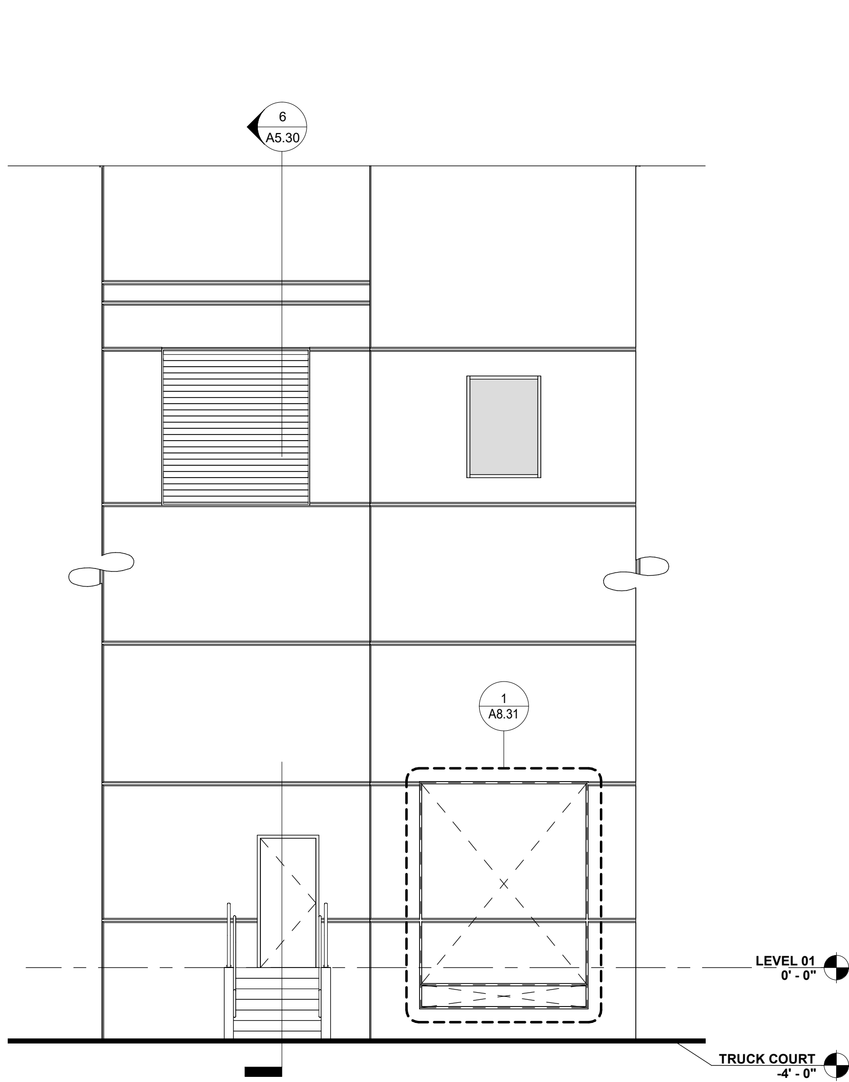
ENLARGED ELEVATION - LOUVER
