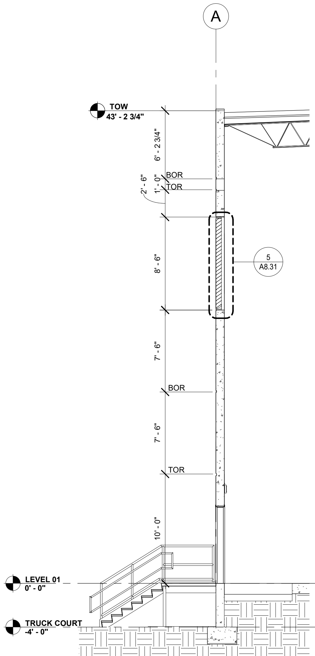
SECTION @ LOUVER
