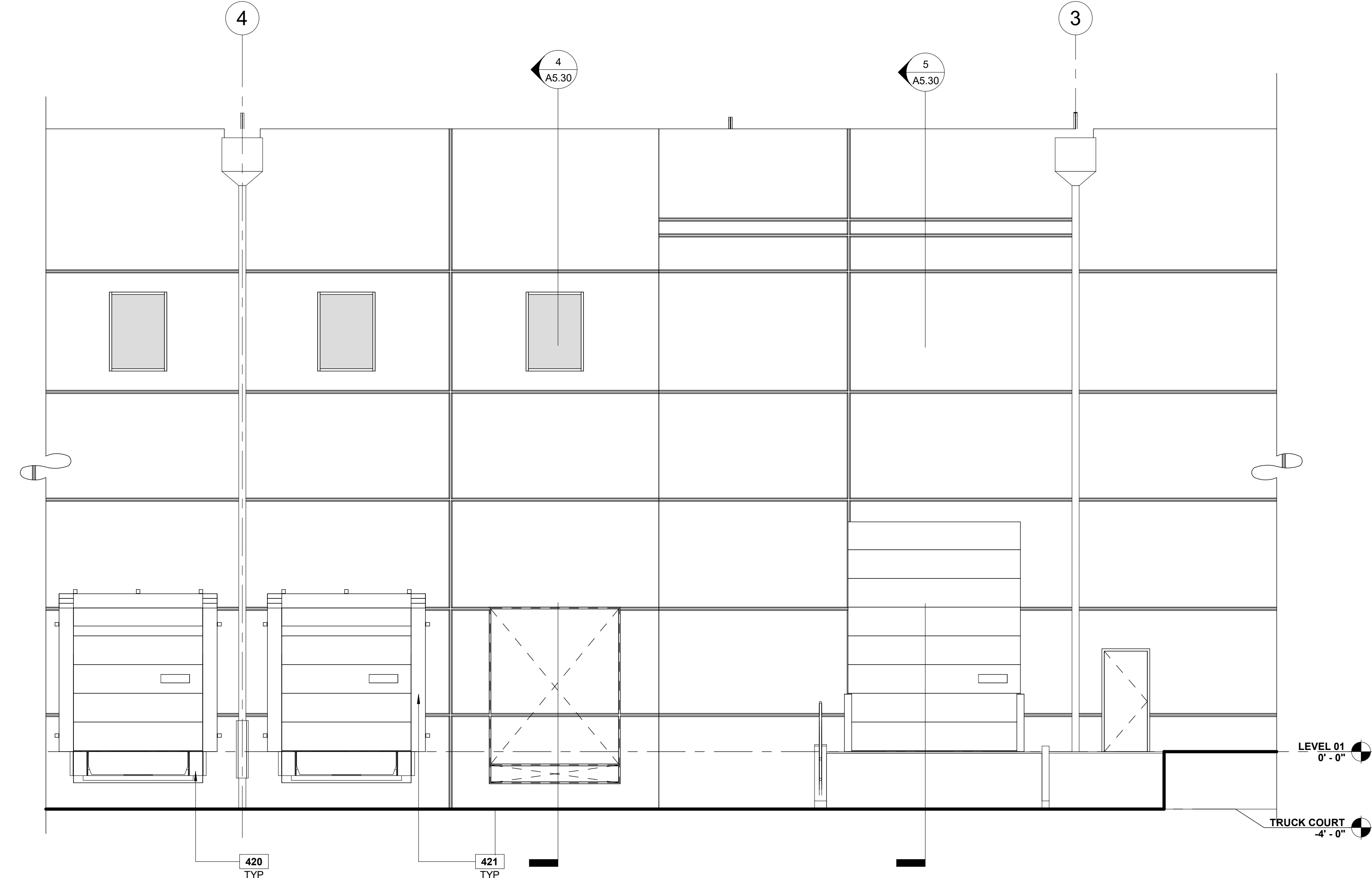
ENLARGED ELEVATION - DOCK WALL
