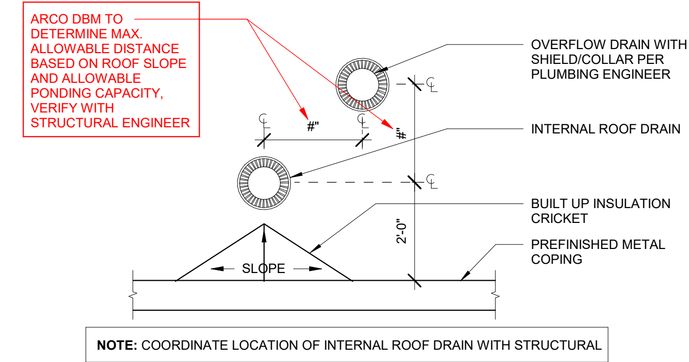
INTERIOR ROOF DRAIN LEADER GUARD SCALE: 1 1/2" = 1'-0"
