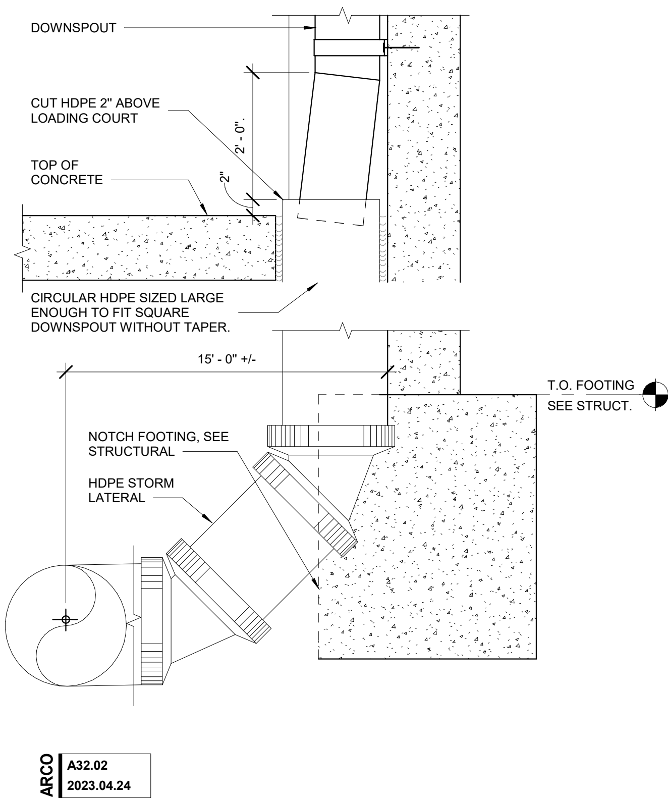
DOWNSPOUT SECTION AT FOOTING SCALE: 1" = 1'-0"
