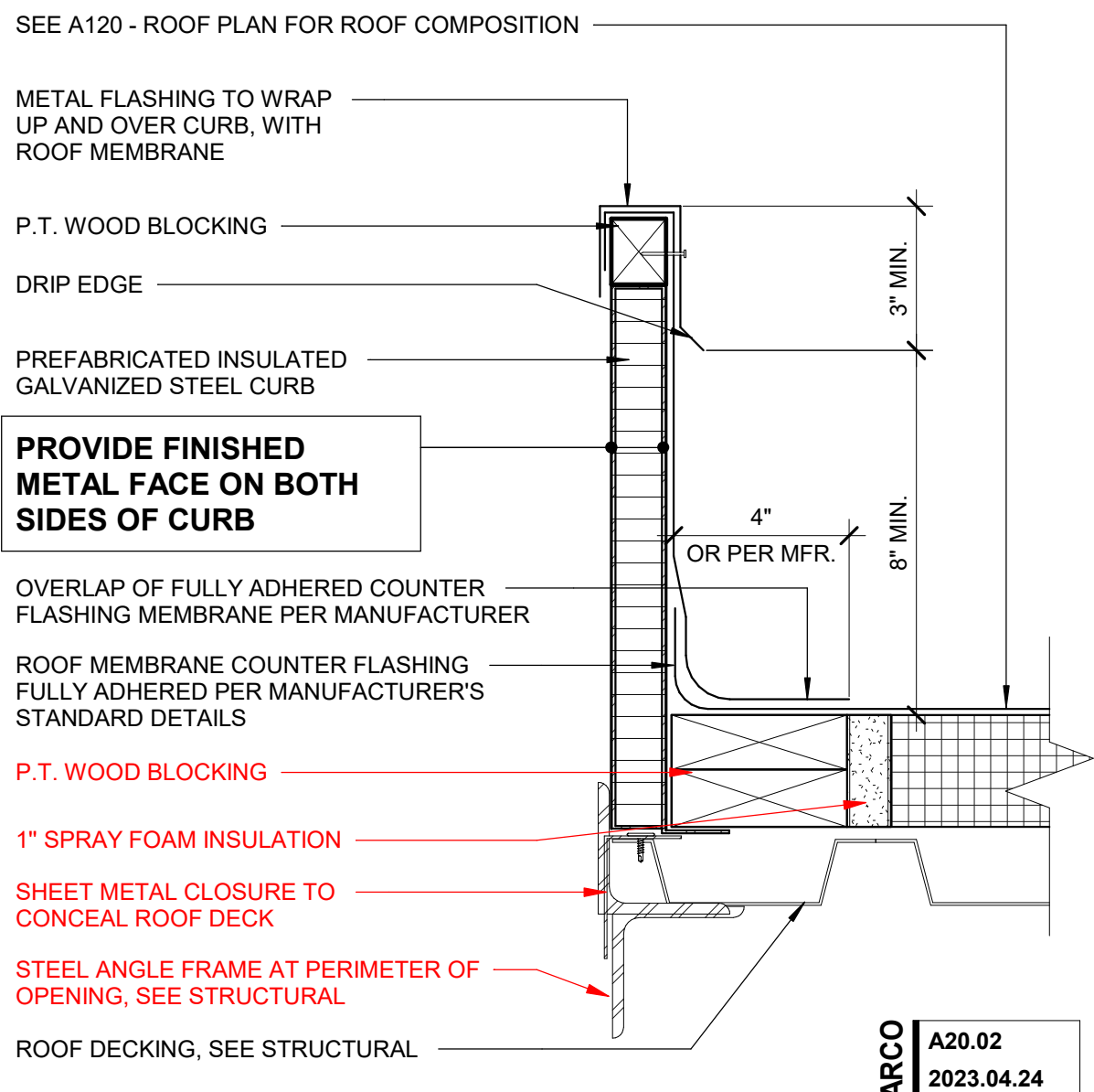
ROOF MECHANICAL CURB SCALE: 3" = 1'-0"
