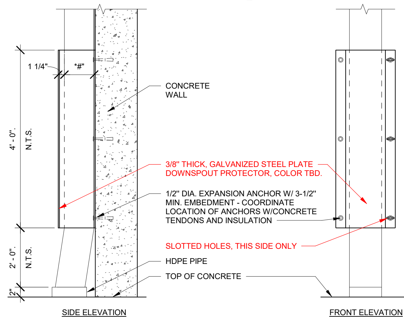
DOWNSPOUT GUARD - SINGLE SCALE: 1" = 1'-0"
