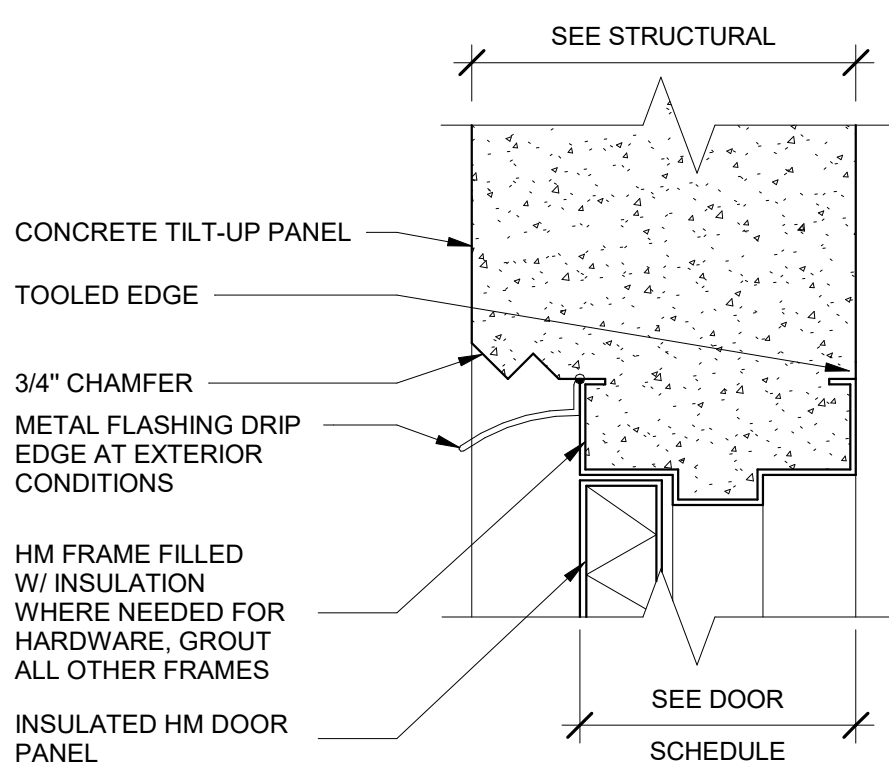
HM HEAD AT TILT
