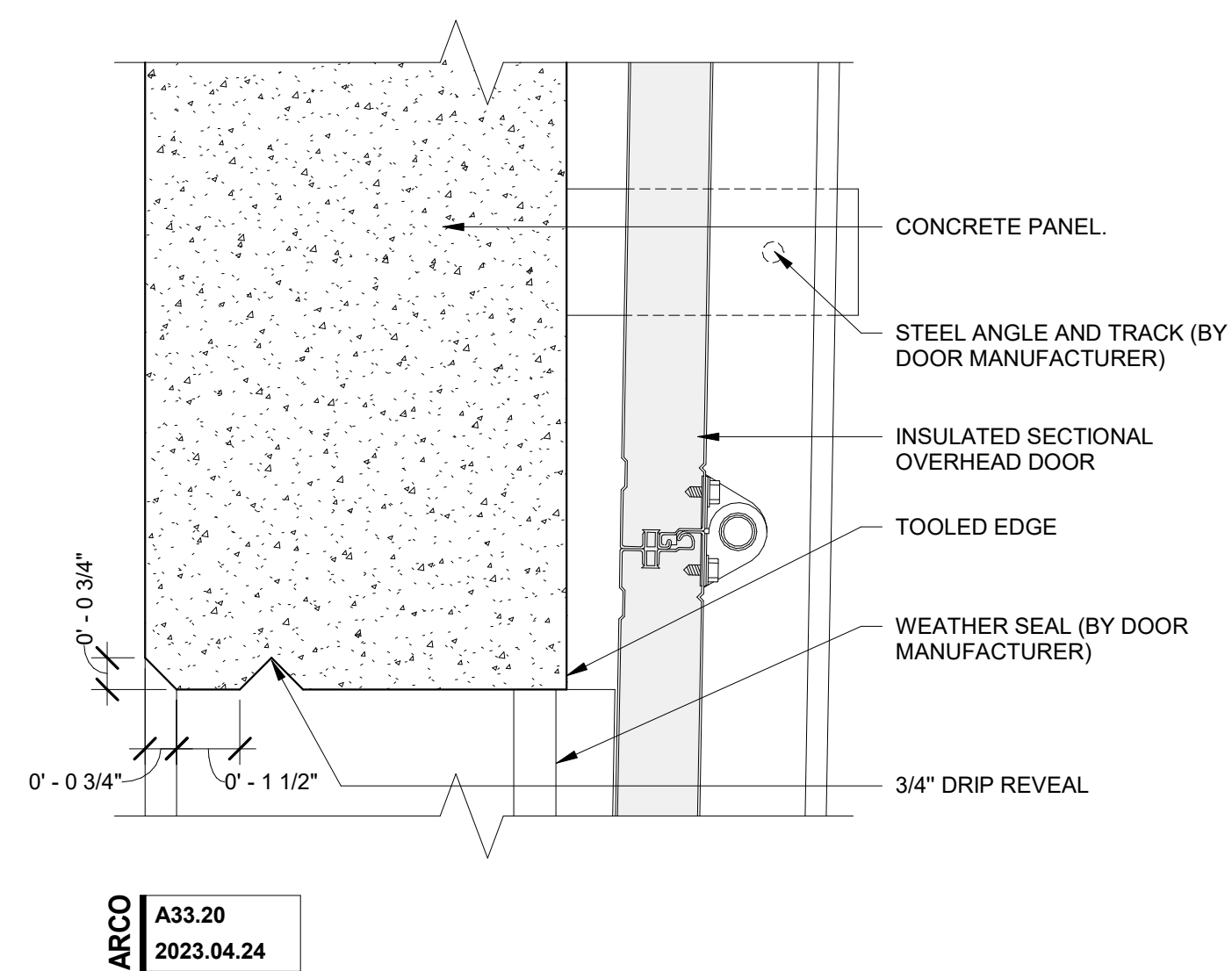
SECTION DOOR HEAD
