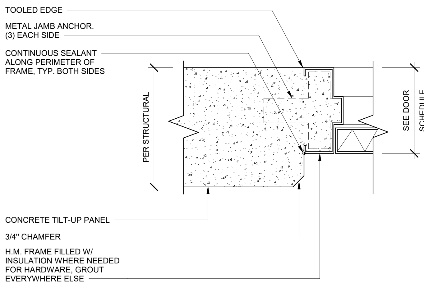
HM JAMB AT TILT
