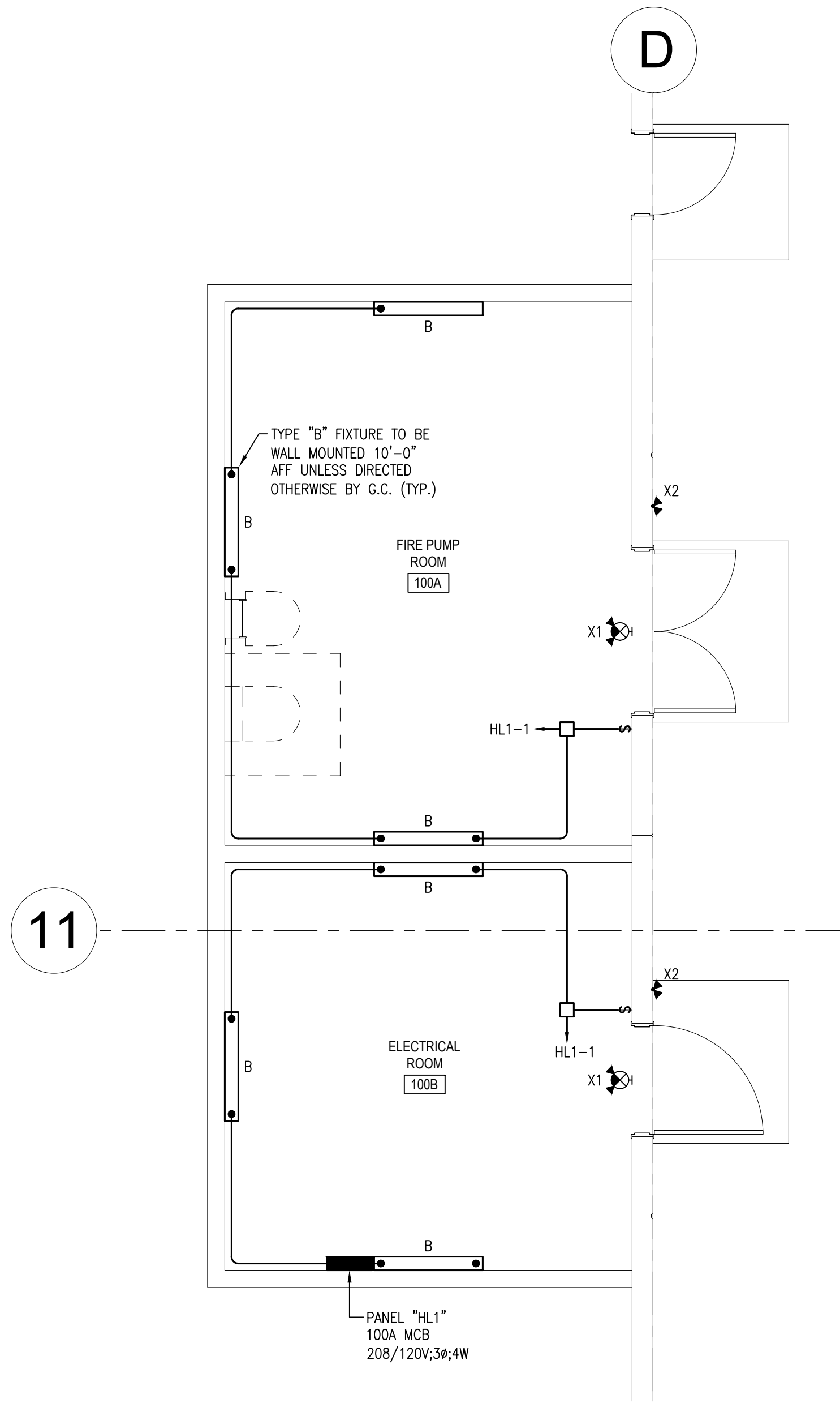
1 ENLARGED LIGHTING PLAN E4.0 SCALE: 1/4" = 1'-0"
