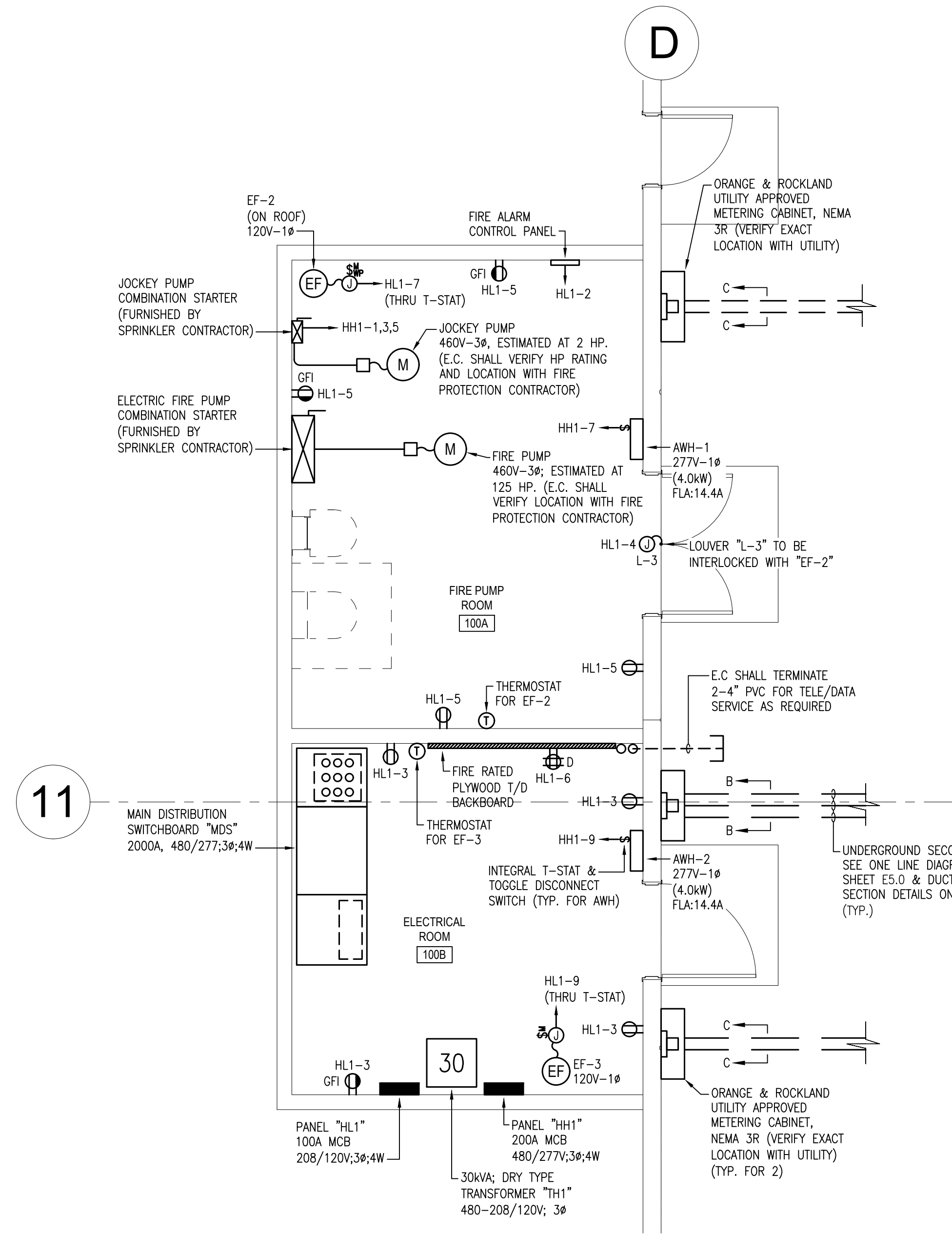
2 ENLARGED POWER PLAN E4.0 SCALE: 1/4" = 1'-0"
