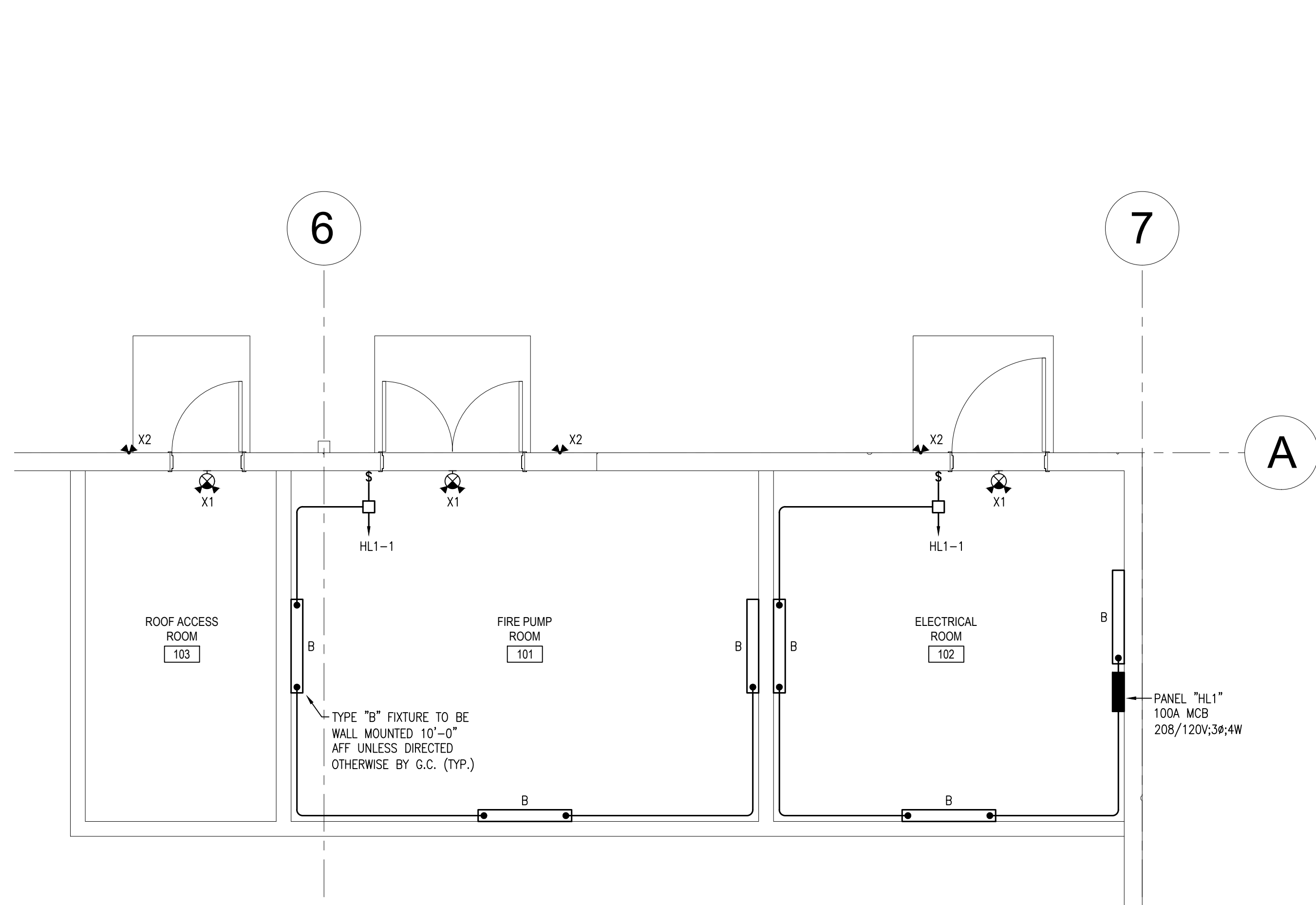
1 E4.0 ENLARGED LIGHTING PLAN SCALE: 1/4" = 1'-0"
