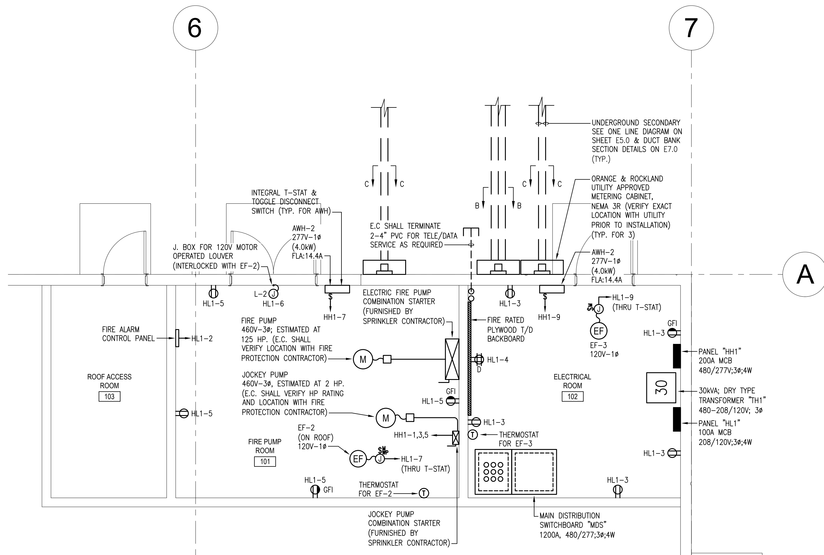
2 E4.0 ENLARGED POWER PLAN SCALE: 1/4" = 1'-0"
