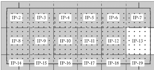
1 IMPACT PIER ELEMENT LAYOUT - PLAN VIEW - BUILDING 1
