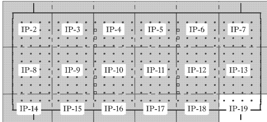
1 IMPACT PIER ELEMENT LAYOUT - PLAN VIEW - BUILDING 1
