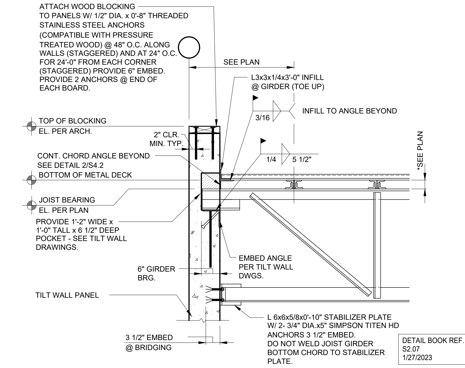
3 S4.1 JOIST GIRDER BEARING ON TILT WALL PANEL WITH PARAPET
