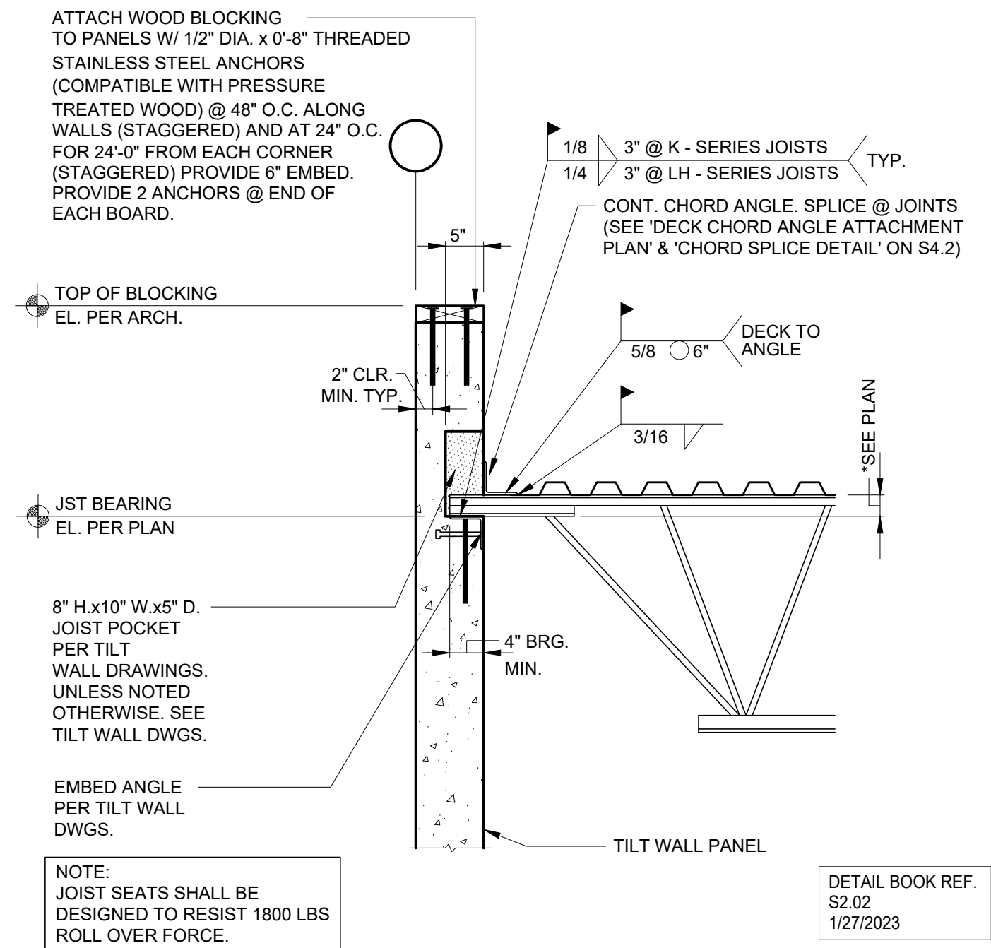
1 S4.1 BAR JOIST BEARING ON TILT WALL PANEL WITH PARAPET
