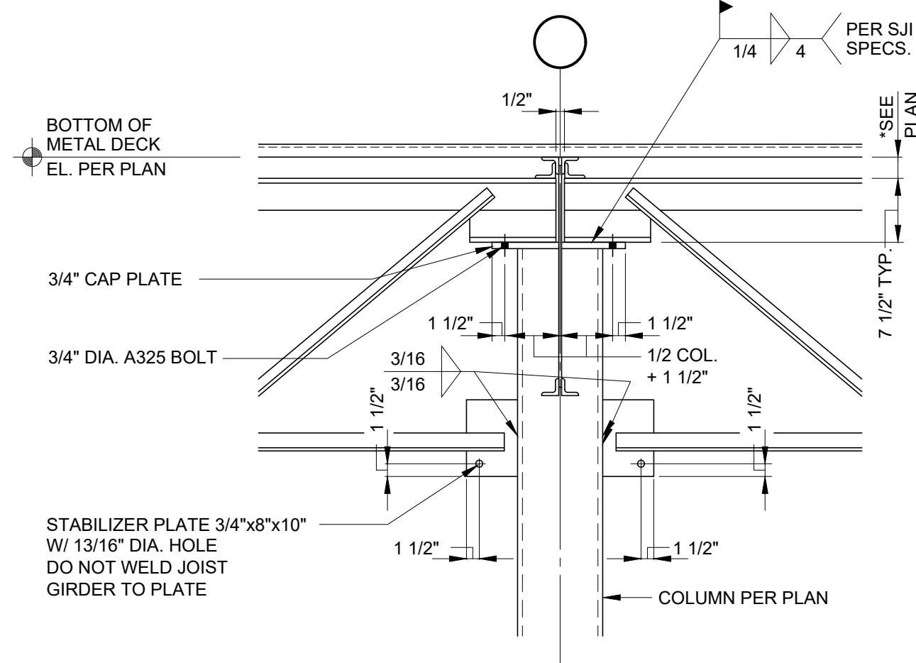
4 S4.1 JOIST GIRDER TO COLUMN CONNECTION
