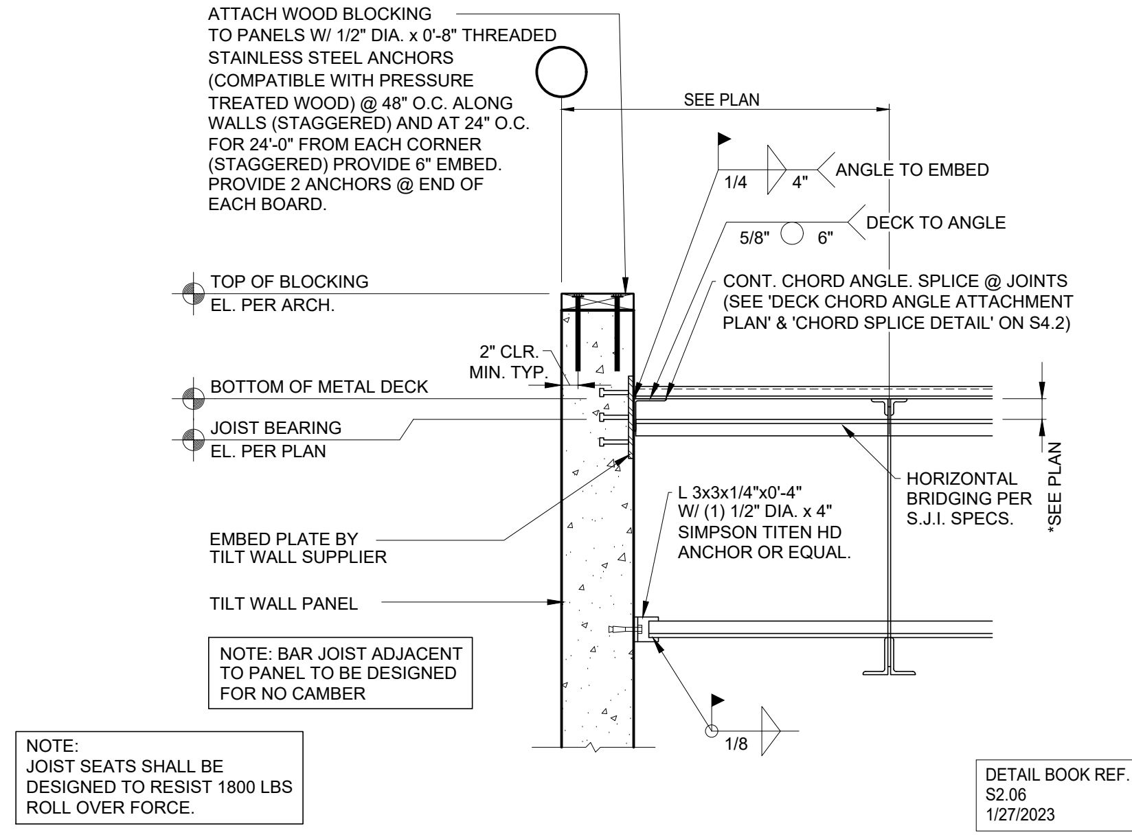
2 S4.1 DECK SUPPORT AT TILT WALL PANEL WITH PARAPET
