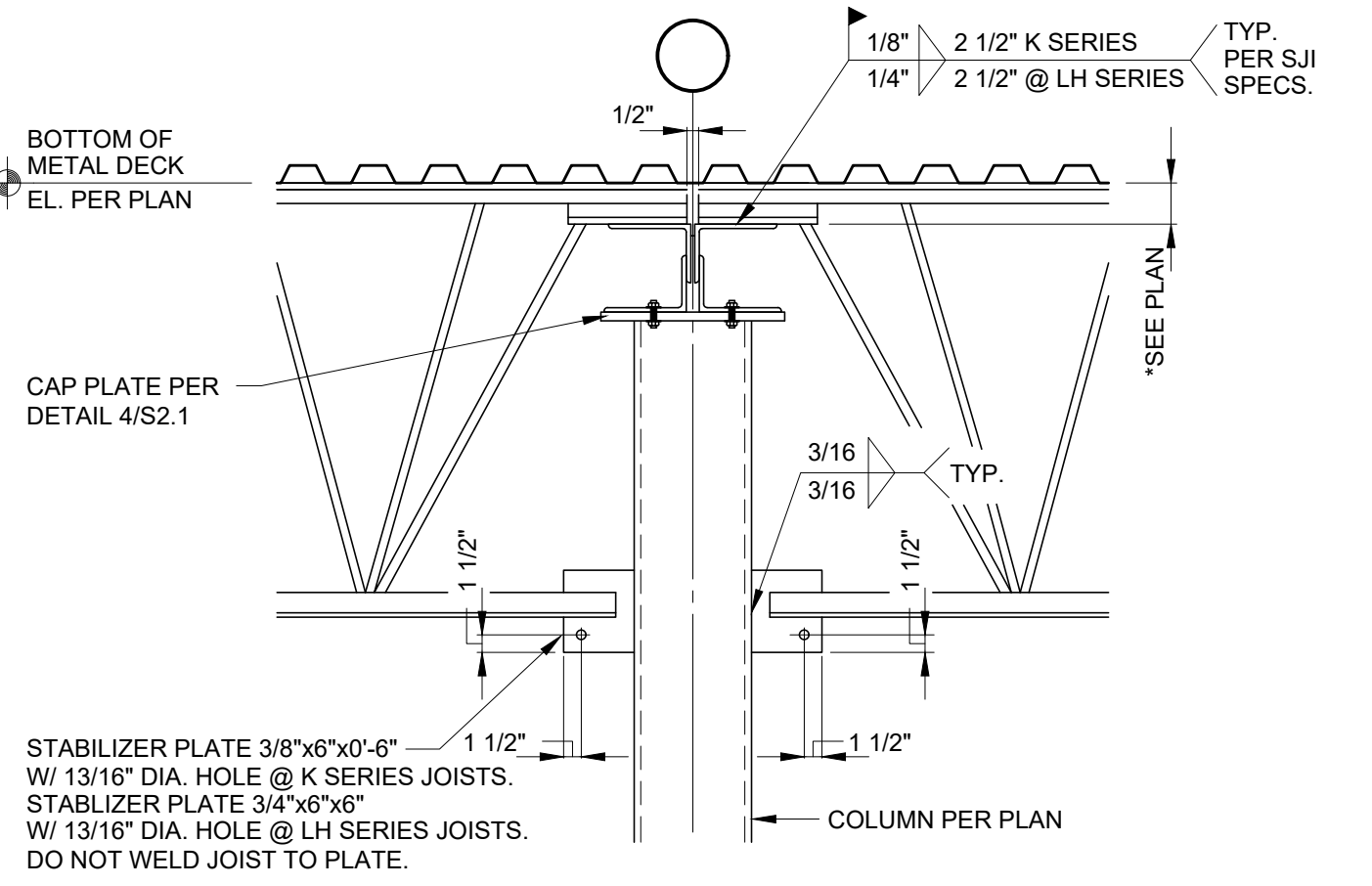
5 S4.1 JOIST TO COLUMN CONNECTION
