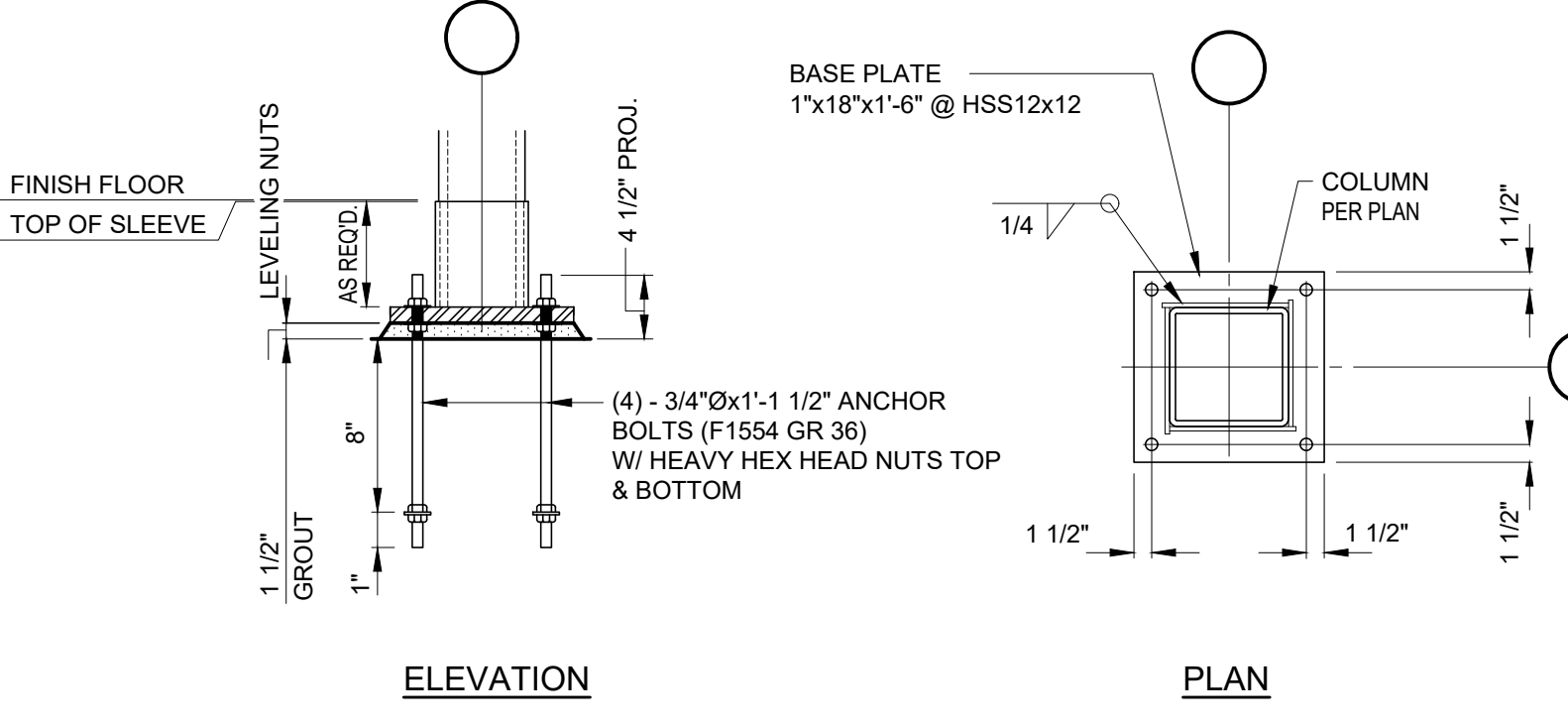
TYPICAL TUBE COLUMN BASE DETAIL W/SLEEVE
