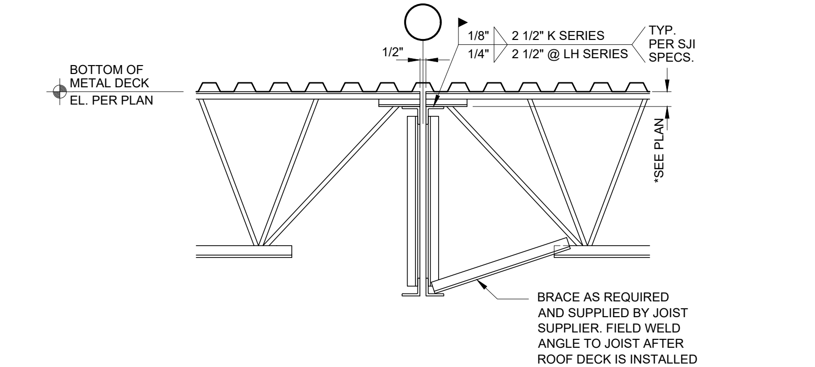
6 S4.1 JOIST TO GIRDER CONNECTION
