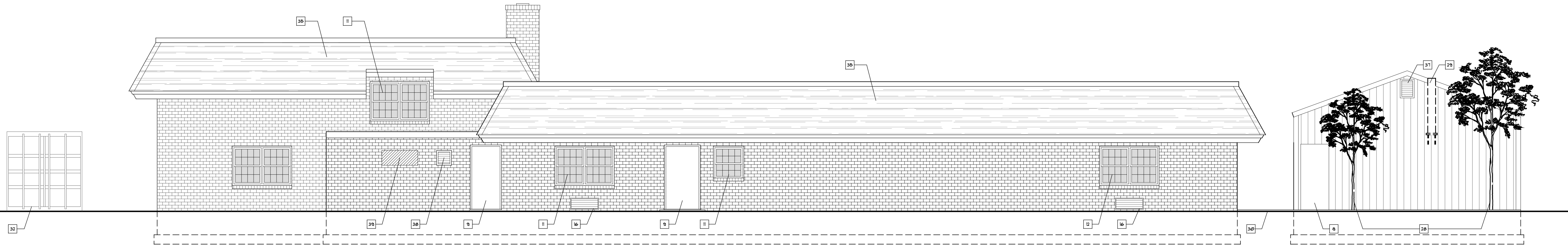
2 Existing East Demoliton Elevation AD2.01 Scale: 3/16" = 1'-0"
