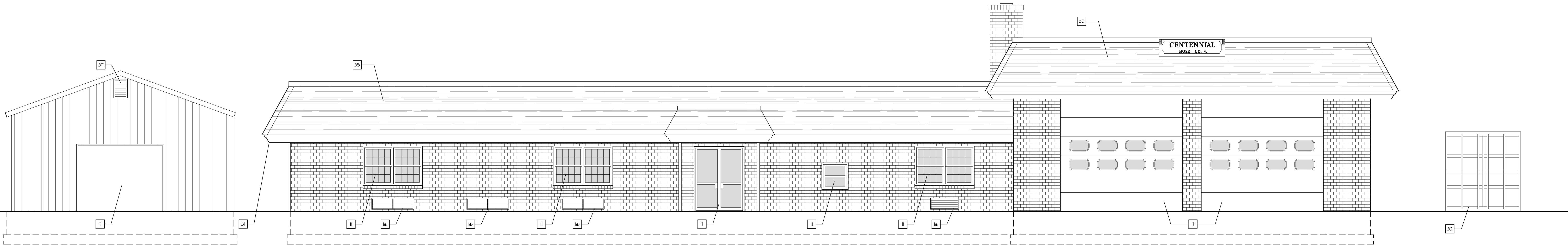
1 Existing West Demoliton Elevation AD2.01 Scale: 3/16" = 1'-0"
