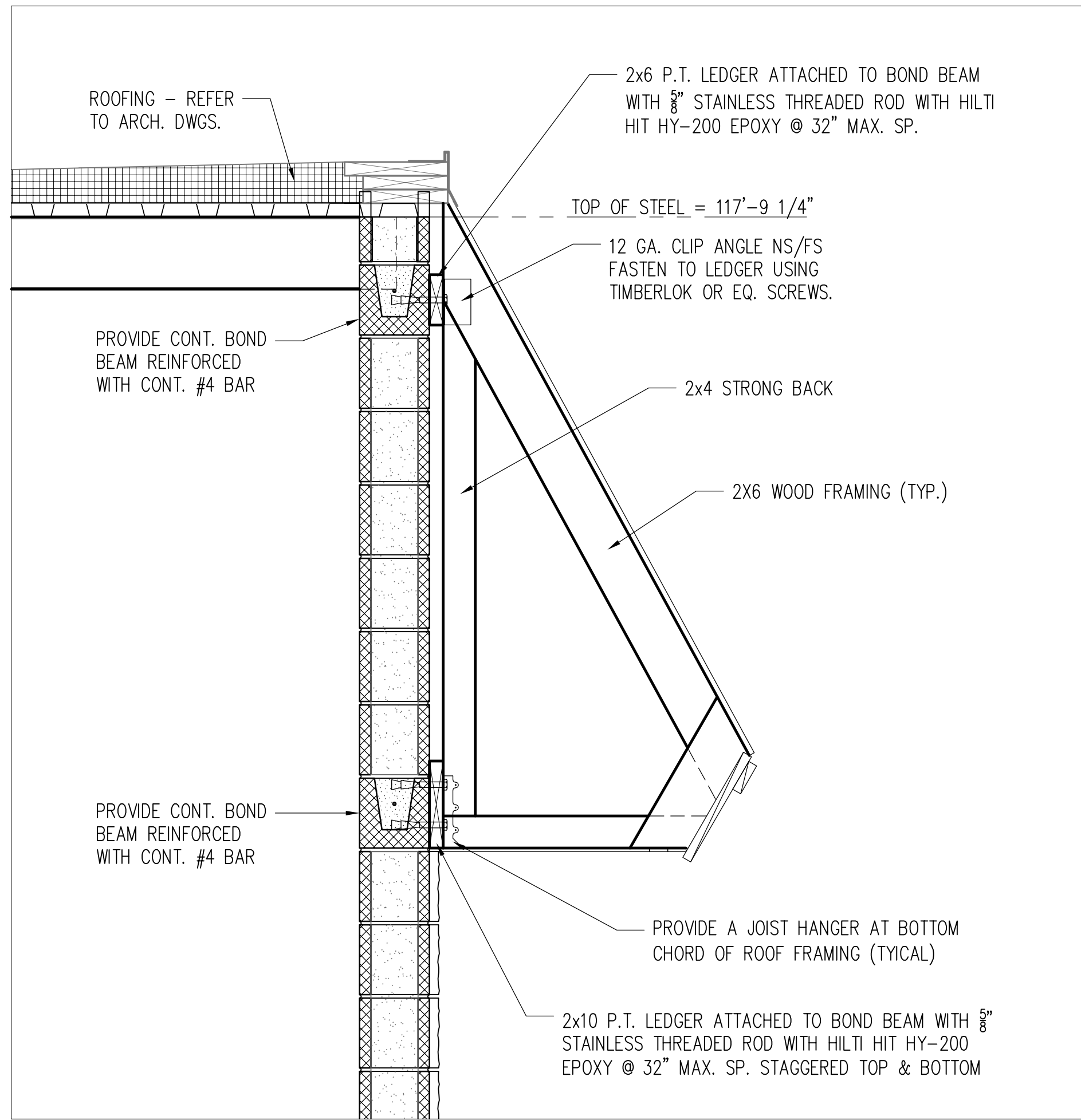
D.2 MANSARD ROOF FRAMING DETAIL S300 SCALE: 1" = 1'-0"
