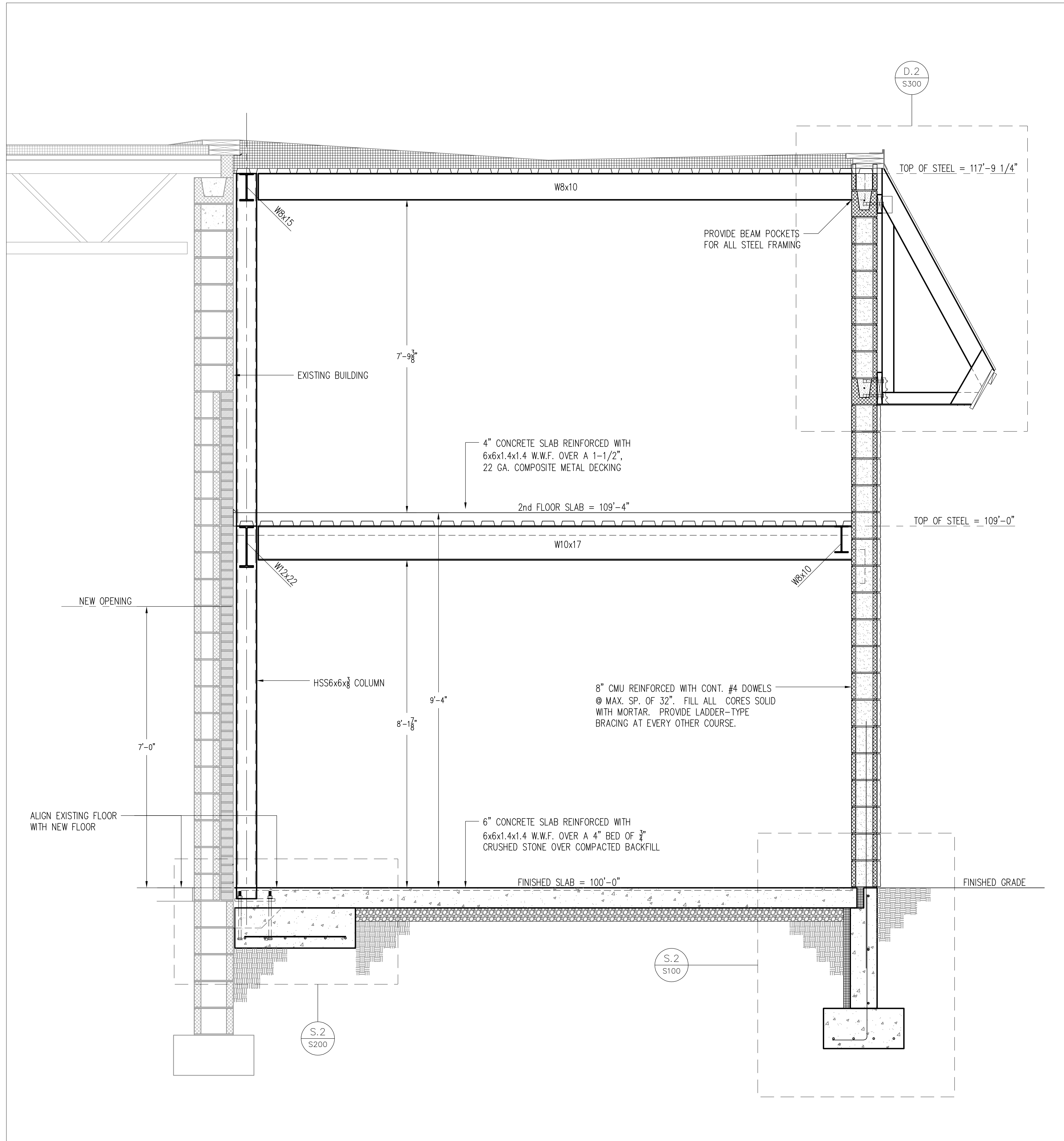
D.1 SECOND FLOOR FRAMING PLAN - TOP OF STEEL 108'-5" S200 SCALE: 1/8" = 1'-0"
