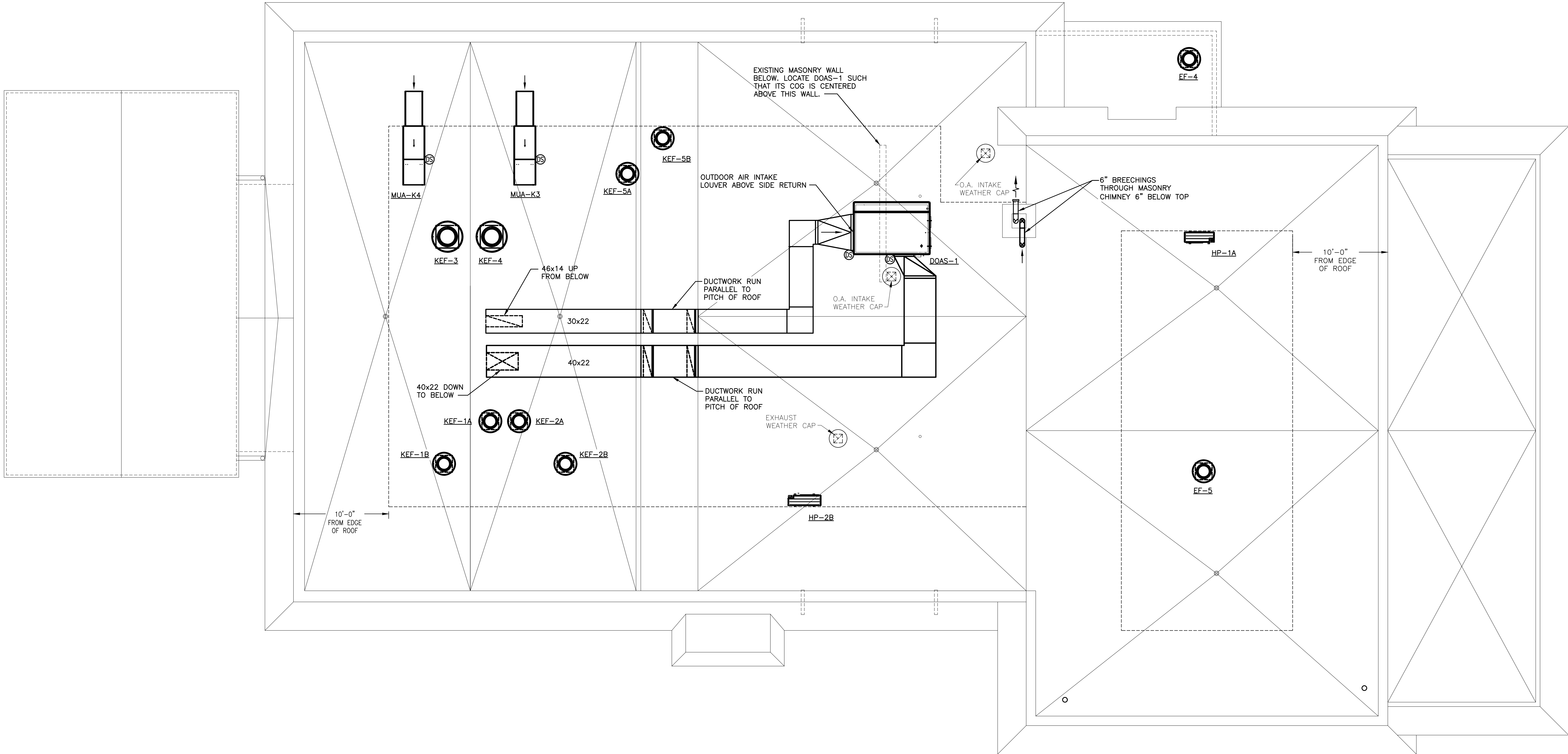
1 HVAC: CONSTRUCTION ROOF EQUIPMENT PLAN SCALE: 3/16"=1'-0"
