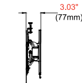
SIDE VIEW COLLAPSED
