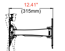
SIDE VIEW EXTENDED +15°/-5° TILT
