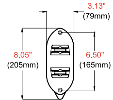
WALL PLATE DETAIL
