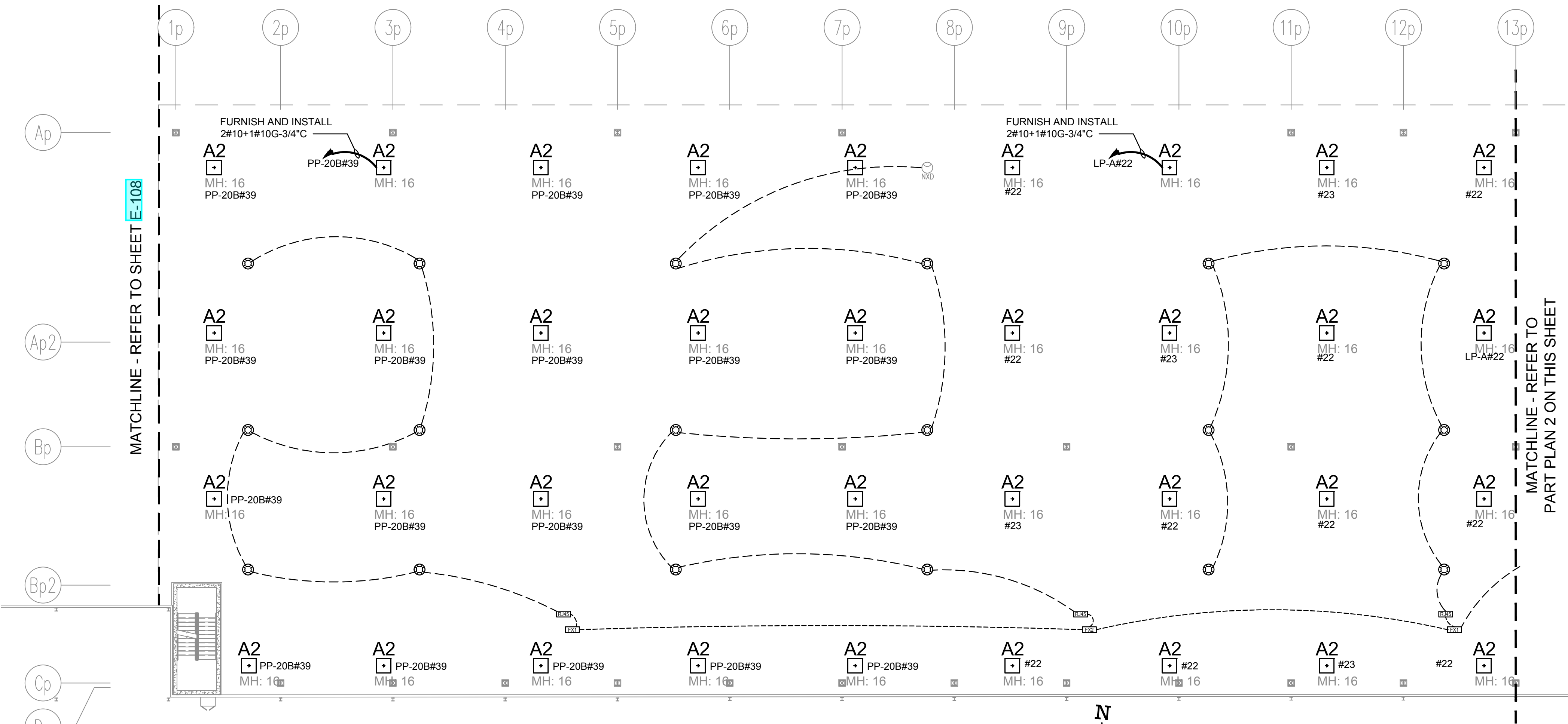
1 ELECTRICAL LIGHTING PLAN - PARKING DECK (WEST)
