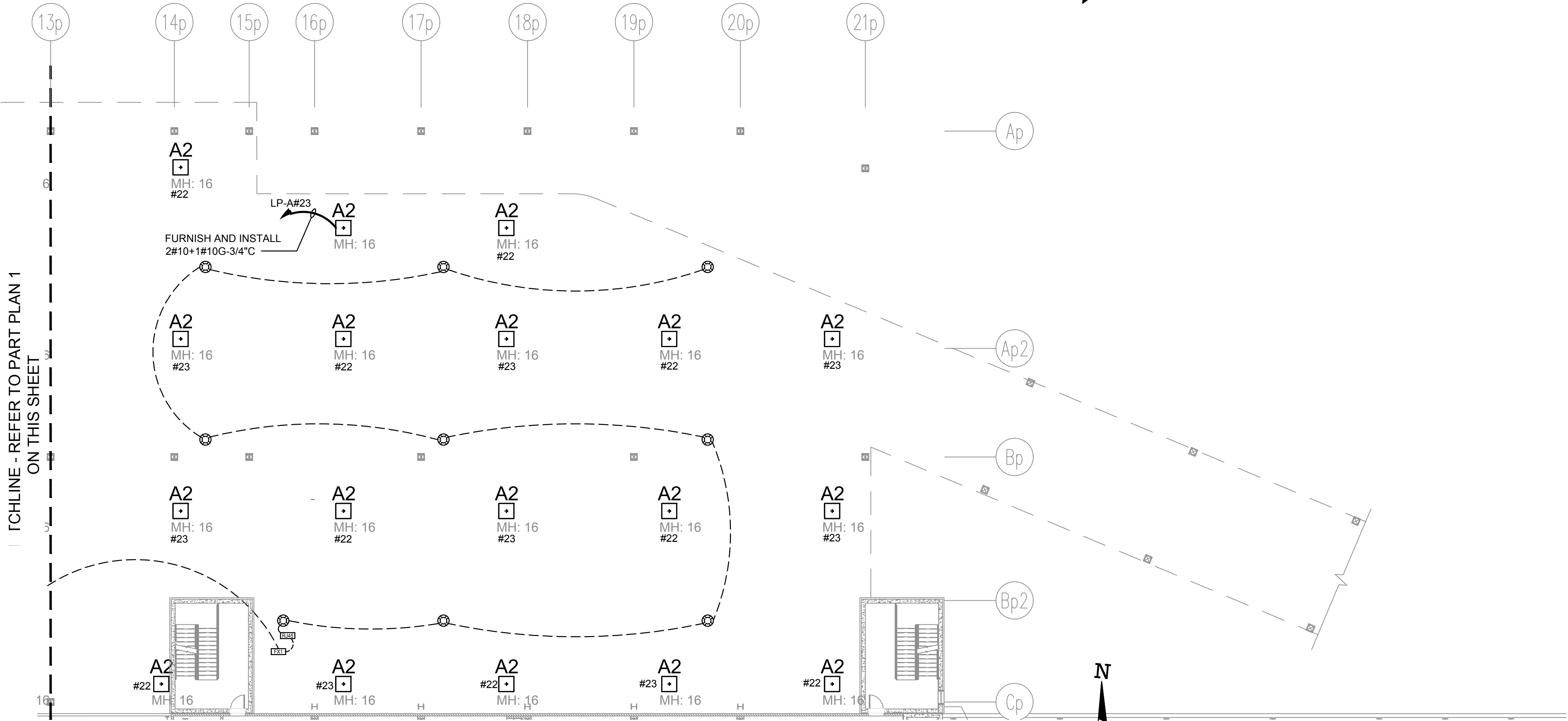
2 ELECTRICAL LIGHTING PLAN - PARKING DECK (EAST)
