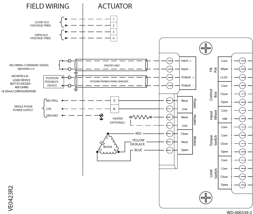
Figure 5. 120 Vac Modulating.
