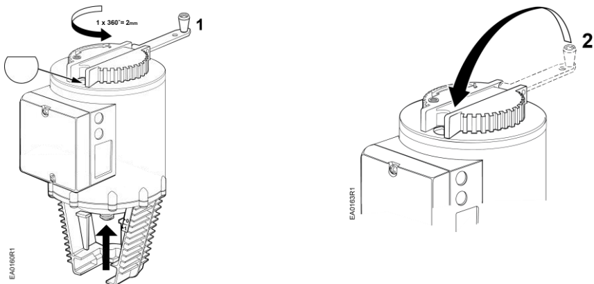
Figure 13. Automatic Operation.
