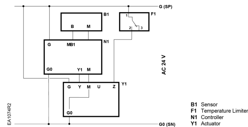
Figure 13. Connecting Terminals.
