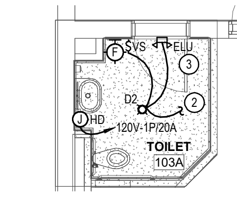
ENLARGED FIRST FLOOR BATHROOM PLAN
