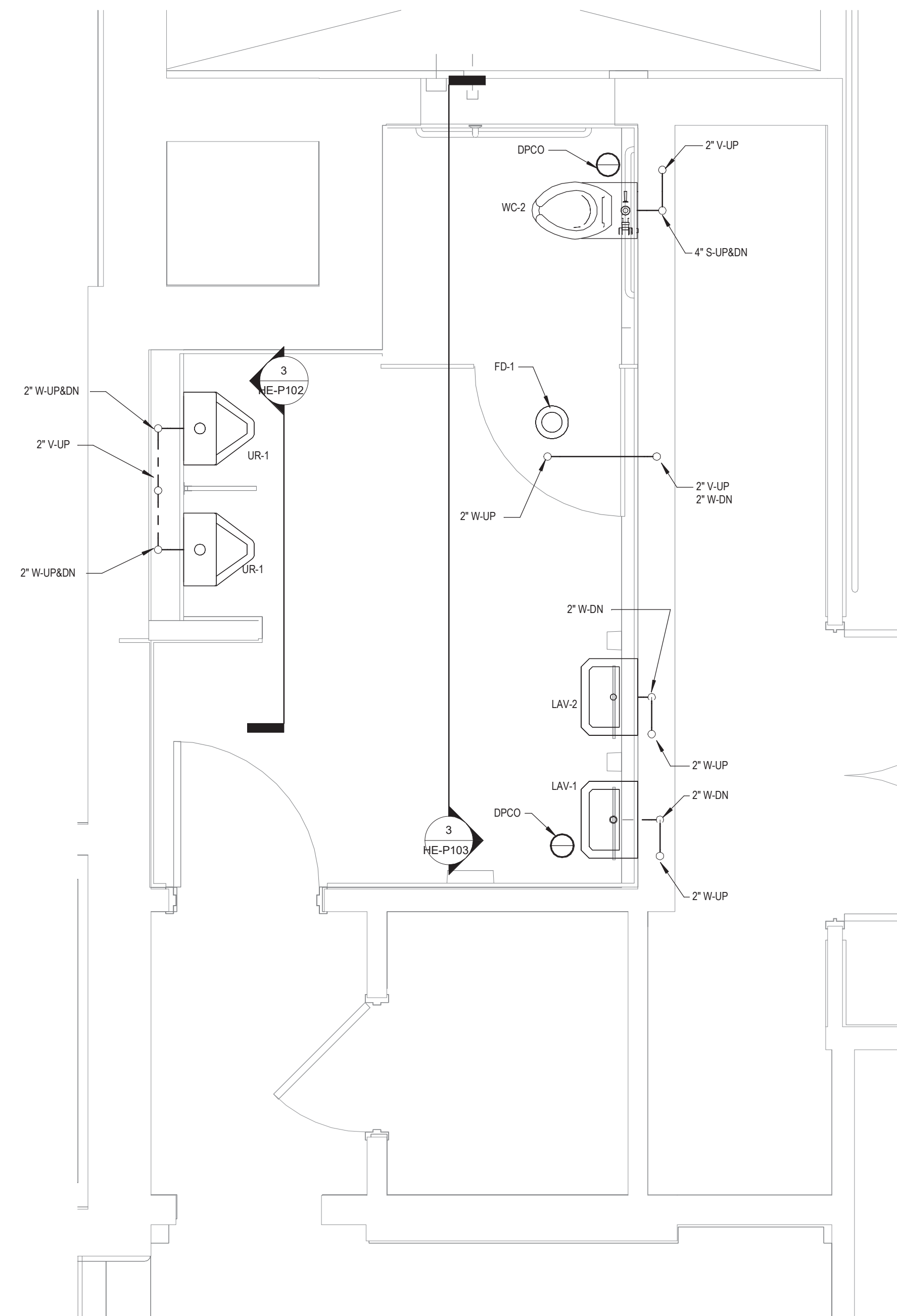
2 FIRST FLOOR BOYS BATHROOM SANITARY AND VENT INSTALLATION PLAN 1/2" = 1'-0"
