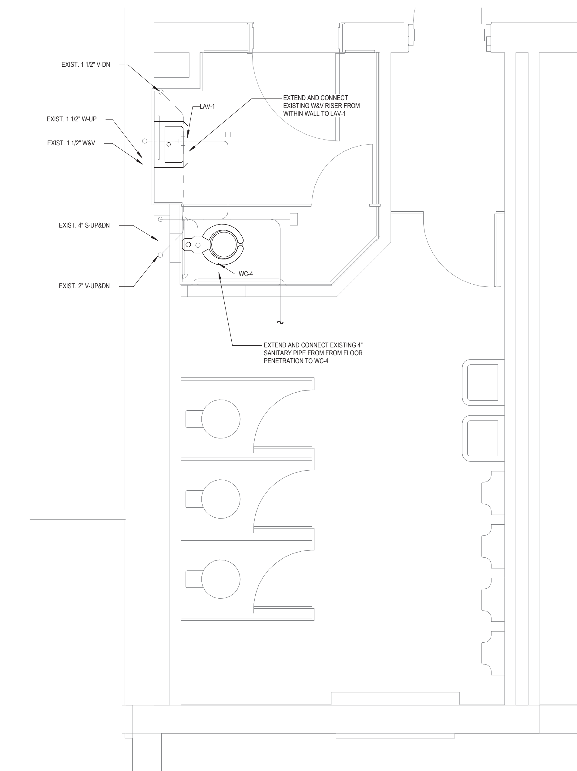
1 FIRST FLOOR TEACHER'S BATHROOM SANITARY AND VENT INSTALLATION PLAN 1/2" = 1'-0"
