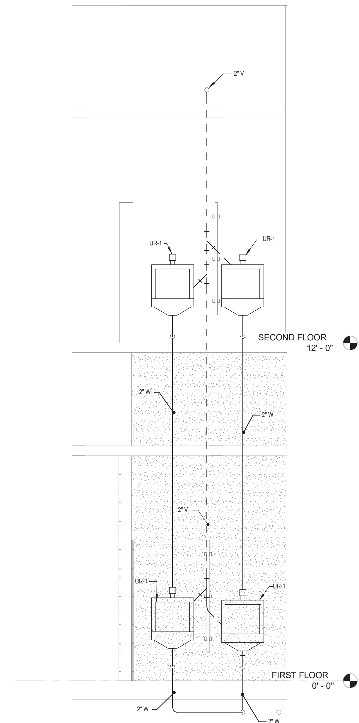
3 SANITARY AND VENT SECTION AT BOYS BATHROOM URINALS 1/2" = 1'-0"
